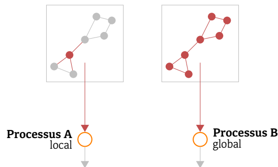
FIGURE 3.18 : Processus local/global.
