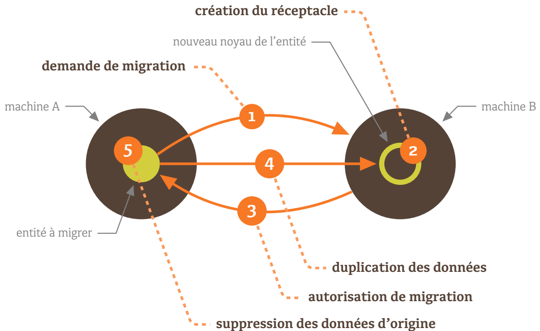
FIGURE 11.3 : Protocole de migration
