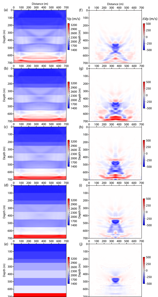
Figure 4: Reference and time-lapse V_p models: left panel shows the evolution of reference models from (a) reconstructed baseline image to (e) the true baseline model, and right panel illustrates each time-lapse image corresponding to the reference model at the left part.
