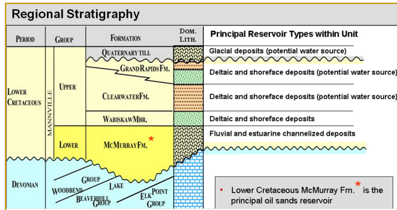
Figure 4.1: Geological overview of the field. Lower Cretaceous McMurray Fm is the principal oil sands reservoir.
