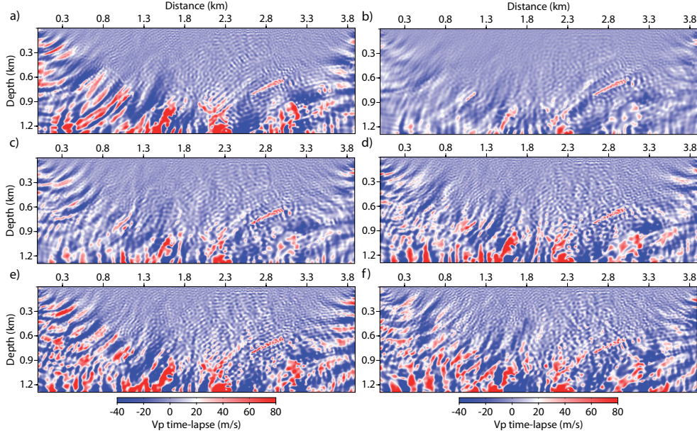
Figure 3.10: Time-lapse variation models obtained by the sequential difference strategy applied to noise-free dataset, starting from the recovered baseline model B1 ( df = 1 Hz) and frequency decimation on monitor dataset: (a) df = 0.2 Hz, (b) df = 1 Hz, (c) df = 2 Hz, (d) df = 3 Hz, (e) df = 4 Hz, (f) df = 5 Hz.
