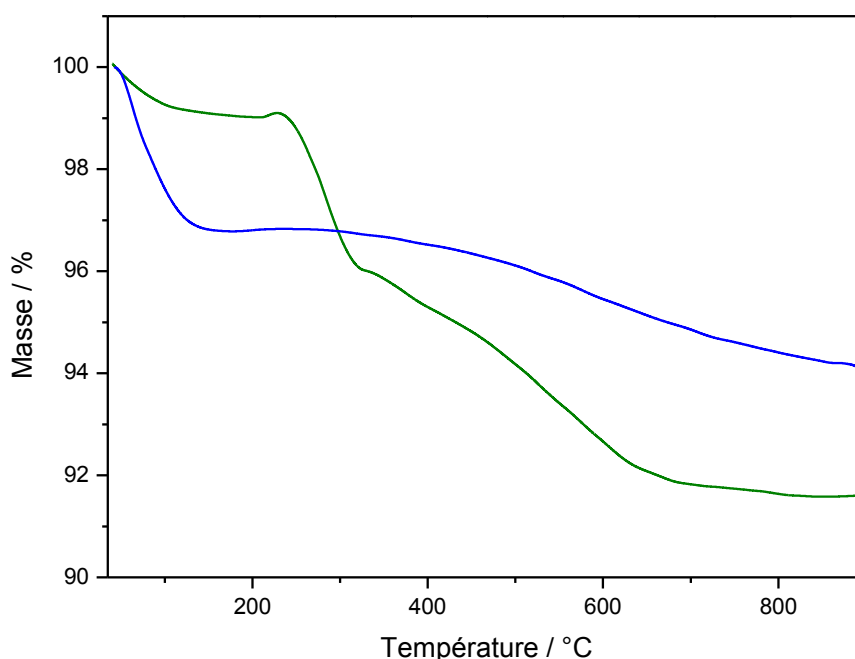
Figure IV-15 : Thermogramme des silices SiO 2 (c) (bleu) et SiO 2 (c)F (vert)
