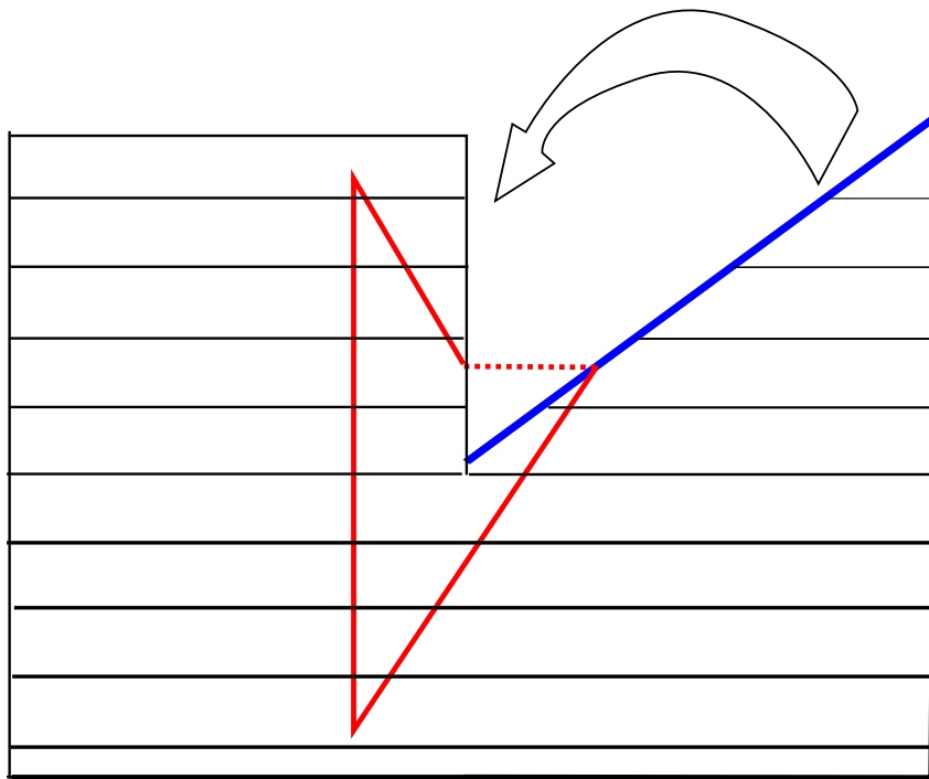
Figure 5.1: An example of convex geometry
