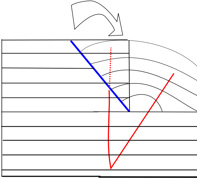
Figure 5.2: An example of non-convex geometry
