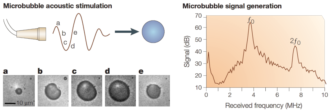
Figure A.5: (Left) Volumetric oscillation of a microbubble during exposure to ultrasound. The microbubble images were acquired under a light microscope each 330ns. (Right) Frequency versus amplitude data from microbubbles demonstrating returning signal both at the fundamental f_0 and second harmonic 2f_0 frequencies. (Source: [Lindner, 2004]).
