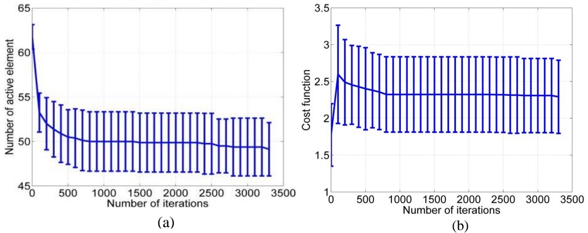
Figure 4.14: the evolution of (a) the active element number and (b) the cost function value as function of the iterations for an 8x8 2D array from the center of the 24x8 array. An iteration number of 1000 is sufficient for this small array.
