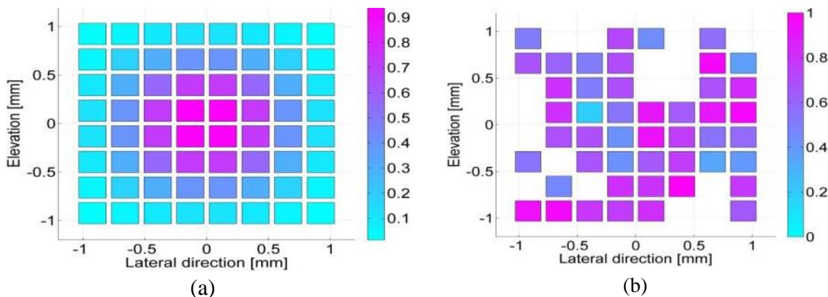
Figure 4.15: (a) the 8x8 dense array and (b) its corresponding optimized sparse array with 47 active elements. The colorbar indicates the apodization coefficients of the elements.
