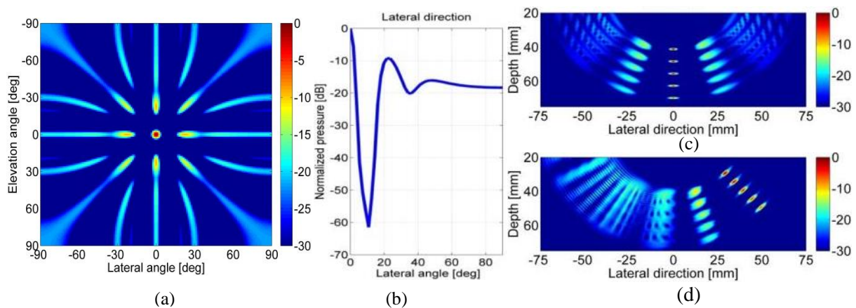
Figure 4.2 : beam pattern of the 8x8 array probe (a) c-scan plane at 50 mm, (b) and beam profile and (c) - (d) PSF in unsteering and steering cases, respectively. The ratio between the main lobe and the grating lobes is less than 10 dB (b). The PSF shows the effect of the grating lobes which can deteriorate the probe practical imaging features.
