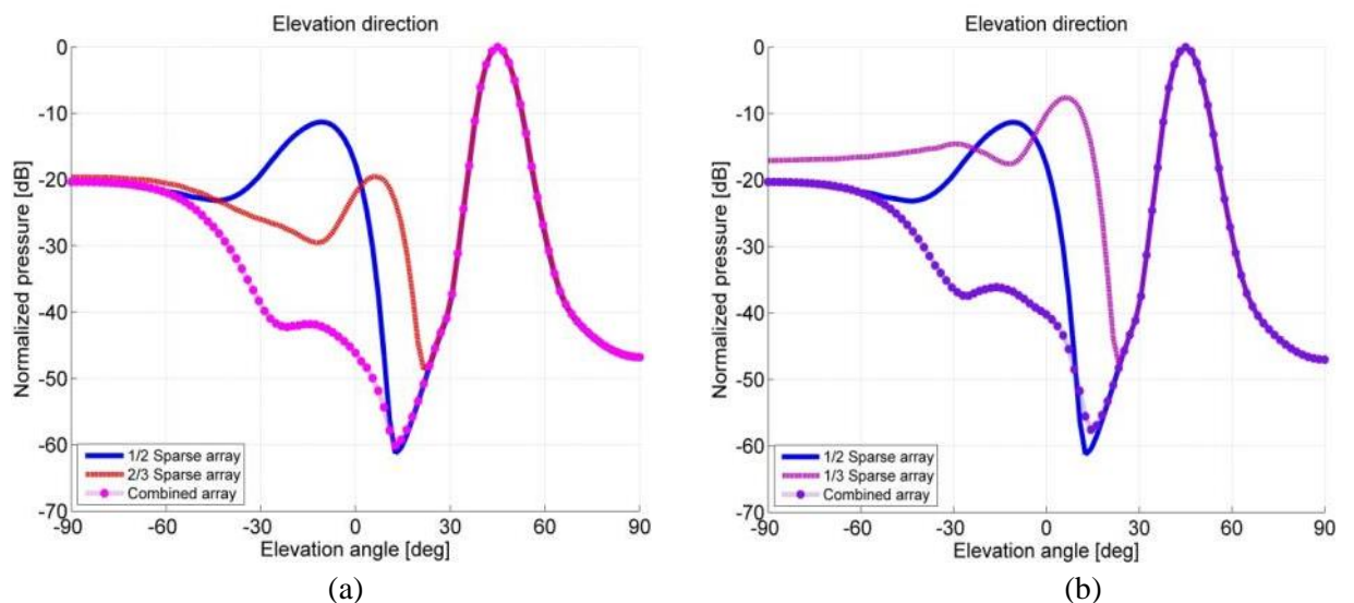
Figure 2.18: the concept the effective aperture when steering at (45^\circ, 45^\circ) . In (a) beam profiles of the regular sparse array (deriving from the 64x16 2D array) filled with 1/2 element (continuous line), 2/3 elements (dashed line) and the result when transmitting with one configuration and receiving by the other (dotted line), (b) the same results when the 2/3 element sparse array is replaced by a 1/3 (109 elements) sparse array.
