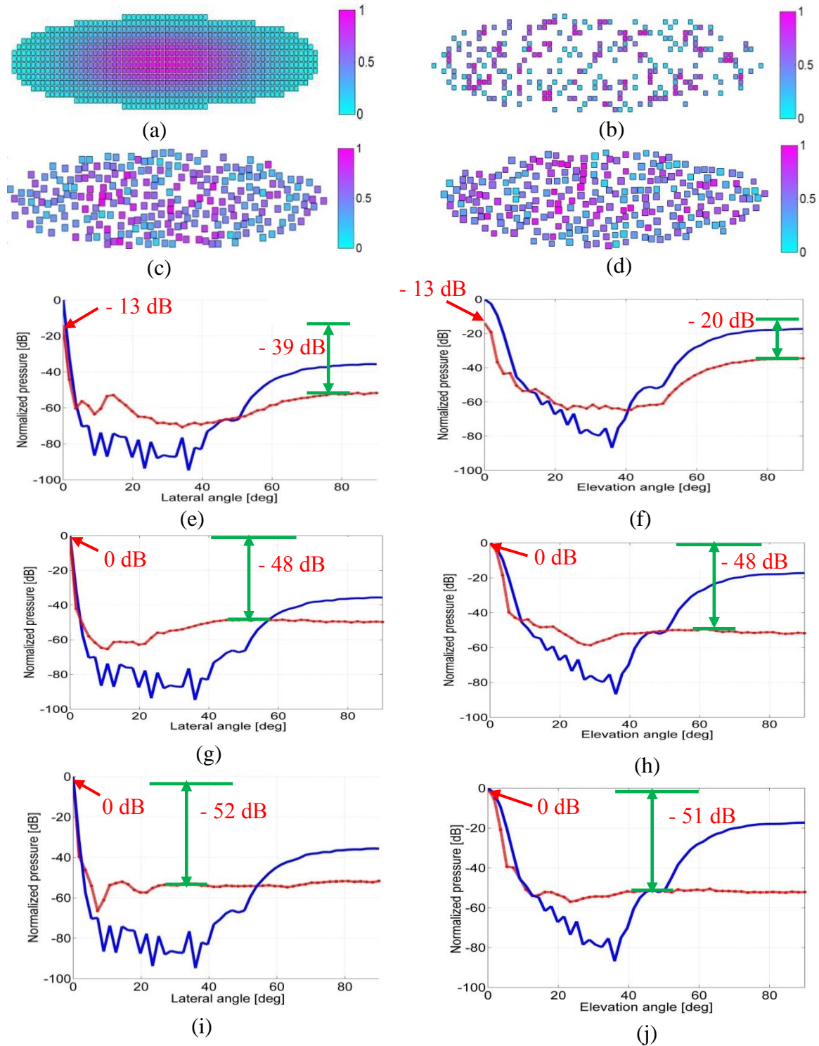
Figure 3.26: (a) the ellipsoidal part of the 64 \times 16 2D array of 828 elements, the optimized (b) standard sparse array with 256 elements of 0.5\lambda , (b) non-grid array with 256 elements of 0.7\lambda and (c) variable size arrays with 256 elements between 0.6\lambda and 0.8\lambda . The beam profile of each array is compared to that of the dense array to evaluate the energy loss and the grating lobes due to the element number reduction. The comparison to the dense array in both lateral and elevation direction is (e)-(f) for the sparse array, (g)-(h) for the non-grid array and (i)-(j) for the variable size array. In the standard sparse array, the energy loss is about 13 dB compared to the dense array whereas it is 0 dB in the non-grid arrays. The grating lobes are -39 dB and -20 dB in standard sparse array, -48 dB in non-grid array and at least -51 dB in variable size array against -36 dB and -17 dB in dense array in lateral and elevation directions respectively.
