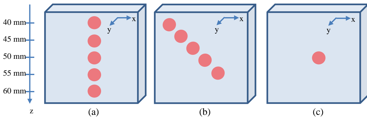
Figure 2.11: (a) and (b) represent the five-scatterer phantoms used in the PSF simulations (a) no-steering, (b) steering at ( 45^\circ , 45^\circ ) in both lateral (along x) and elevation (along y) directions and (c) represents the single scatterer phantom used to perform the beam profiles comparison. All the phantoms have the same dimensions.
