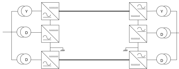
Figure 1.7: +U_1, -U_2 HVDC link
