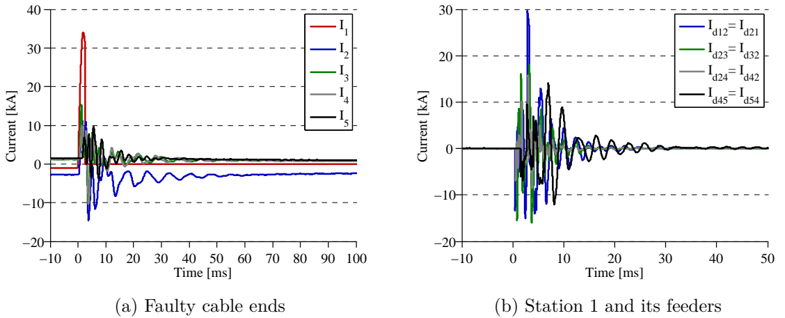
Figure 6.17: Current measurements for the fault clearing process
