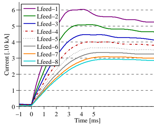
Figure 4.18: Current I_{21}
