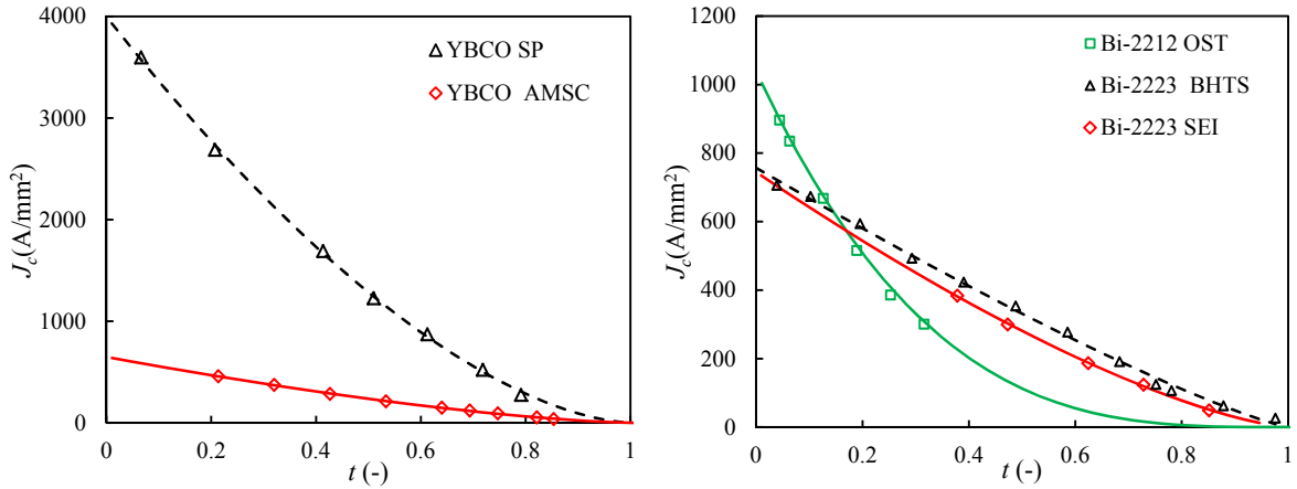
Figure A.3: The J_{c,s,f}(T) of YBCO SP and YBCO AMSC conductors (left). The J_{c,s,f}(T) of BSCCO SEI, BSCCO BHTS and BSCCO OST conductors (right).
