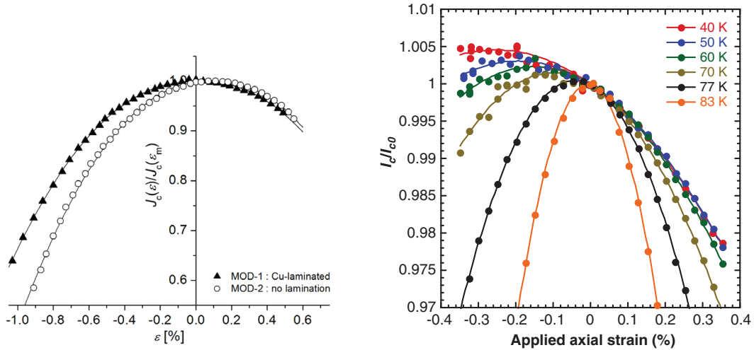
Figure 3.37: Dependence of the superconducting current density on applied axial strain in a copper laminated MOD-RABiTS sample at 76 K [167] (left). The temperature I_c strain dependency of an IBAD YBCO sample between 40 K and 83 K [175] (right).
