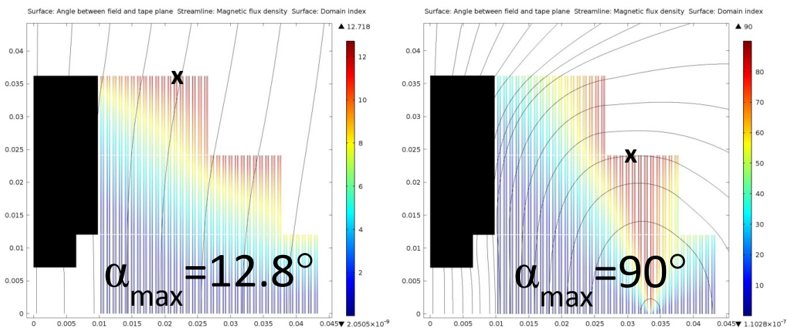
Figure 4.10: The deviation ( \alpha ) of the flux density with respect to the YBCO tape planes (bottom) at the bore flux density of 19 T (left) and 6 T (right) with the iron pole.
