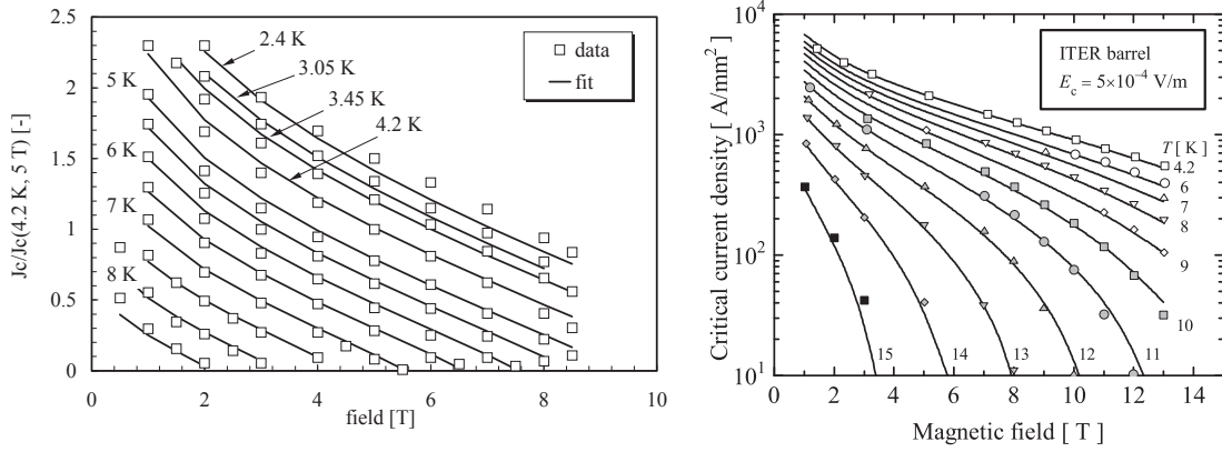
Figure A.2: Flux density dependence of the normalized J_c ( J_c(T, B)/J_c(4.2\text{ K}, 5\text{ T}) ) in Nb-Ti wires [28] (left). Flux density dependence of J_c in Nb 3 Sn wire (ITER barrel) at temperature ranging between 4.2 K and 15 K [98] (right).
