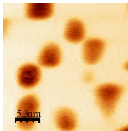
Fig. 2.19. AFM image in constant height mode.
