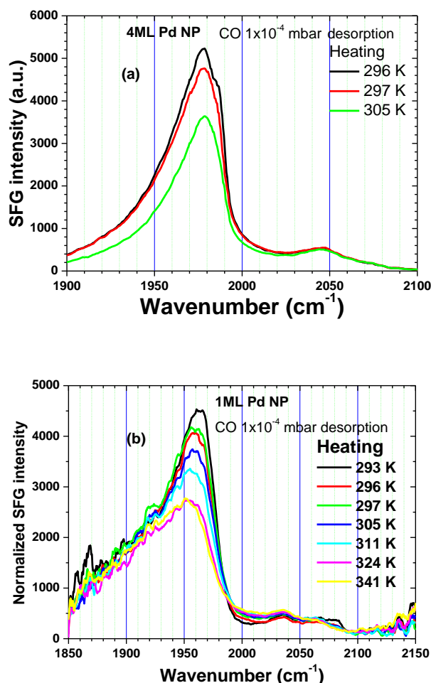
Fig. 5.15. SFG spectra of CO 10^{-4} mbar during heating on (a) 4ML and (b) 1 ML of Pd NP. (a) All spectra are normalized by the reference areas and (b) all spectra are normalized by the reference spectra.
