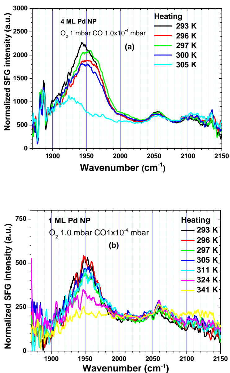
Fig. 5.14. SFG spectra of CO\ 1.0\times 10^{-4}\text{ mbar} + O_2\ 1.0\text{ mbar} adsorbed on (a) 4 ML; (b) 1 ML of Pd NP/ 3ML MgO/ Ag(100) samples upon heating. The spectra are normalized by the spectra of reference.
