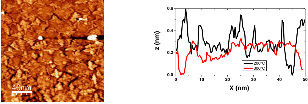
Fig. 2.17. 2 ML MgO film deposited on Ag(100) surface at 573 K. Left : STM image. Right : topographic profile along the grey line (red curve). The black curve shows a typical profile when MgO is grown at 473 K.
