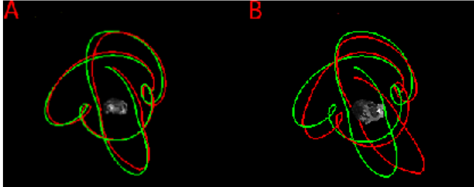
Figure 5.4: Simulated Itokawa asteroid sequence. A) A complex camera trajectory is shown to be more accurate when also matching the depth maps. The green curve represents the ground truth camera trajectory and the red curve is the estimated one. B. trajectory of purely intensity-based minimization for comparison.
