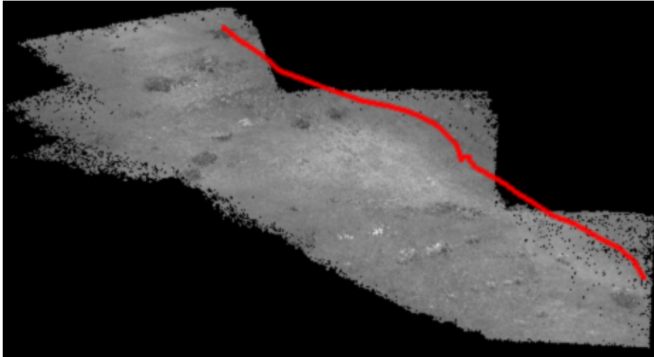
Figure 5.6: PProVisG MARS 3D Challenge sequence. The resulting camera trajectory and 3d reconstruction illustrated. The reconstruction shows the part of ground which is visible during the sequence.
