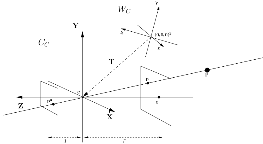
Figure 2.1: A perspective camera model
