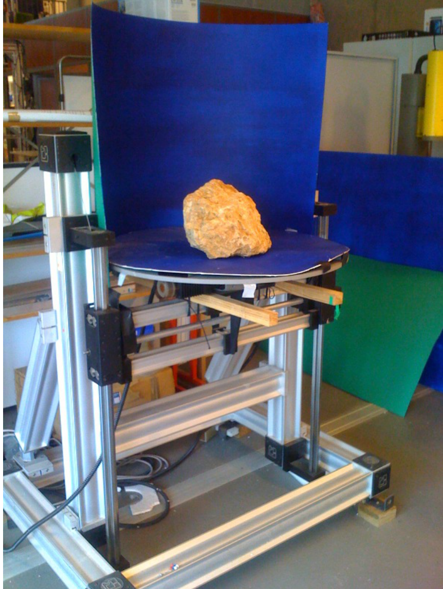
Figure A.2: The turn-table at INRIA was used for recording the rock sequence.
