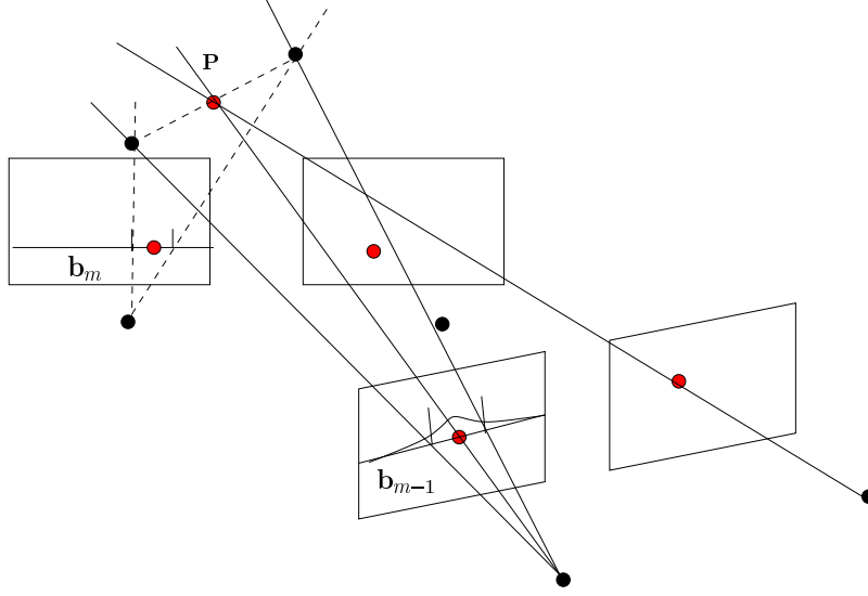
Figure 4.2: The transfer of a bounds into next stereo view. A bound is defined as [-p\sigma_k, p\sigma_k] interval using the disparity variance \sigma_k . The appropriate bound scale p is selected which includes also warping process noise.
