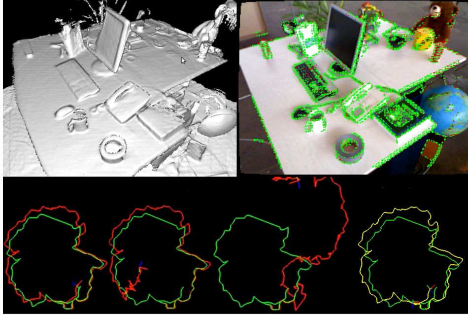
Figure 6.6: Kinfu performance compared with incremental dense tracking using freiburg_desk2 sequence with motion capture ground truth (green trajectory). Kinfu is executed with (3m)^3 , (5m)^3 and (8m)^3 voxel volumes. The red trajectories on the left are output from from Kinfu. Based on the trajectories, Kinfu gains lower drift due to structure integration, but planar surfaces cause tracking failures. (3m)^3 volume does not contain the floor and therefore Kinfu works well. On the right, the yellow trajectory is the proposed incremental RGB-D tracking result. Problems with planar surfaces do not exist, and the method allows larger operating volumes due to lower memory consumption. By using keyframes, the drift can be completely eliminated. The green dots reveal the selected points.
