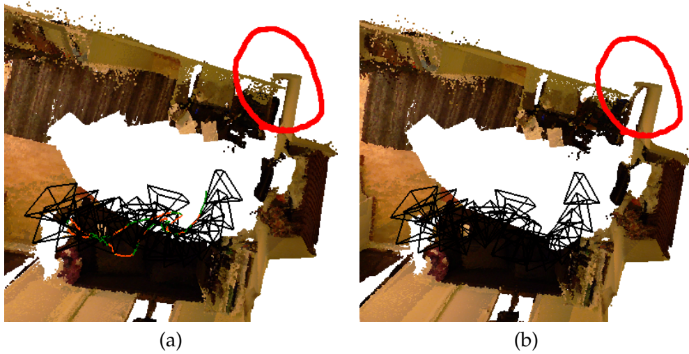
Figure 7.11: Room B sequence. Reconstruction bias in when operating in a) incremental mode, b) SLAM mode. After 360^\circ turn the first and last keyframe should map points consistently into a single 90^\circ corner. In this case a) is slightly more precise, because subsequent images are photometrically the most comparable with negligible interpolation errors.
