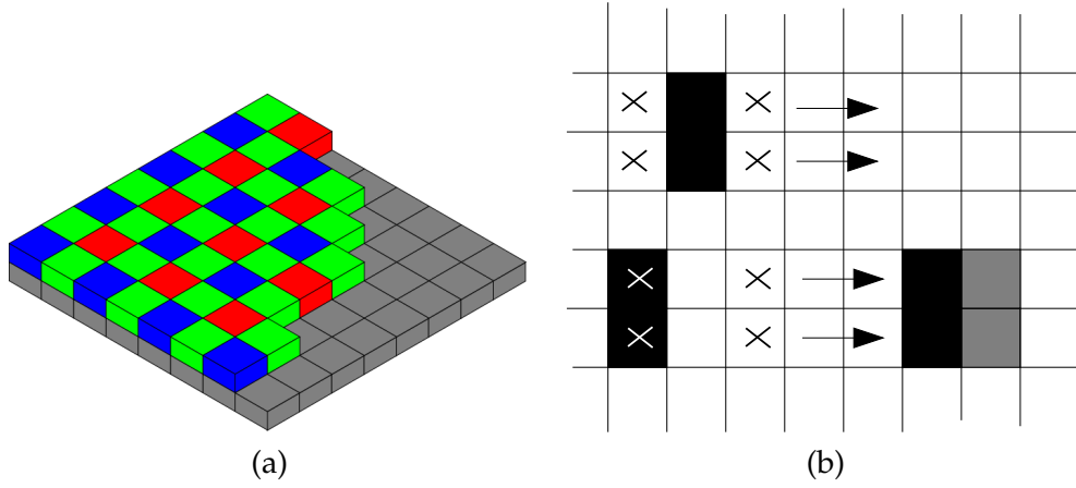
Figure 3.10: a) Bayer pattern in Kinect sensor. b) Examples how interpolation can remove edges and spread them.
