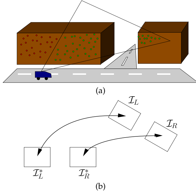
Figure 3.11: a) In contrary to Silveira, Comport et al. use dense matched 3D points to direct visual odometry. b) Left and right stereo images are matched from the available 4 combinations.
