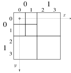
Figure 3.8: The multi-resolution pyramid layers are displaced when a rapid 2 \times 2 box filtering is used as anti-aliasing filter.
