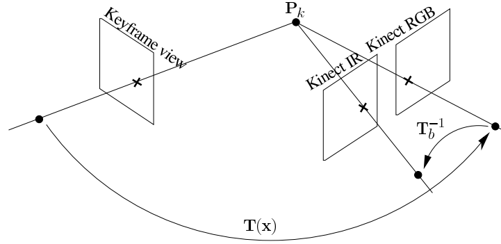
Figure 6.3: The warping of points from keyframe into Microsoft Kinect RGB and IR image coordinate systems. The additional depth lookup from an IR image is required by Equations 5.3 and 6.4.
