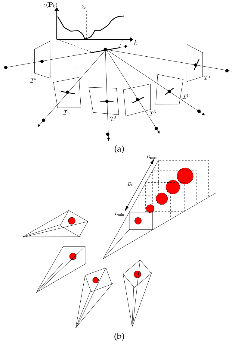
Figure 3.13: a) Photometrical refinement using bounded depth range. The optimal depth has the most similar color in all images. The pose configuration is assumed to be precise. b) Traditional plane sweeping algorithm illustrated. A depth value at reference image pixel is determined by the best color consistency in multiple views.
