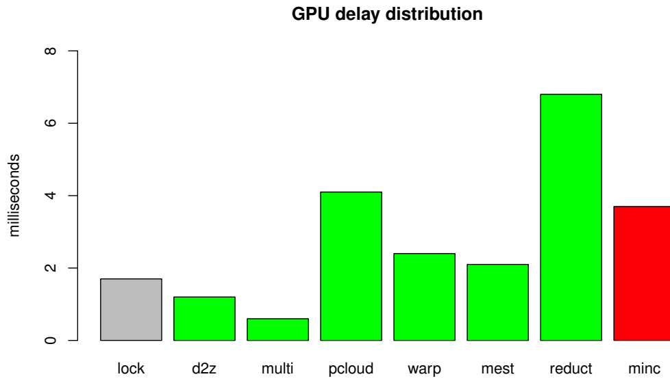
Figure 6.7: GPU tracking time distribution (23ms) for one frame. Green bars represent phases scalable to n threads. The red bar is executed by a single thread. The gray bar ( lock ) contains CUDA interop delays which are only required for visualization. d2z is disparity to depth conversion, multi is multi-resolution pyramid generation, pcloud is the 3D reconstruction, warp contains the cost function evaluations, mest is the M-estimation, reduct is linear system reduction, and minc motion estimation and update.
