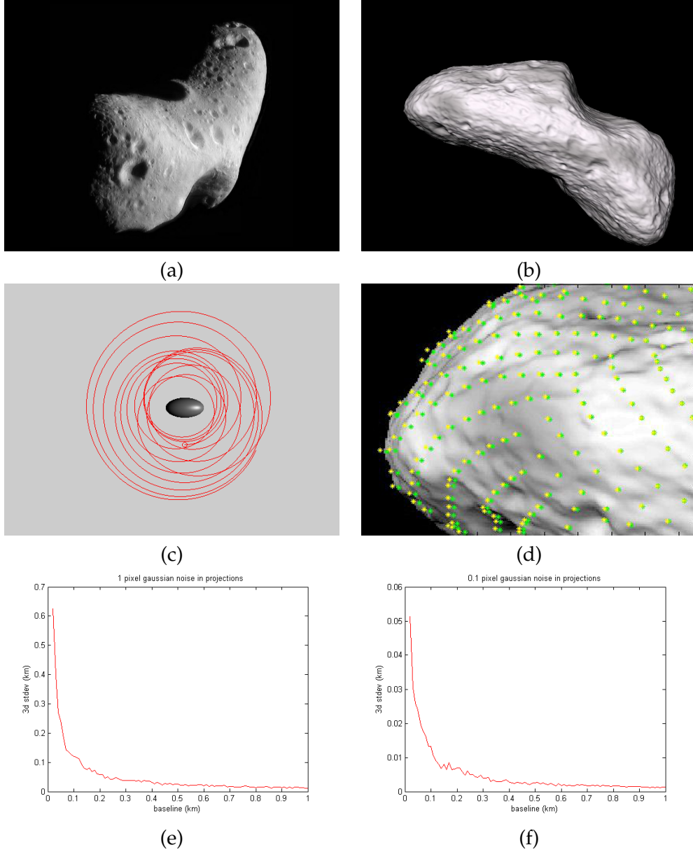
Figure A.1: Blender generated dataset for asteroid reconstruction mission. a) Real Eros Asteroid. b) A rendered Eros using Blender, c) A real satellite trajectory around the Itokawa asteroid provided by Thales-Alenia Space, d) Convergence was verified by matching a precise target projection with an estimated projection points. The precise projections on green and photometrically estimated ones on yellow before convergence. e) Hartley-Sturm reconstruction error in kilometers as a function of stereo baseline in an asteroid orbiting mission. Assuming 1px Gaussian stdev in disparity values. Over 1km baseline is required to reduce reconstruction error into tens of meters. f) Assuming 0.1px Gaussian stdev in disparity values. 200meters is a sufficient baseline, which produces 10m standard deviation for 3D points. Calibration is exact without any noise.
