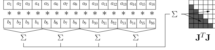
Figure 6.4: Efficient reduction on GPU. Dot products are divided into sub-ranges which are reduced in parallel. J^T J is symmetric 6 \times 6 matrix and elements can be mirrored with respect to the diagonal. The Jacobian columns are transposed into rows to improve memory caching.
