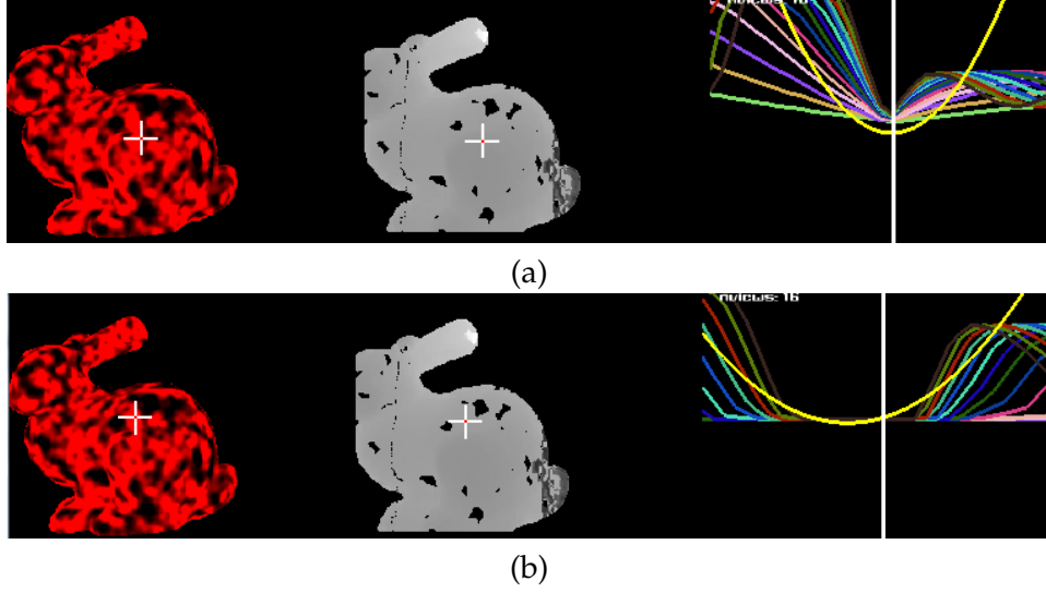
Figure 3.12: a) Textured Stanford bunny edges are associated with cost curves from 16 views. The vertical white line represents the correct depth value within the bounds. Yellow parabola's minimum represents the final image based estimate. b) Without edge information, image based estimation is not precise.
