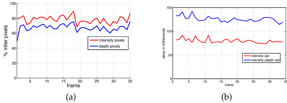
Figure 5.8: PProVisG MARS 3D Challenge sequence [29]. a) M-estimator functionality illustrated for the rover sequence. Total amount of selected pixels (inliers+outliers) is set to 50% which produces 38400 points in 320 \times 240 resolution. b) Optimization delay per frame in milliseconds with (blue) and without (red) depth component. Incorporating the depth component increases computational requirement by 50%. For a full real-time system disparity maps must be generated by external hardware/GPU.
