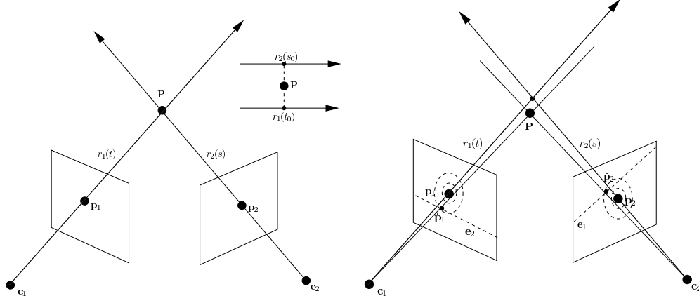
Figure 2.3: a) Midpoint triangulation, b) Hartley-Sturm triangulation.
