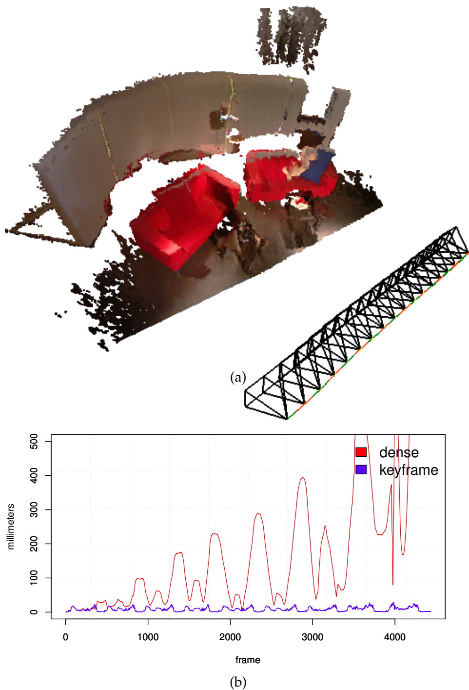
Figure 8.13: a) A rapid 3D scene reconstruction is made by moving a camera along a fixed 3.30m studio rail. b) A comparison between dense tracking and keyframe tracking. In dense tracking drift increases in time, but keyframe tracking maintains small bounded error. A person is moving in the scene during the last cycles.
