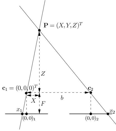
Figure 2.4: Rectified stereo triangulation. P , optical center c_k and the projection point x_k are on the same line based on perspective projection model. Relation between the disparity and depth value is determined by similar triangles. Right triangles are formed from point P at distances Z and Z + F , where F is the focal length.
