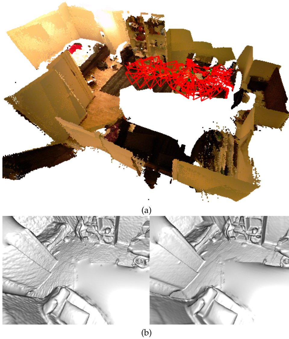
Figure 7.7: Room B sequence. a) A keyframe model obtained by executing keyframe SLAM in an apartment. b) Watertight Poisson reconstruction without and with depth fusion. Notice how holes are filled and missing regions such as the floor appears.
