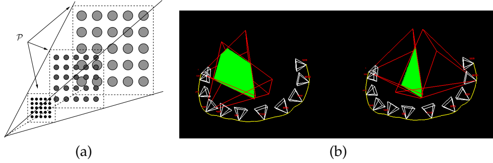
Figure 6.1: a) The 3D test point set \mathcal{P} used to compare camera poses is illustrated. \mathcal{P} approximates the view frustum by three 2D point grids. The projection error of \mathcal{P} between the current view and each keyframe view is compared to find the nearest keyframe. b) As comparison, frustum intersection volume based metric. The metric varies little when rotating around z-axis and can behave un-predictable way when the camera angles are significantly different.
