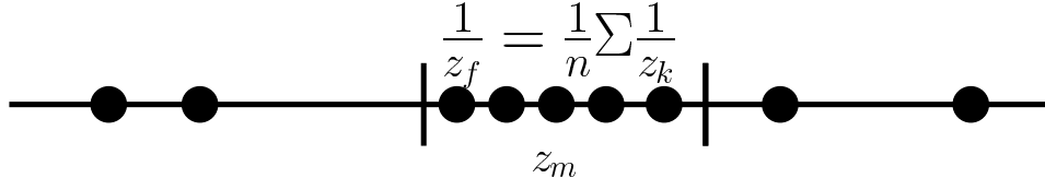
Figure 7.1: Robust depth estimation. A local average is computed within bounds near the median depth. Inverse depths are more likely to have Gaussian distribution in stereo camera settings. In case of small depth error, the bounds can be directly initialized near a depth map measurement.
