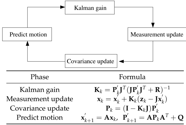
Figure 2.7: Kalman filtering process.
