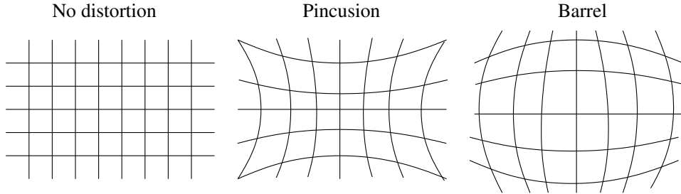
Figure 2.2: Pincushion and barrel distortion illustrated
