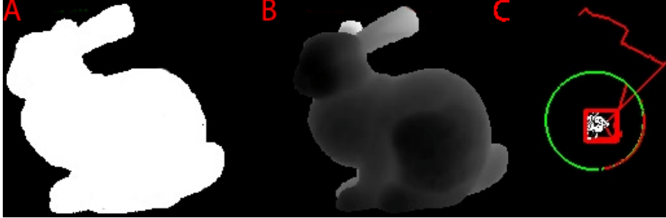
Figure 5.5: Orbiting sequence around Stanford bunny. A. image from the sequence, B. the corresponding depth map, C. the estimated camera trajectory (red) along with the ground truth (green). Insufficient texturing produces a singular \mathbf{H} which causes divergence during pose estimation. This problem is fixed by incorporating depth maps.
