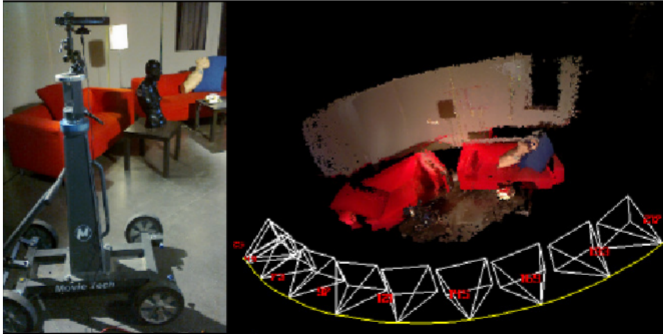
Figure 8.1: A RGB sensor is used to build a keyframe database which contains the views in the camera motion zone. The TV camera pose is estimated by registering the image content with the nearest keyframe.
