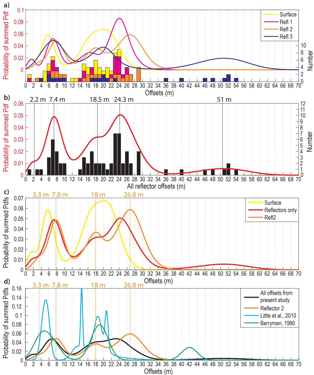
FIGURE 4.20 – Comparison of the four slip datasets. a) Histograms of the four sets of offset measurements compared to the four summed PDF curves. b) Histogram of the offset measurements derived from the GPR data (Refl1, Refl2, Refl3), compared to the corresponding summed PDF curve. Best-constrained offsets are indicated. c) Comparison of the summed PDF curves obtained for the Surface data (yellow), from the Reflector 2 data (orange), and for all GPR data (red). Best-constrained offsets derived for Refl2 are indicated. d) Comparison of the summed PDF curves obtained from the entire dataset of the present study (black), the Reflector 2 data (orange), the Little et al. [2010] data (blue) and the Berryman [1990] data (green).
