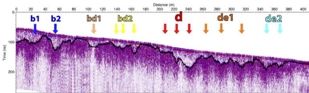
Cross Section P23
