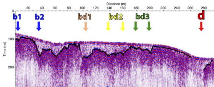
Cross Section P31
