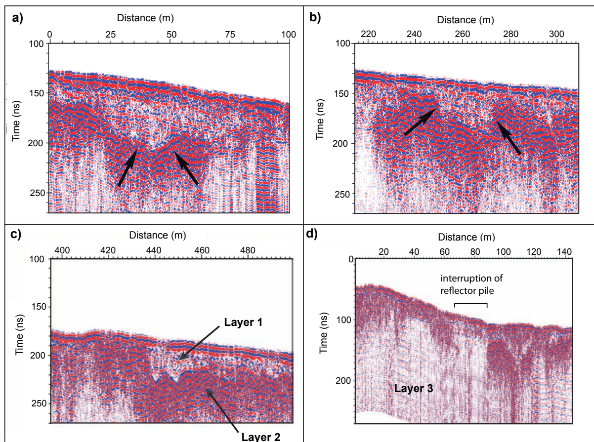
Figure 3.13: Close-up views of example GPR sections. The X-axis represents the distance from the western tip of the profile (a) The layer 2 pile of reflectors follows the trough edges so that the reflectors slightly dip toward the trough axis. (b) and (c) The layer 2 reflectors are interrupted at the trough edges. The trough is filled with layer 1 that clearly differs from layer 2. (d) The entire reflector pile is interrupted vertically, suggesting high electrical conductivity in the interruption zone.
