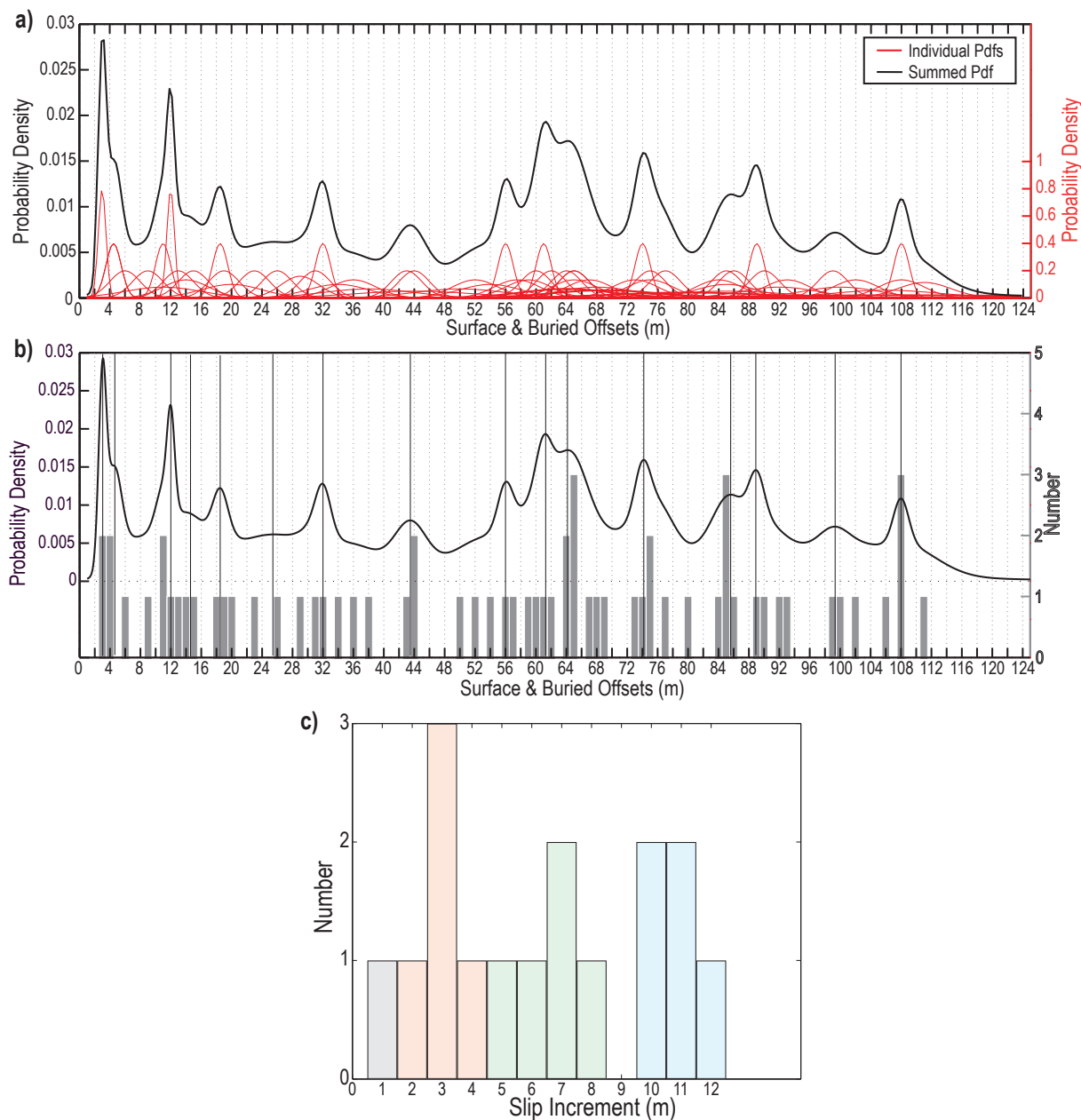
Figure 3.20: Probability density analysis of entire collection (surface and buried, 66 data) of offsets and slip increments. (a) Individual (red) and summed (black) PDFs of entire offset data collection, with two different scales. (b) Summed PDF curve compared with histogram of measured offset values. Best-constrained offset values are highlighted with vertical black lines. (c) Histogram of best-constrained slip increments for entire data collection. The three dominant sets of values are highlighted in pink, green and blue. See text for discussion.
