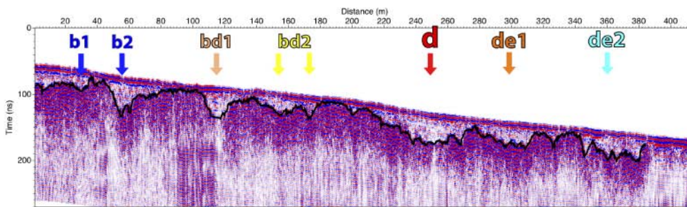
Cross Section P24
