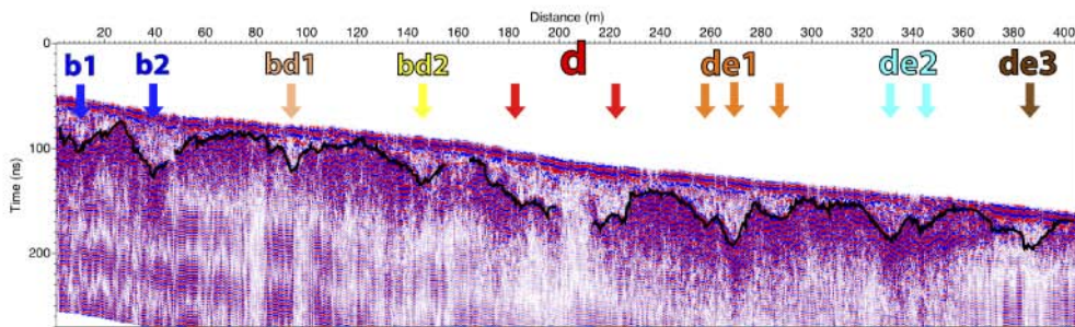
Cross Section P22
