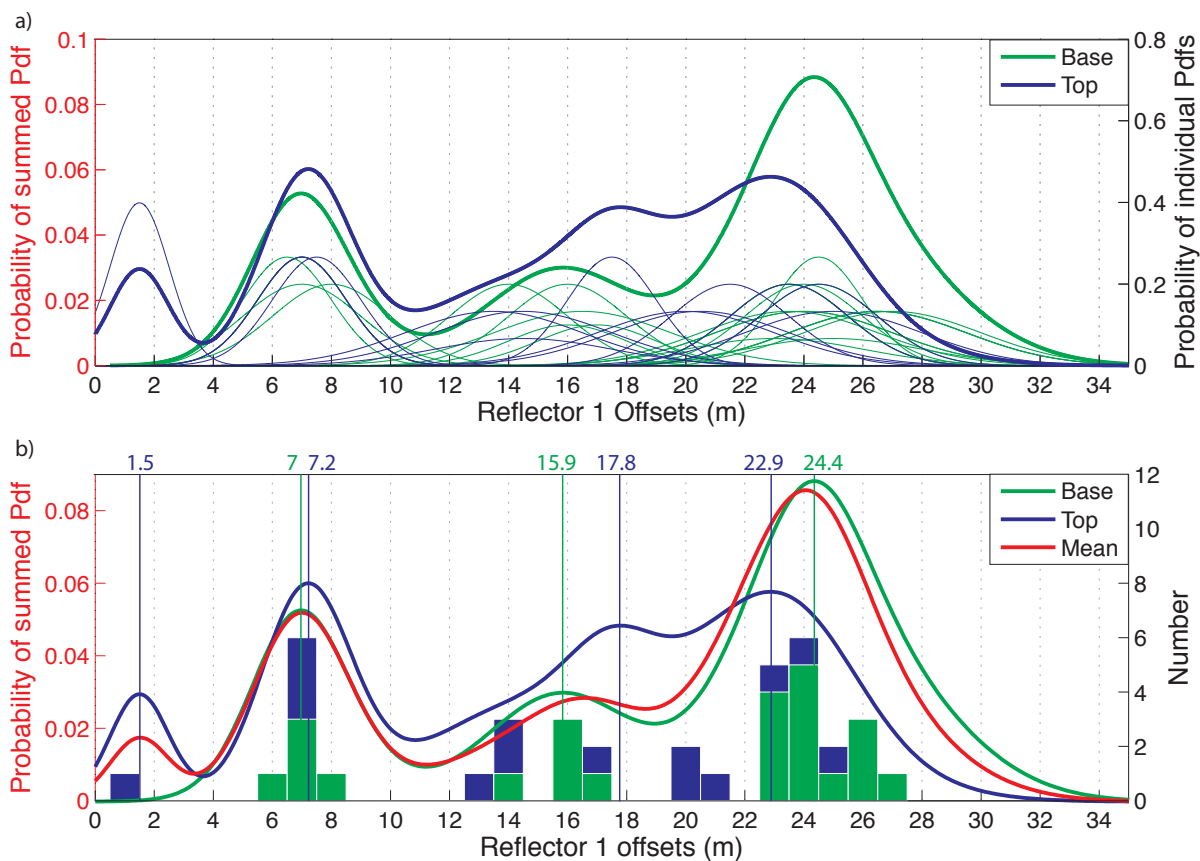
Supplement D- 8: Probability density analysis of the offsets measured in the Reflector 1 surface, discriminating the measurements for the bases and tops of the markers (from Table 4.1). (a) Individual Pdfs (thin lines, right axis) are compared to the summed PDF curves (thick lines, left axis), for both the bases and tops. (b) The histogram of the bases and tops offset values are compared to the corresponding summed PDF curves (green and blue), and to the summed PDF curve for the entire dataset (red). The best-constrained offsets are indicated. The figure has to be compared with Figure 4.14.
