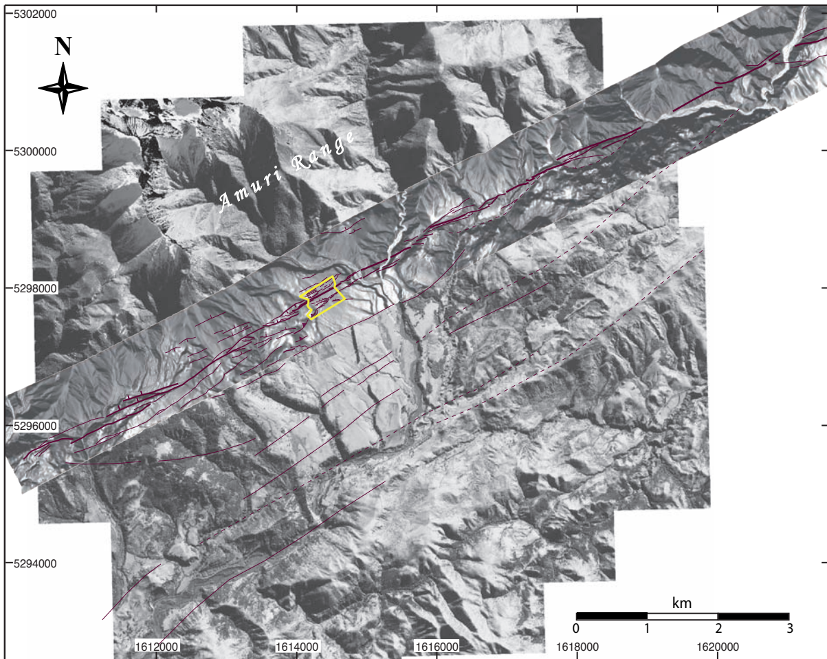
Figure 3.5: Detailed mapping of the Hope Fault trace, based on combined analysis of Ikonos satellite image and LiDAR data (white swatch; only half of swath length is shown). Fault traces in purple. Thicker lines for most pronounced, hence most important, fault traces. Lines without marks are for right-lateral strike slip faults, teeth marks indicate downthrown side of normal faults, triangle marks indicate upthrown side of reverse faults. Yellow rectangle indicates the GPR survey. See text for more details.
