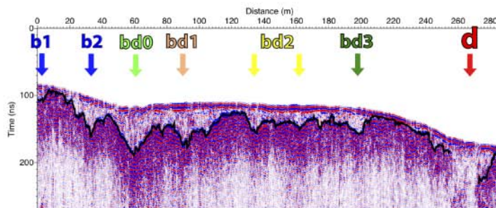
Cross Section P32
