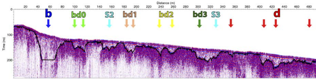
Cross Section P53
