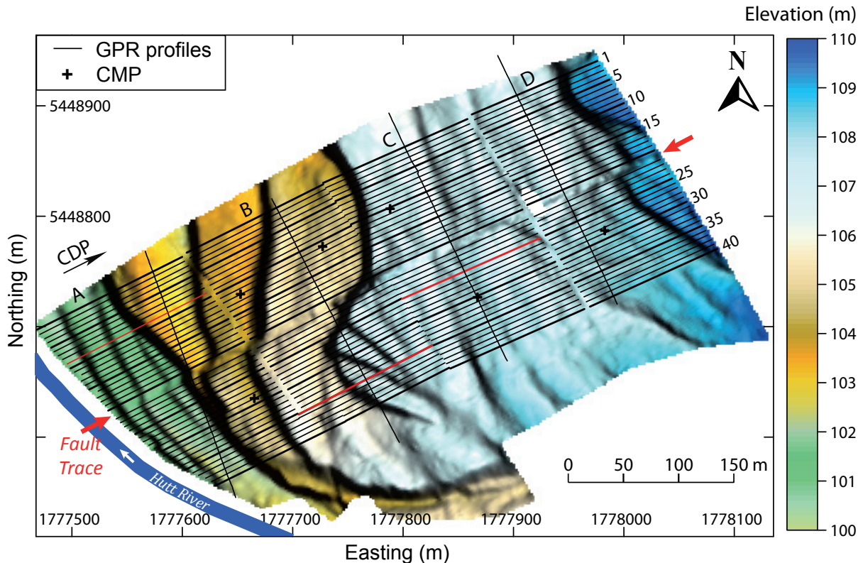
FIGURE 4.5 – Location of GPR profiles and CMPs on the GPS-derived DEM. Red arrows indicate the fault trace. Red lines are sections shown in Figure 4. The GPR fault-parallel profiles are numbered 1 to 40 from north to south, and each is divided into 4 subsections A, B, C, D (limited by fences). The Common Depth Point (CDP) increasing eastward is indicated. All GPR profiles are presented in Supplement D-1. Coordinates are in NZTM 2000 reference frame.
