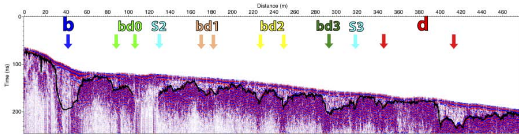
Cross Section P54
