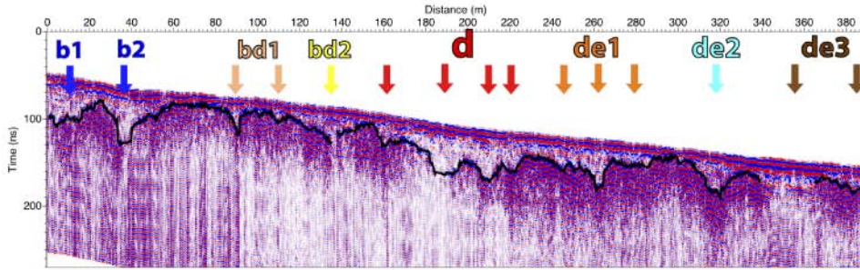
Cross Section P21
