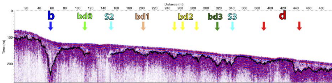
Cross Section P55
