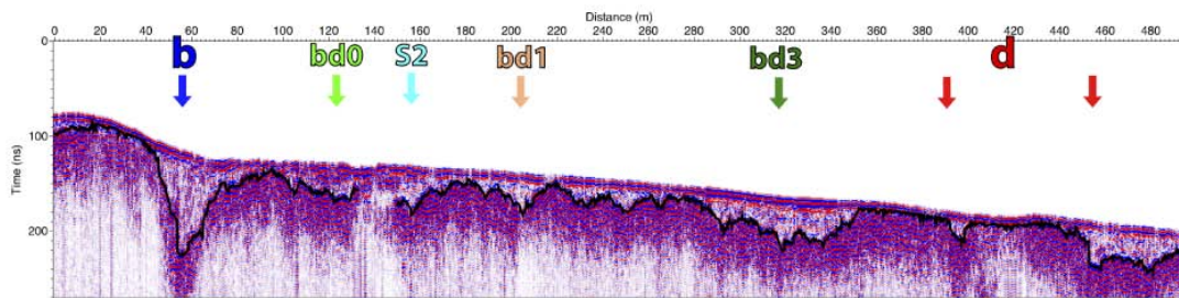
Cross Section P56
