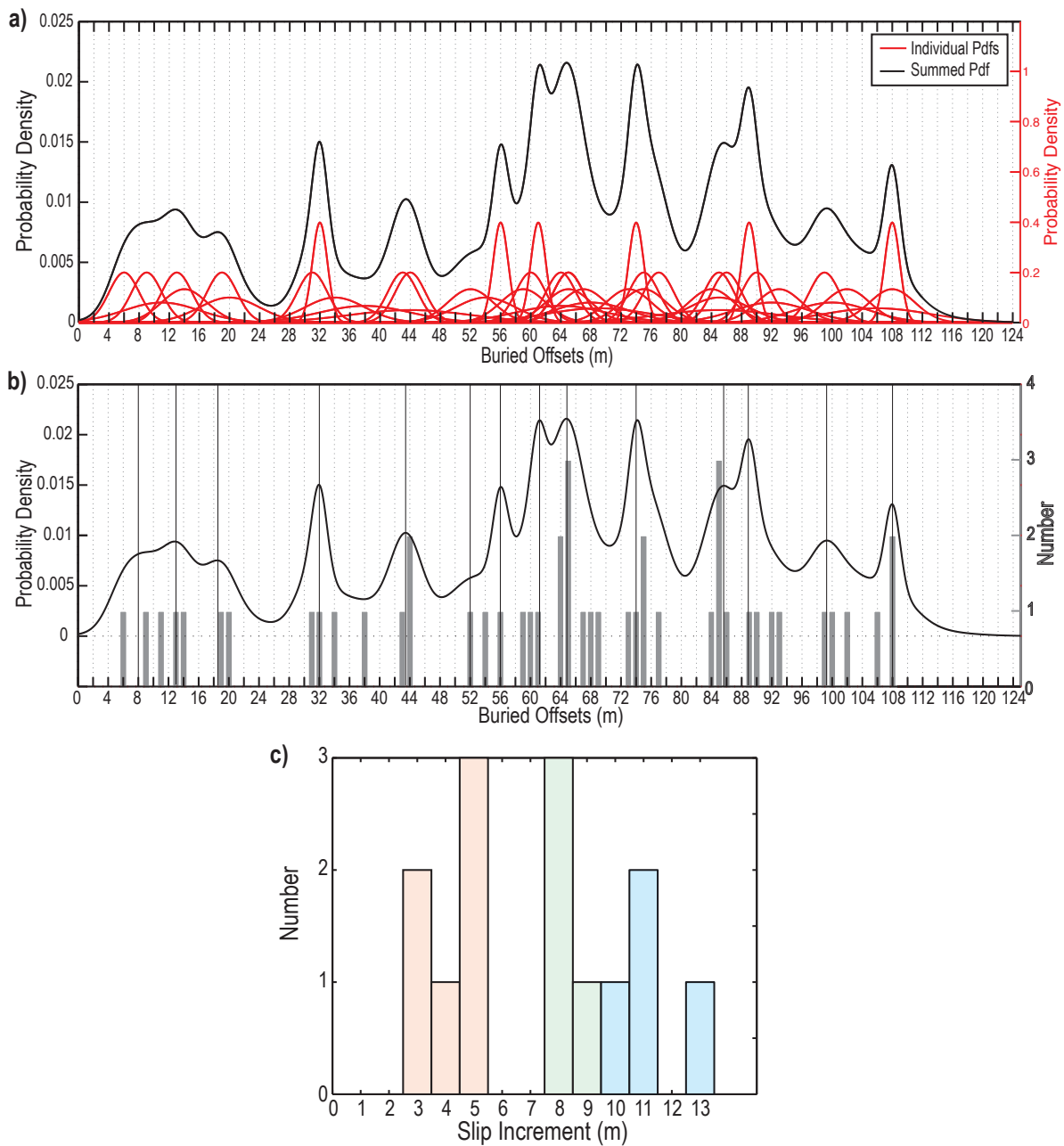
Figure 3.18: Probability density analysis of buried offsets and slip increments. See text for discussion on PDFs calculation. (a) Individual (red) and summed (black) PDFs of buried offset data, with two different scales. (b) Summed PDF curve compared with histogram of measured offset values. Best-constrained offset values are highlighted with vertical black lines. (c) Histogram of best-constrained slip increments. The three dominant sets of values are highlighted in pink, green and blue. See text for discussion.
