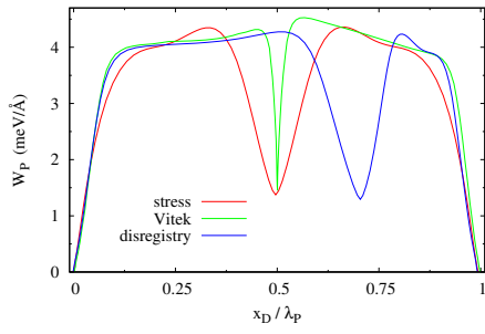
(c) 1479 atomes - \tau = 0 GPa
