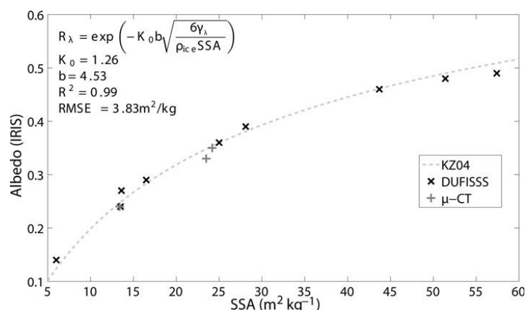
Fig. 6. Relationship between the IRIS-derived albedo and SSA measurements from the DUFISSS system (x) and \mu -CT measurements (+). Dashed line corresponds to the KZ04 albedo model (Eqn (2)).
