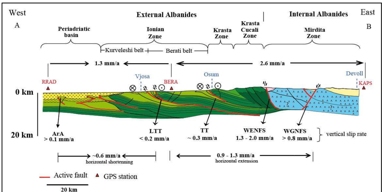
Figure IV.37. Simplified structural cross-section through the Southern Albanides adapted from, the Geological Map of Albania (SHGJSH, 2003), Kilijs et al. (2001), Roure et al. (2004) and Carcaillet et al. (2009). The neotectonic framework is modified from Aliaj et al. (1996, 2000) and the strike-slip component deduced from GPS network (Jouanne, et al., 2012). Values of relative displacements between GPS sites are indicated above GPS stations. Vertical slip rates calculated in the present study are shown, as well as, the horizontal shortening and extension estimated from the slip rate.
