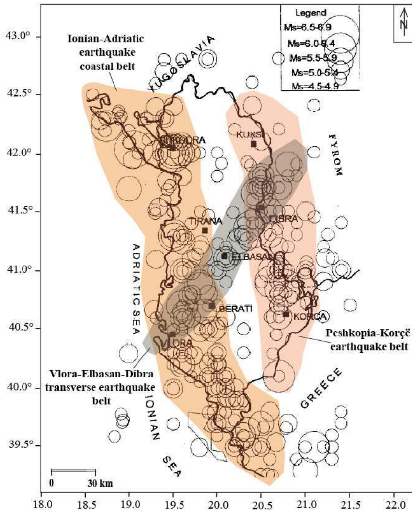
Figure IV.6. Epical map of earthquakes in Albania and neighboring areas for the period 1901–1995 with M_s \geq 4.5 , from Sulstarova et al. (2000). The three earthquake belts are clearly identified by polygon of different colors.
