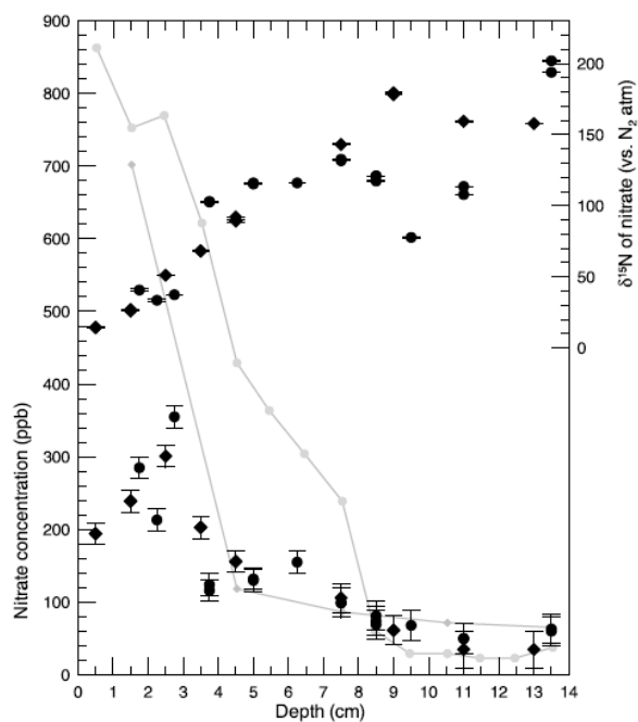
Figure 1.27. The nitrate concentration and \delta^{15}\text{N} profile with depth for two ice cores extracted from Dome C. Concentration measurements were estimated from mass spectrometer measurements and error bars show one sigma from analytical errors (Blunier et al., 2005). Previous concentration measurements by (Röthlisberger et al., 2000) are shown in grey dots and diamonds.
