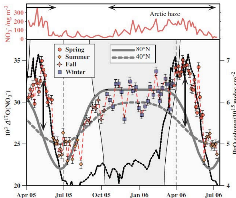
Figure 1.24. The concentration and \Delta^{17}\text{O}(\text{NO}_3^-) values from atmospheric nitrate collected at Alert, Canada (Morin et al. 2008). The black dashed line represents satellite retrieved BrO measurement data. Solid and dashed grey lines represent calculated \Delta^{17}\text{O}(\text{NO}_3^-) values at 80^\circ\text{N} and 40^\circ\text{N} latitudes respectively. The strong deviations from these calculations during spring caused by interaction between snowpack emitted \text{NO}_x and BrO are shown using the vertical thick black arrows.
