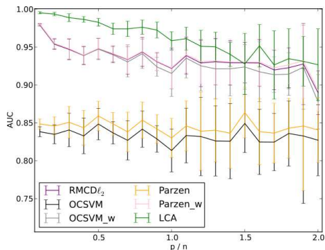
Figure 3.16: Outlier detection accuracy of non-parametric density estimation algorithms, represented by their AUC (real data) . LCA outperforms both Parzen density estimation and One-Class SVM, even applied on whitened data. RMCD parametric method has the same accuracy than the latter. LCA seems to be sensitive to the p/n ratio as its performance decreases with this ratio.
