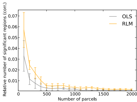
Figure 5.6: Percentage of parcels significantly associated with a non-null effect of the SNP \times Stressful Life Events (SLE) interaction , according to standard and robust regression. The latter always uncovers more significant associations.
