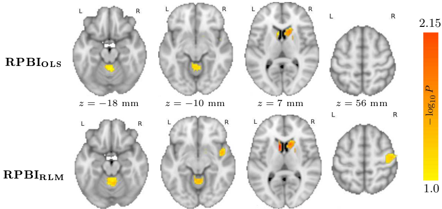
Figure 5.7: Voxel-level FWER-corrected p-values maps given by RPBI_{OLS} and RPBI_{RLM} on our gene-neuroimaging study (represented as negative \log_{10} p-values). Four brain regions are associated with a significant non-null effect according to the robust version of RPBI, while only two of them are reported by standard RPBI. The significant associations observed in the left and right ventral striatum (third column, z = 7 mm) are particularly relevant to the study, as the ventral striatum plays a key role in the processing of positive and negative reward signals, including anger expressions.
