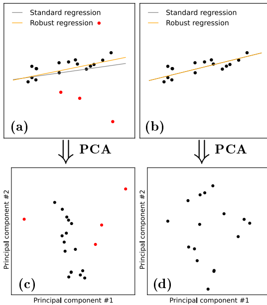
Figure 3.1: Influence of outliers in a regression task. (a) Contaminated dataset. (b) Uncontaminated dataset. Outliers yield huge residuals that standard regression tries to minimize so as to diminish the sum of squared residuals criterion. Robust regression can accommodate the presence of outliers and is almost equivalent to standard regression when no outlier is present in the dataset.
