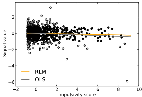
Figure 5.9: Relationship between the mean signal within a parcel centered at the hypothalamus and the impulsivity factor (1364 subjects) . Covariables effect has been removed from the two values. Regression lines have been drawn on top of the data for standard (OLS) and robust regression (RLM).
