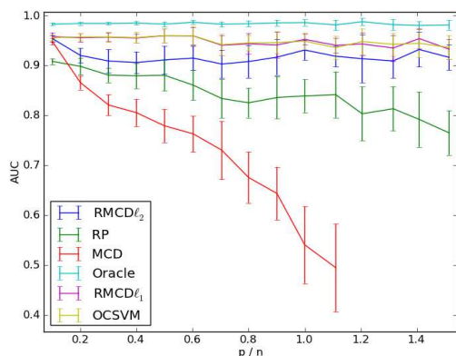
Figure 3.10: Synthetic data, variance outliers. AUC for various outlier detection methods in the case of variance outliers ( p = 100 , \kappa(\Sigma) = 100 , a = 1.15 , \gamma = 40\% ). \ell_1 - and \ell_2 -regularized versions of the MCD outperform by far the standard MCD, benefiting from the isotropic distribution of the outliers. RMCD-RP's accuracy slightly decrease with p/n , which makes it not suitable for our problem. OCSVM w also gives good performance.
