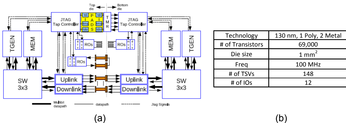
Figure 33: 3D NoC with fault tolerant (a) architecture (b) design summary
