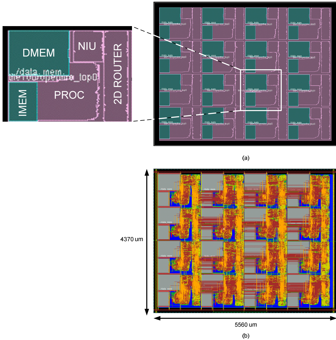
Figure 76: Baseline 2D MPSoC architecture (a) amoeba view (b) routed layout
