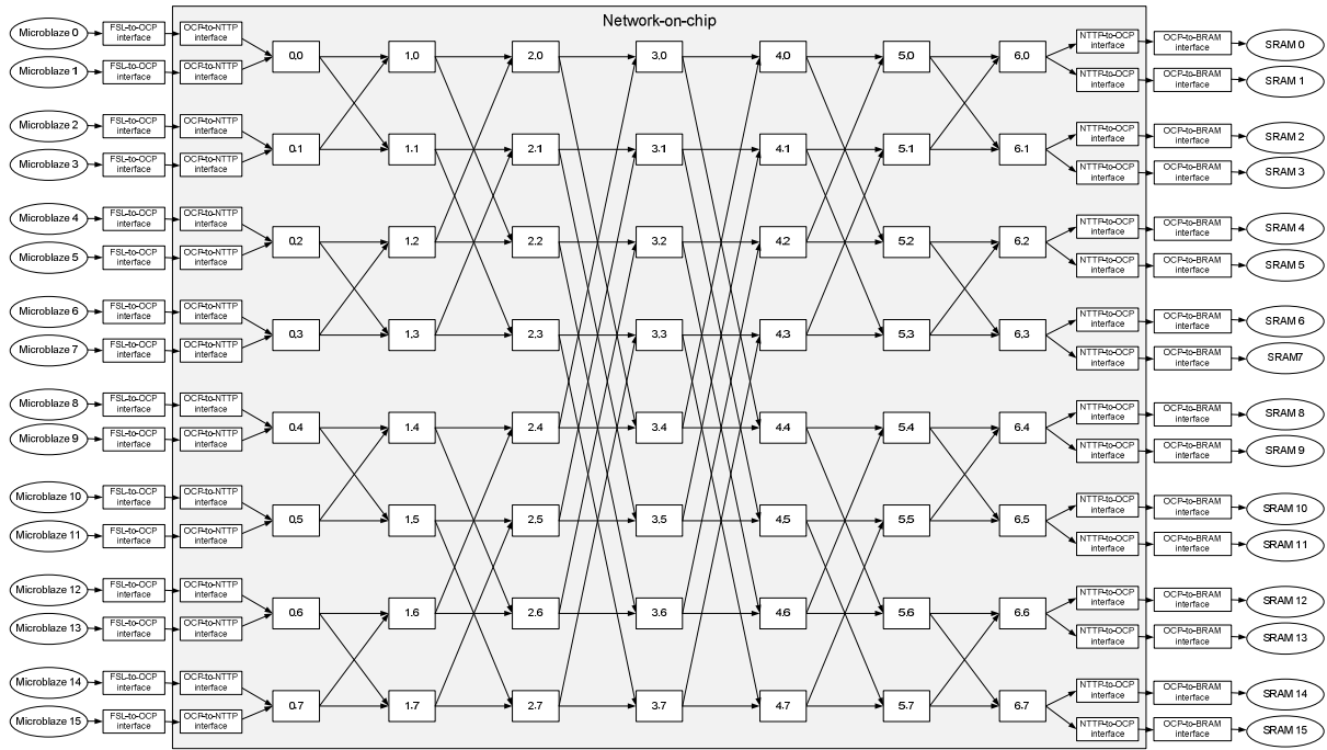
Figure 6: 2D NoC-based MPSoC architecture with masters and slaves connection
