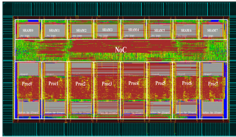
Figure 71: Routed layout of MPSoC2 architecture (bottom tier)
