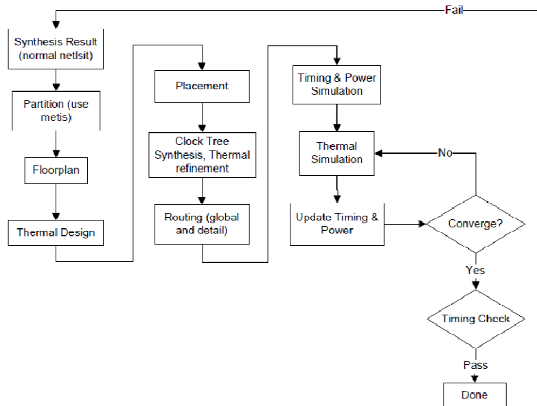
Figure 36: 3D design methodology for timing, power and temperature exploration [131]
