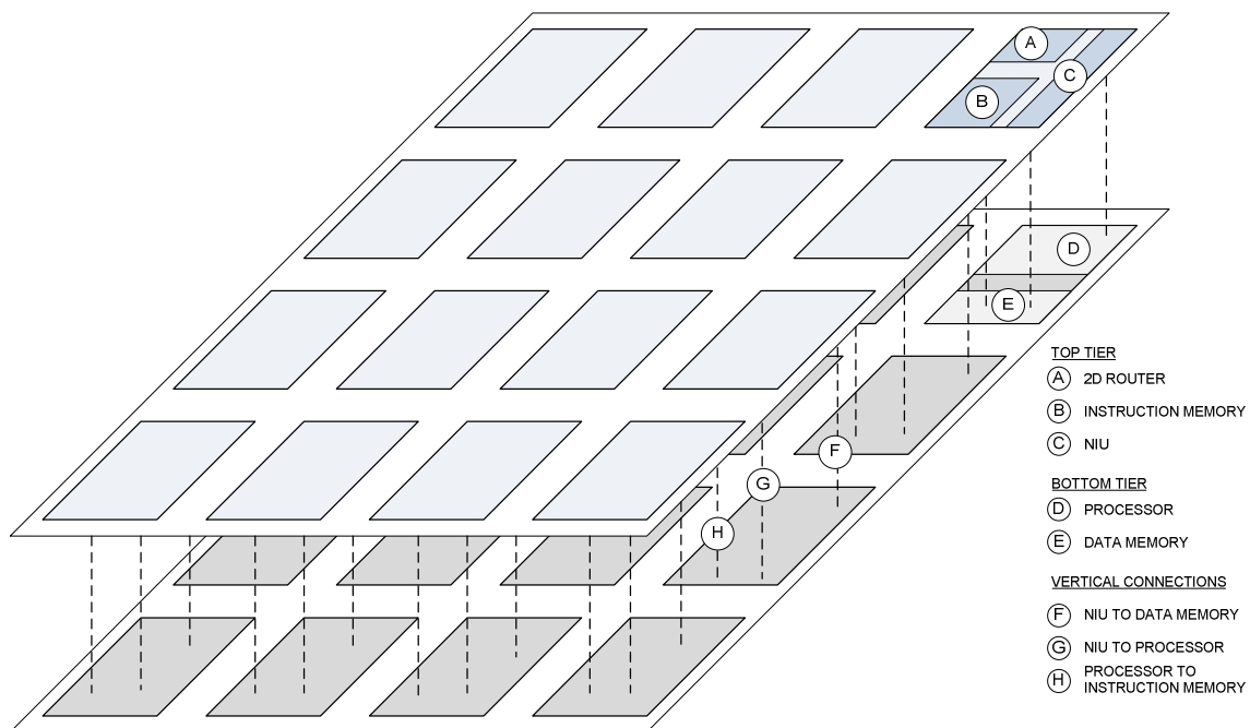
Figure 77: Heterogeneous 3D MPSoC stacking
