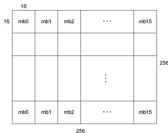
Figure 8: Processor allocation for data parallel of DCT application on 256 \times 256 pixels image
