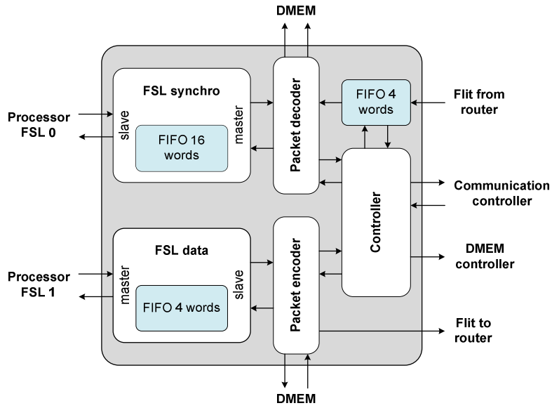
Figure 47: NIU architecture
