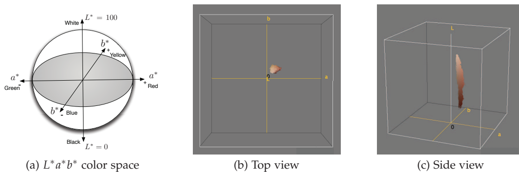
Figure 4.4: Skin color distribution in L^*a^*b^* color space.
