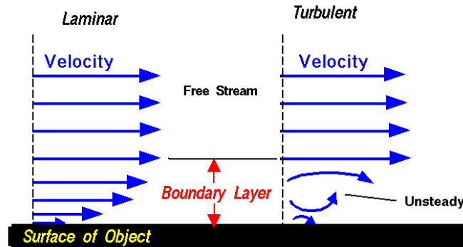
Figure 1.3: Boundary layer of plane channel flow (velocity is zero at the surface), figure from Glenn Research Center, NASA
