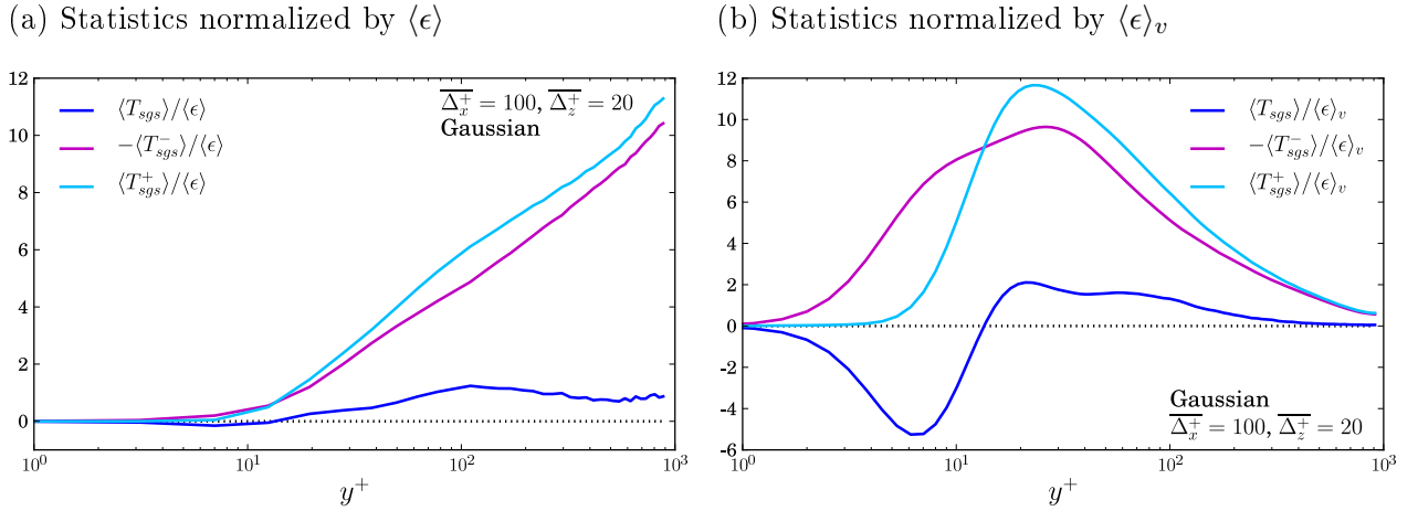
Figure 4.3: SGS energy transfer including the back scatter and forward scatter contributions, normalized by plane-averaged (a) and volume-averaged (b) rate of kinetic energy dissipation. Statistics are given for the same filter width \overline{\Delta_x^+} = 100 and \overline{\Delta_z^+} = 20 and a Gaussian filter.
