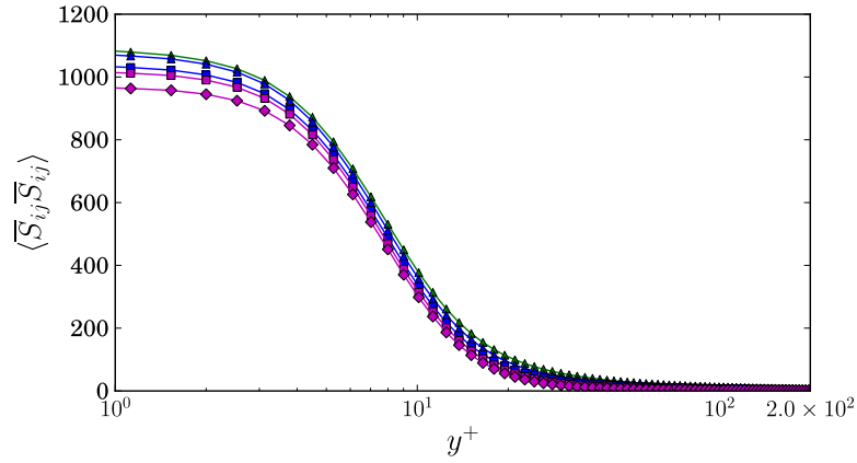
Figure 4.30: Near wall region behavior of the differential operator \langle \overline{S}_{ij} \overline{S}_{ij} \rangle using Lss-5 th filter.
