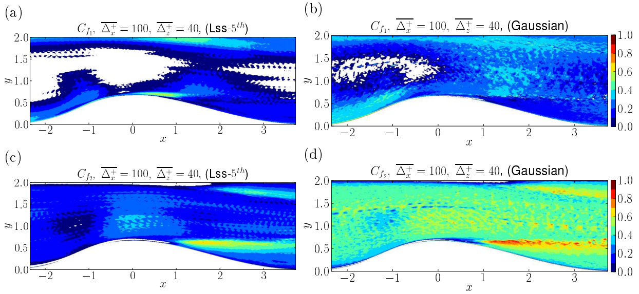
Figure 5.39: Correlations C_{f_1} and C_{f_2} between the exact SGS force and its counterpart modeled by the Smagorinsky model using Lss-5 th (a, c) and Gaussian (b, d) filters.
