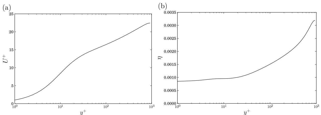
Figure 3.9: Mean streamwise velocity U^+ (a) and the Kolmogorov scale \eta (b) along wall normal position at the lower half of plane channel flow at Re_\tau = 950 .
