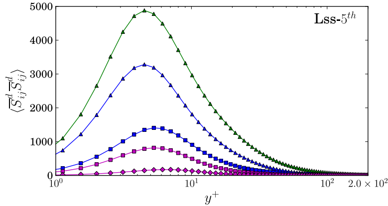
Figure 4.23: Near wall region behavior of the WALE model operator \langle \overline{S_{ij}^d S_{ij}^d} \rangle using Lss-5 th filter.
