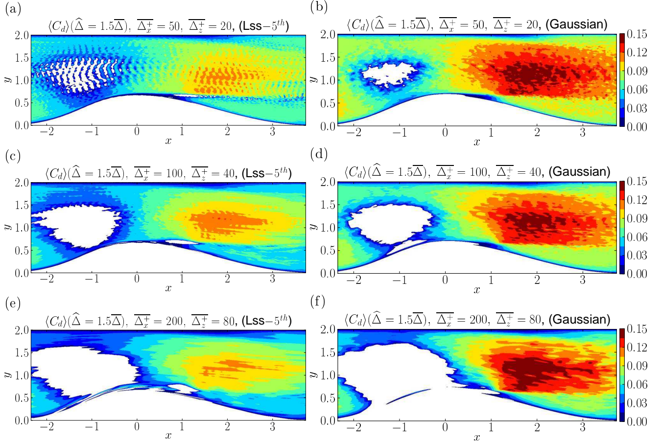
Figure B.7: A priori estimate of coefficient \langle C_d \rangle of Dynamic Smagorinsky model in the converging-diverging channel regions with three filter sets ( \widehat{\Delta} = 1.5\overline{\Delta} ) using Lss-5 th (a, c, e) and Gaussian (b, d, f) filters.
