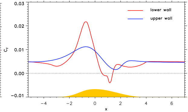
Figure 3.13: Skin friction coefficient C_f = \tau_w / (\frac{1}{2}\rho U_o^2) at the two walls.
