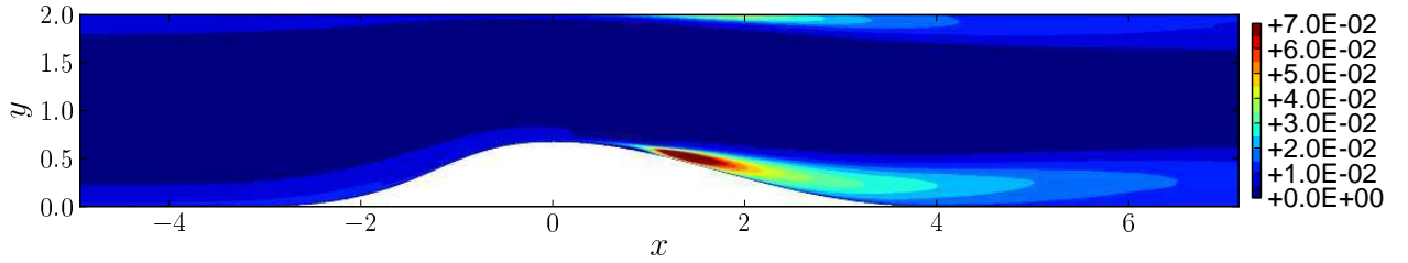
Figure 3.14: Averaged turbulent kinetic energy \langle q^2 \rangle = \langle \frac{1}{2} u'_i u'_i \rangle on channel flow with adverse pressure gradient at Re_\tau = 617 .
