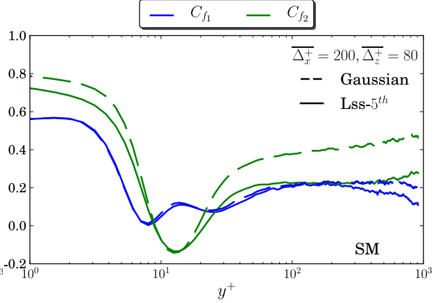
Figure 4.44: Influence of filter type on correlations C_{f_i} .
