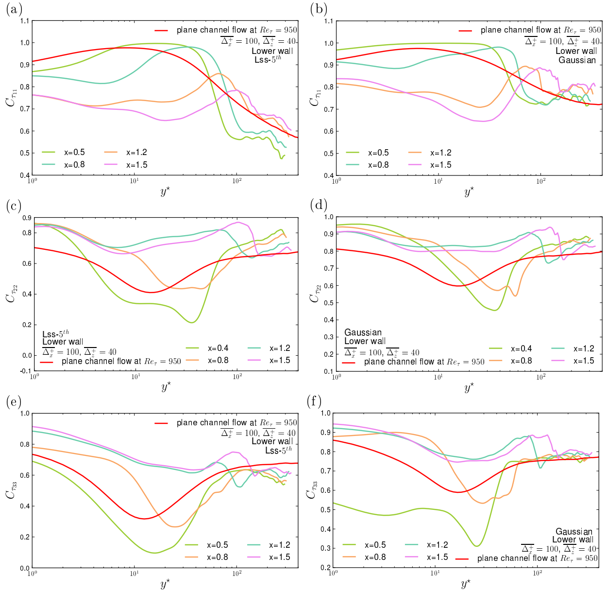
Figure B.12: Wall normal profiles of correlations C_{\tau_{11}} , C_{\tau_{22}} and C_{\tau_{33}} at the lower wall using Lss-5 th (a, c, e) and Gaussian (b, d, f) filter width \overline{\Delta_x^+} = 100 , \overline{\Delta_z^+} = 40 .
