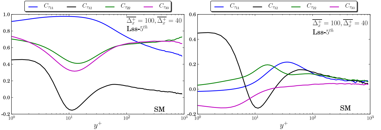
Figure 4.34: Correlations C_{\tau_{ij}} between exact SGS stress tensor and the modeled counterparts by Smagorinsky model using Lss-5 th filter.
