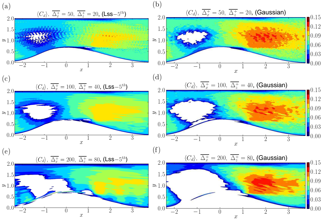
Figure 5.20: A priori estimate of coefficient \langle C_d \rangle of Dynamic Smagorinsky model in converging-diverging regions with three filter widths ( \widehat{\Delta} = 2.0\overline{\Delta} ) using Lss-5 th (left) and Gaussian (right) filters.
