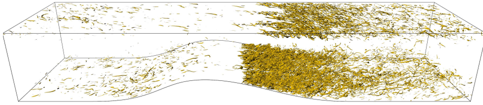
Figure 3.17: Iso-value of the Q-criterion ( Q = \frac{1}{2}[|\Omega|^2 - |S|^2] with S = \frac{1}{2}[\nabla u + (\nabla u)^T] and \Omega = \frac{1}{2}[\nabla u - (\nabla u)^T] ) for the whole simulation domain.
