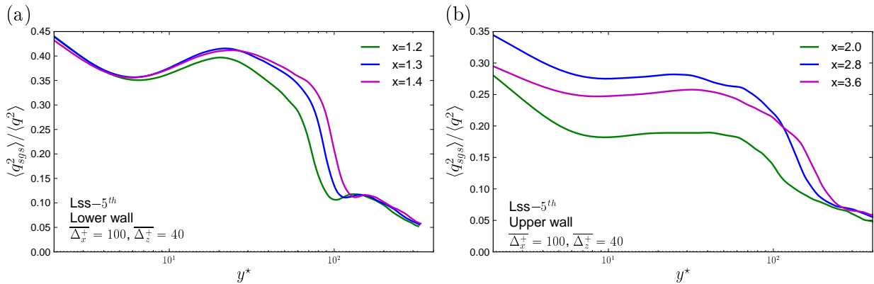
Figure 5.3: One-dimensional fraction of subgrid scale kinetic energy to the total turbulent kinetic energy at diverging lower wall (a) and flat upper wall (b) regions using Lss-5 th filter set ( \Delta_x^+ = 100, \Delta_z^+ = 40 ).
