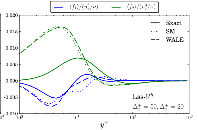
Figure 4.46: Exact f_i and its modeled counterparts by Smagorinsky model and WALE model using Lss-5 th filter.
