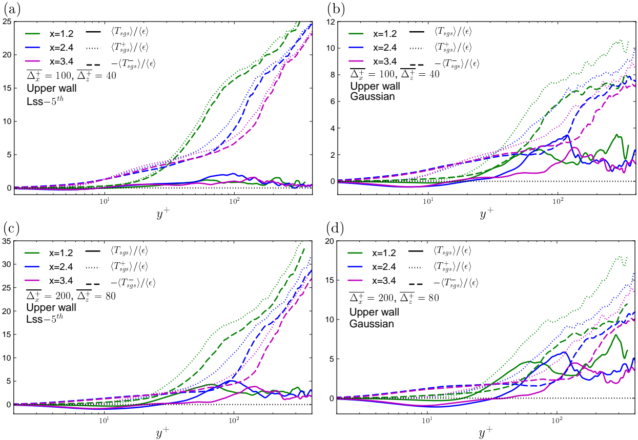
Figure 5.8: One-dimensional profiles of forward scatter of net SGS energy transfer in the diverging APG region at the upper wall, including the average of its positive and negative contributions using Lss-5 th (a, c) and Gaussian filter (b, d). Statistics are normalized by the rate of kinetic energy dissipation.
