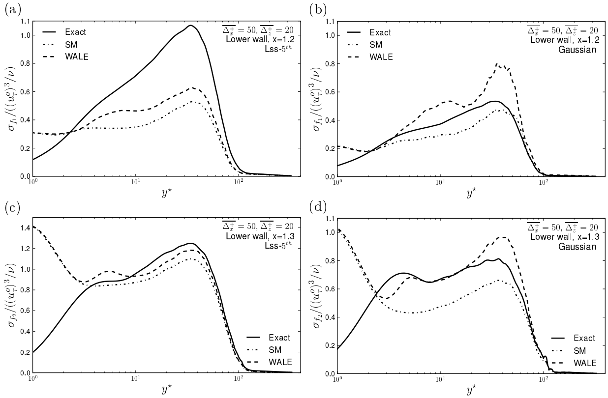
Figure B.17: Comparison of standard deviation of the exact f_1 , f_2 and the modeled counterparts obtained by the Smagorinsky and WALE models with filter width \overline{\Delta_x^+} = 50 , \overline{\Delta_z^+} = 20 using Lss-5 th (a, c) and Gaussian (b, d) filters at the lower wall.
