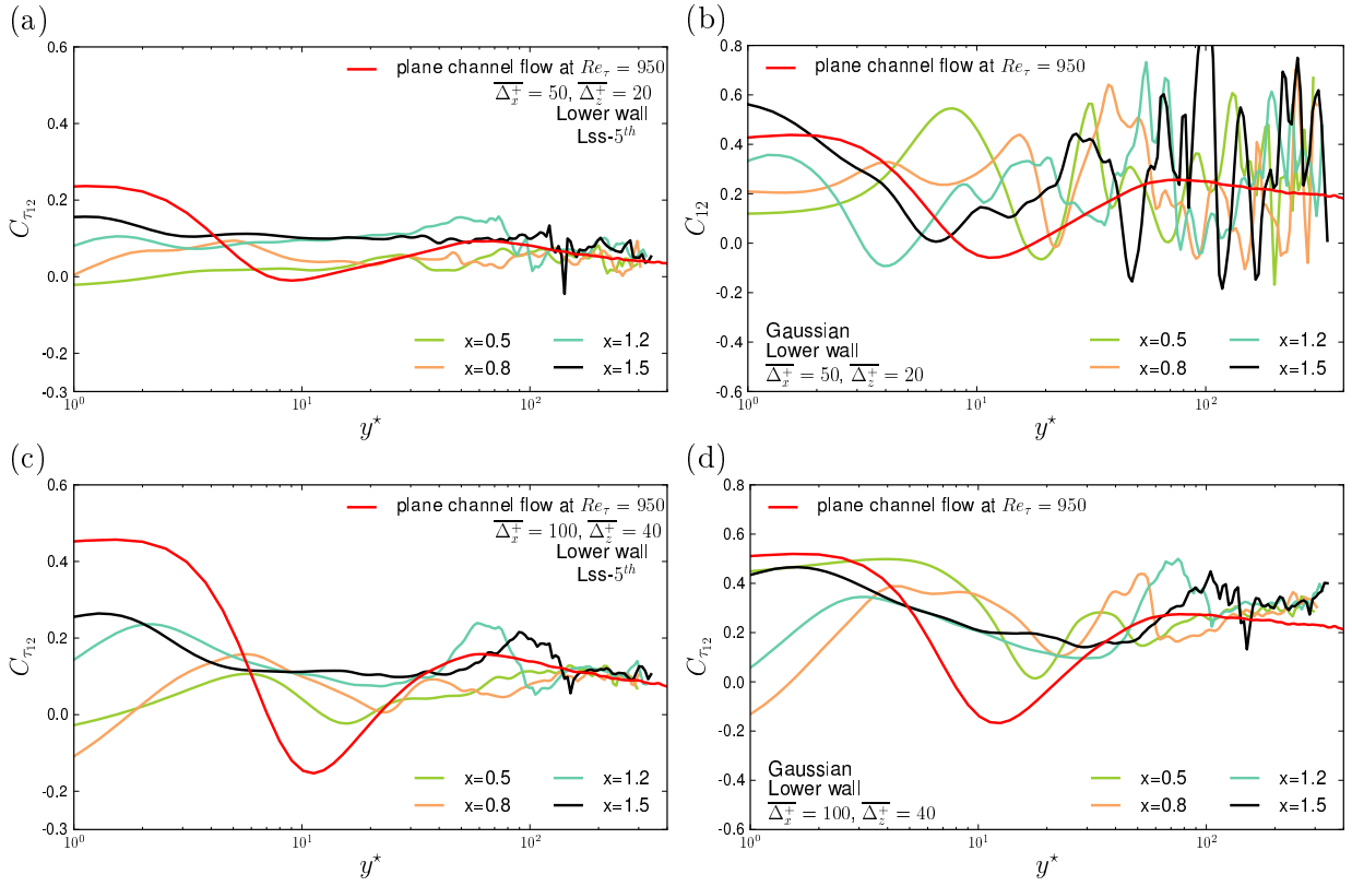
Figure 5.35: One-dimensional profiles of correlation C_{\tau_{12}} at the lower wall using Lss-5 th (a, c) and Gaussian (b, d) filters.
