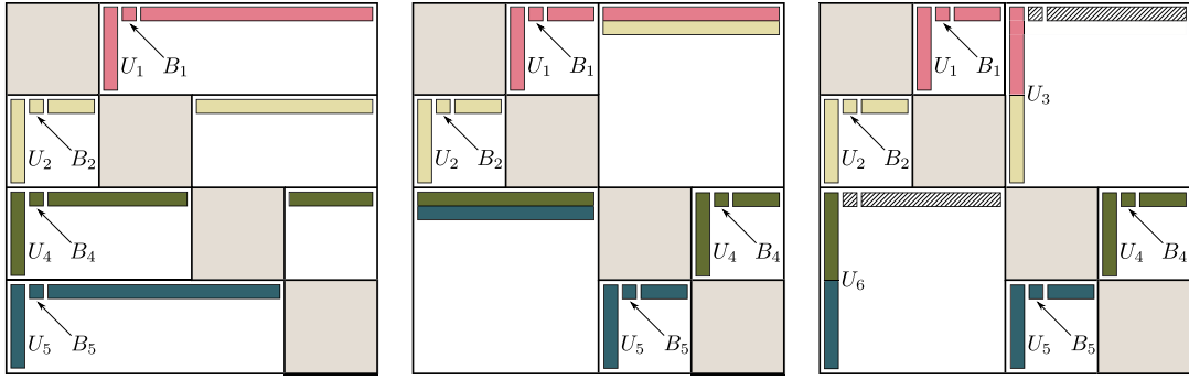
(a) First step of row compression at the leaf level l . The blockrows are entirely compressed. (b) Second step of row compression level (parents of the leaves). Matrices generated through compression at previous level are partly merged. (c) After the merge, blockrows at the l - 1 level are recompressed.
