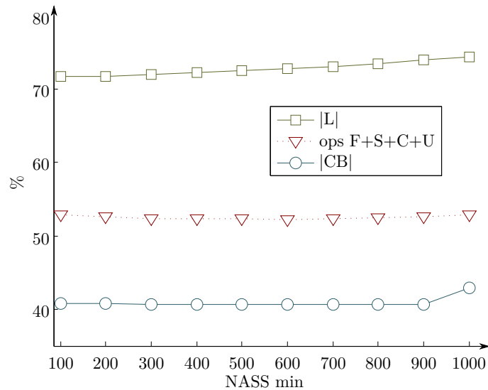
Figure 4.6: Influence of the minimal size of the separator (NASS min) required for a frontal matrix to be selected for BLR processing on the Helmholtz128 problem. The low-rank threshold is set up to \varepsilon = 10^{-8} and the cluster size is 448.
