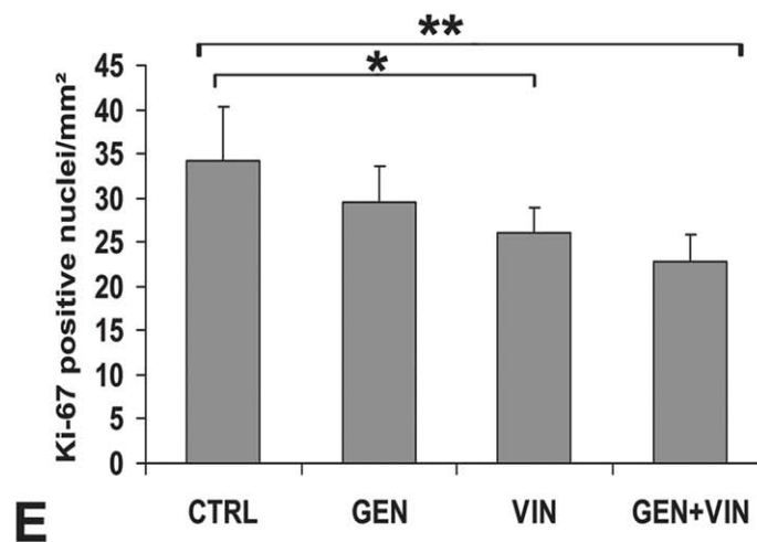
FIGURE 3.—Proliferation of submandibular salivary glands in PND35 female rat offspring after gestation-lactation exposure to 1 mg/kg body weight of genistein (GEN), vinclozolin (VIN), and the mixture (GEN+VIN). Immunohistochemical photomicrographs of Ki-67 ( \times 400 ) expression in submandibular salivary gland (SSG) sections. The Ki-67–positive cells have brown-stained nuclei. Note the presence of numerous Ki-67–positive nuclei (arrows) in the CTRL group (A) and the presence of rare mitotic nuclei in the GEN- (B), VIN- (C), and GEN+VIN- (D) treated groups for these sections. The number of Ki-67–positive nuclei decreases in the VIN and GEN+VIN groups (E). Values are expressed as mean \pm SD per mm 2 (n = 6). Different intergroup values (Tukey test) are indicated by the following symbols: ** p < .01 ; * p < .05 .
