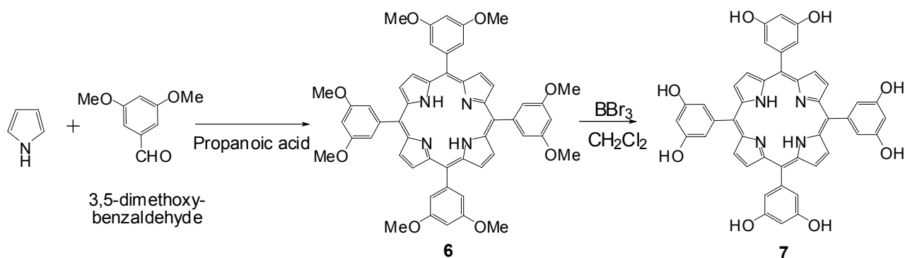
Scheme 3 : Synthesis of the porphyrin precursor 7
