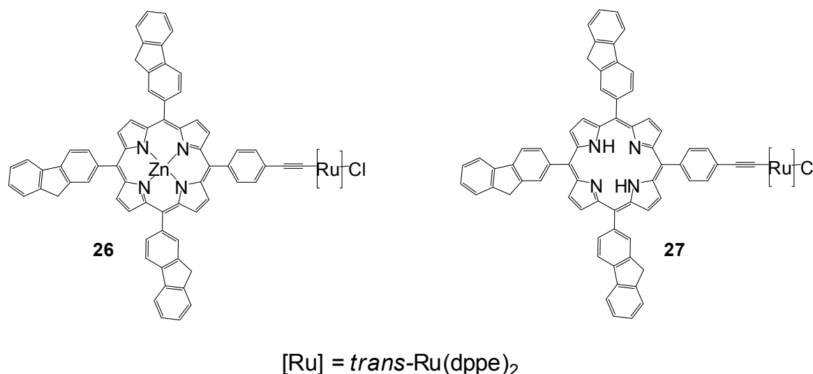
Figure 12 : Proposed target molecules 26 and 27
