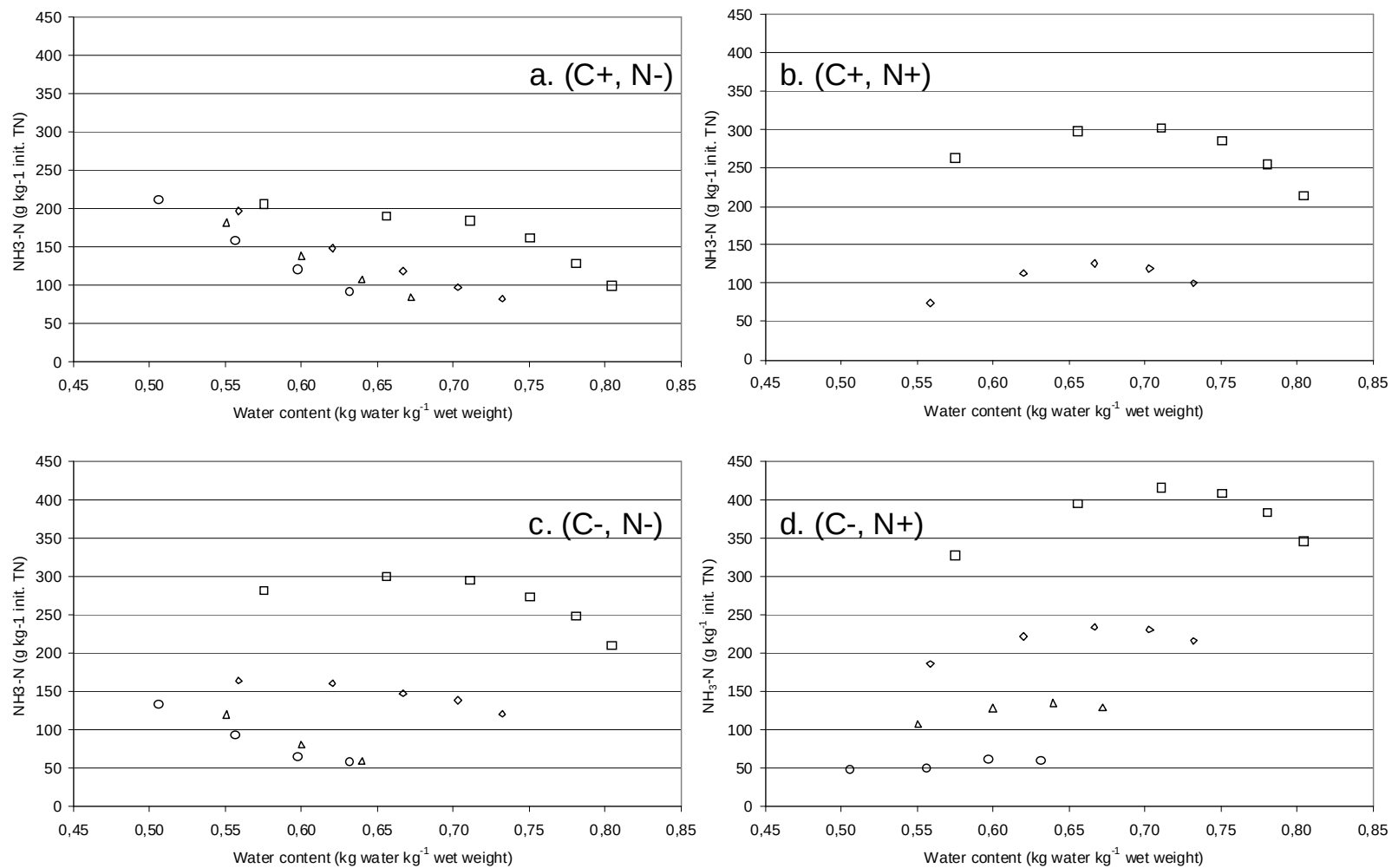
Figure 19. Simulation of the cumulative \text{NH}_3\text{-N} emissions after 56 composting days (g \text{kg}^{-1} initial nitrogen) as a function of water content (kg water \text{kg}^{-1} wet weight) for four couples ( C_{\text{biodeg}} , N_{\text{av}} ) (a, b, c, d) and for four dry matter densities : 100 (squares), 150 (diamonds), 200 (triangles) and 240 (circles) \text{kg DM m}^{-3}
