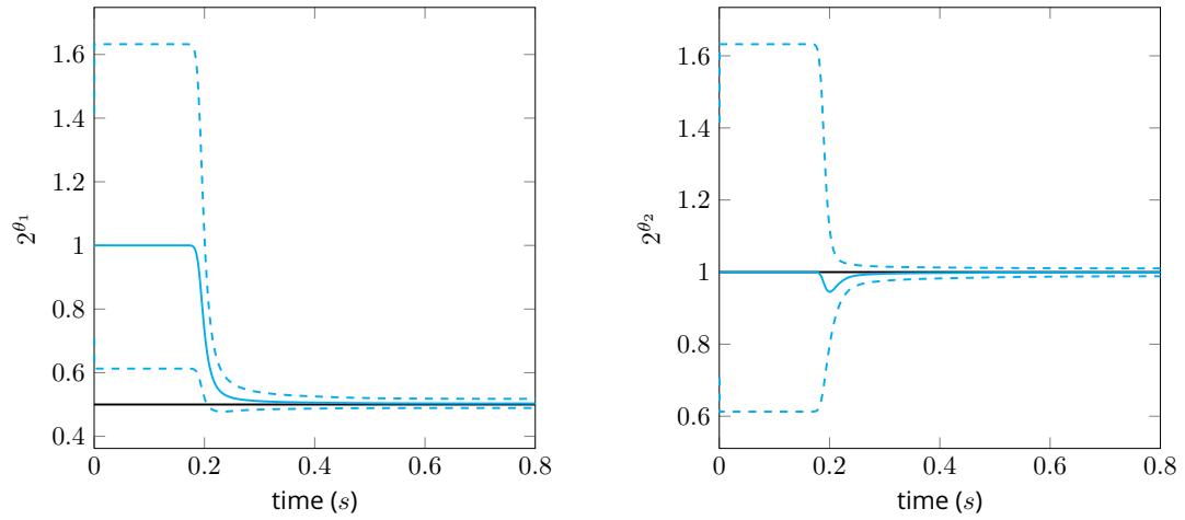
Figure 2.2: Estimation of active parameters using endo- and epicardium synthetic segmentation, M_z = 10^7 \times \mathbb{M}_{S_0} .
