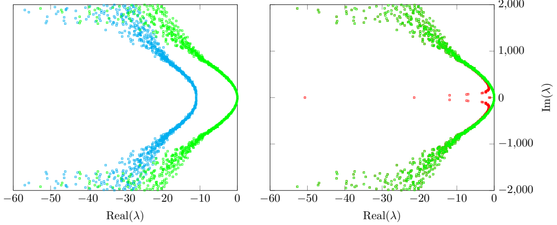
Figure 11: Spectrum of the stabilized operator using either the \mathcal{H}^{\frac{1}{2}} -norm (in (cyan)) and the \mathcal{L}^2 -norm (in (red)). In (green) are the modes of the original operator, i.e. without stabilization.
