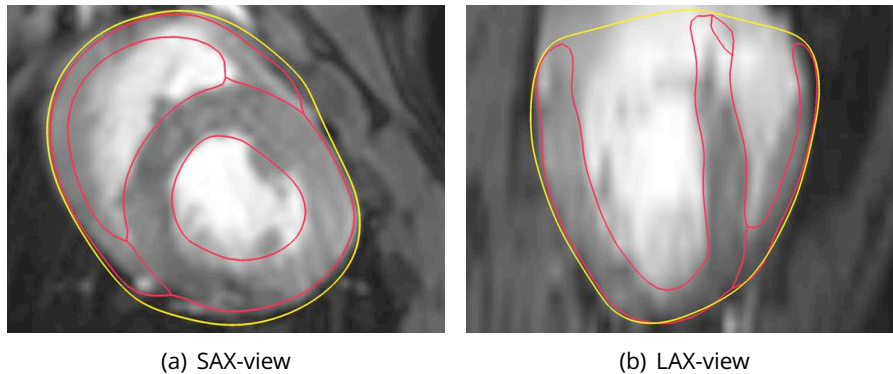
Figure 4.8: Contact surface (in yellow) for the direct model.
