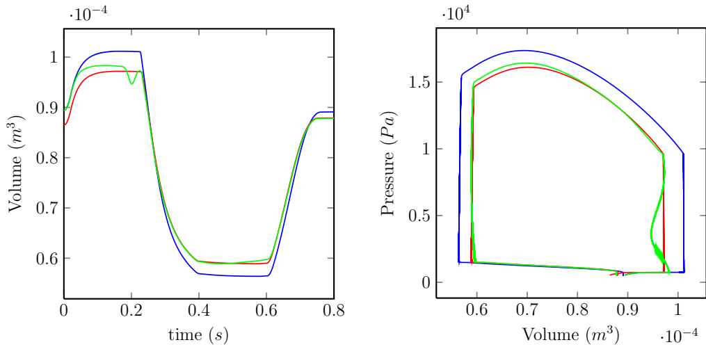
Figure 17: Evolution of the volume (in time) and of the P-V loop for the observer (in (green)) using tag planes with coarse time sampling of the observations and compared to the healthy direct model (in (blue)) and the observed infracted model (in (red)).
