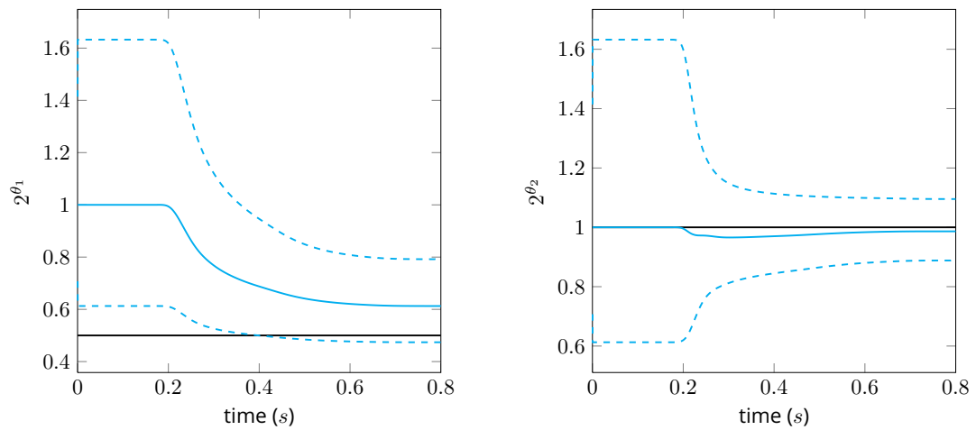
Figure 2.3: Estimation of active parameters using endo- and epicardium synthetic segmentation, M_z = 10^5 \times \mathbb{M}_{S_0} .
