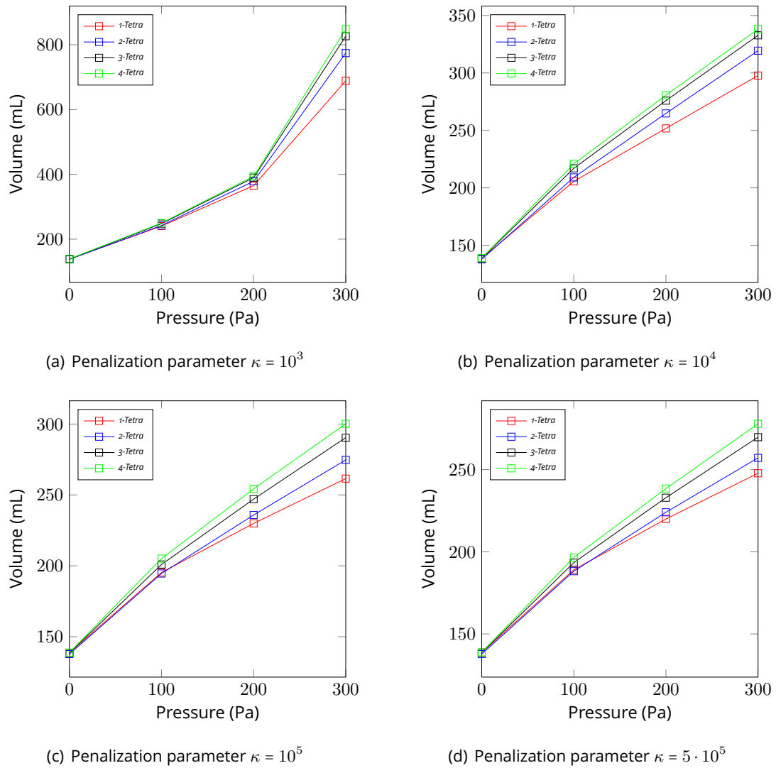
Figure 1.6: Evolution of the volume for various values of the penalization parameter.
