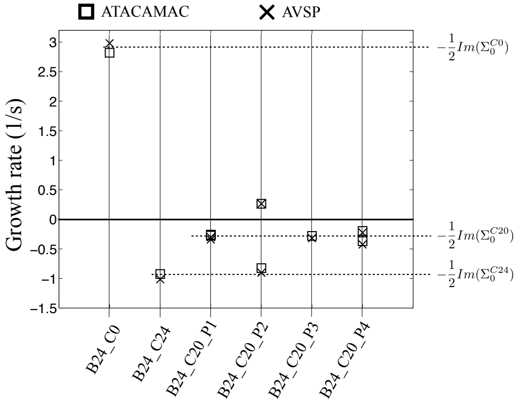
Figure 5.12: Growth rate of the first azimuthal mode ( p = 1 ) for various asymmetric combination of burners with and without CBO: B24_C0 (24 noCBO burner, perfectly symmetric case), B24_C24 (24 CBO burners, perfectly symmetric case) and the four patterns B24_C20 (non-symmetric cases). --- : Values of -\frac{1}{2}I_m(\Sigma_0) (necessary condition, Eq. (5.23)) depending on the configuration ( C_0 , C_{20} and C_{24} ).
