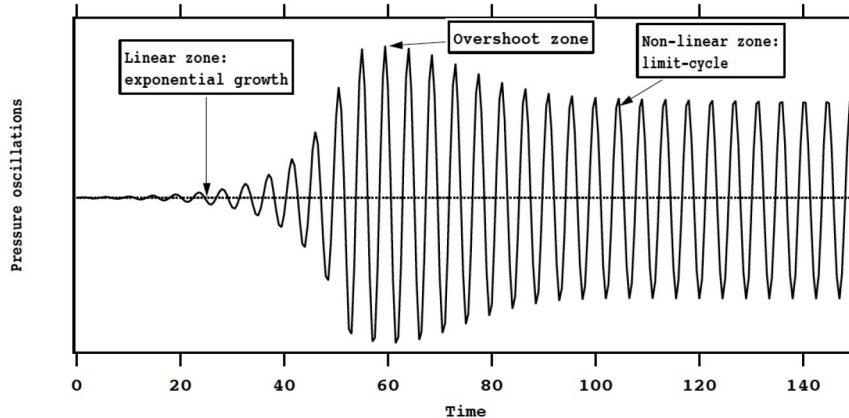
Figure 1.12: Typical time-evolution of a combustion instability: exponential growth of the acoustic pressure followed by an overshoot before reaching a limit cycle [117].
