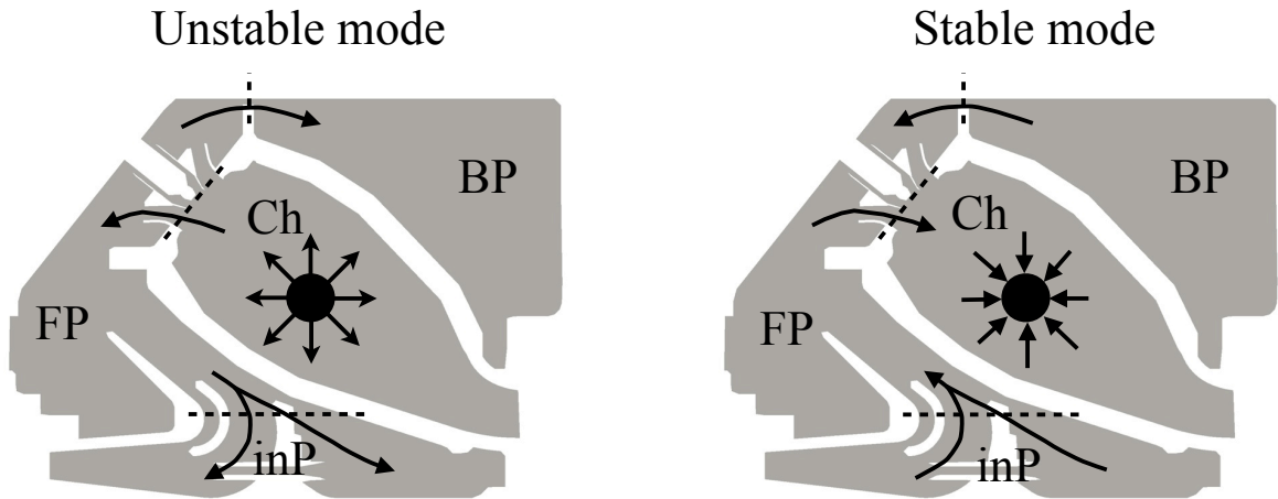
Figure 6.21: Direction of the acoustic fluxes depending on whether the chamber is an energy source (left) or and energy sink (right).
