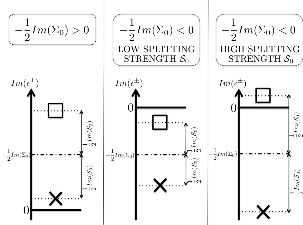
Figure 12: Several situations depending on the condition Eq. (35) and the splitting strength \frac{1}{2}Im(\mathcal{S}_0) . \times : \epsilon^- and \square : \epsilon^+
