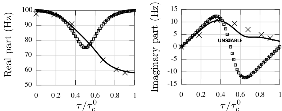
Figure 17: Eigenfrequency of the first order chamber mode ( p = 1 ) for four burners ( N = 4 ) as a function of \tau/\tau_c^0 with n_i = 8.0 . — : Numerical resolution of Eq. (25), \square : Analytical model prediction for weakly coupled situations (Eq. (47)), \times : AVSP results
