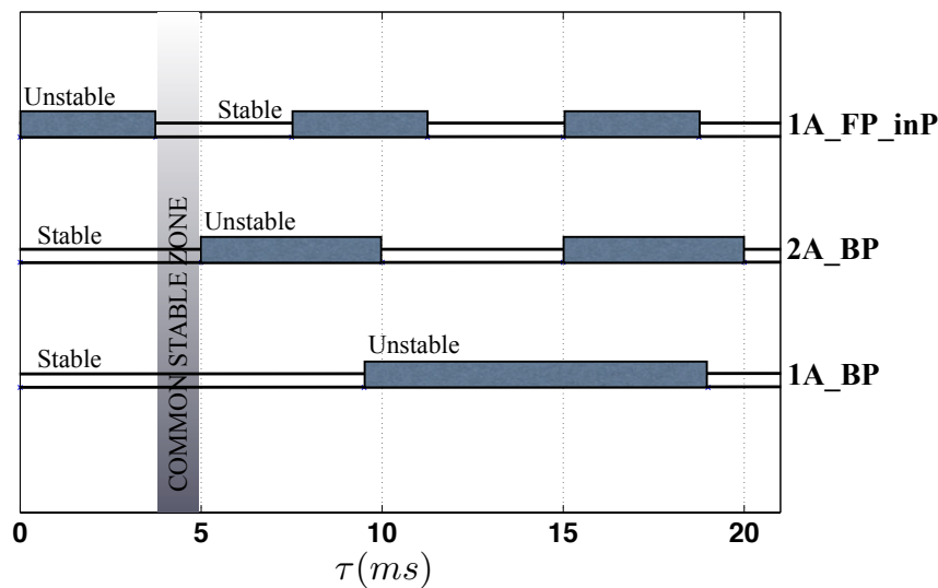
Figure 6.30: Stability map of the 1A_BP, 2A_BP and 1A_FP_inP modes as a function of \tau . The only values of \tau that ensures the simultaneous stability of the three modes are between 4 and 5 ms approximately.
