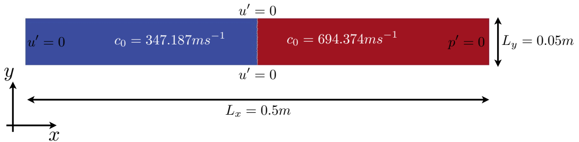
Figure 4.1: 2D rectangle with temperature jump.
