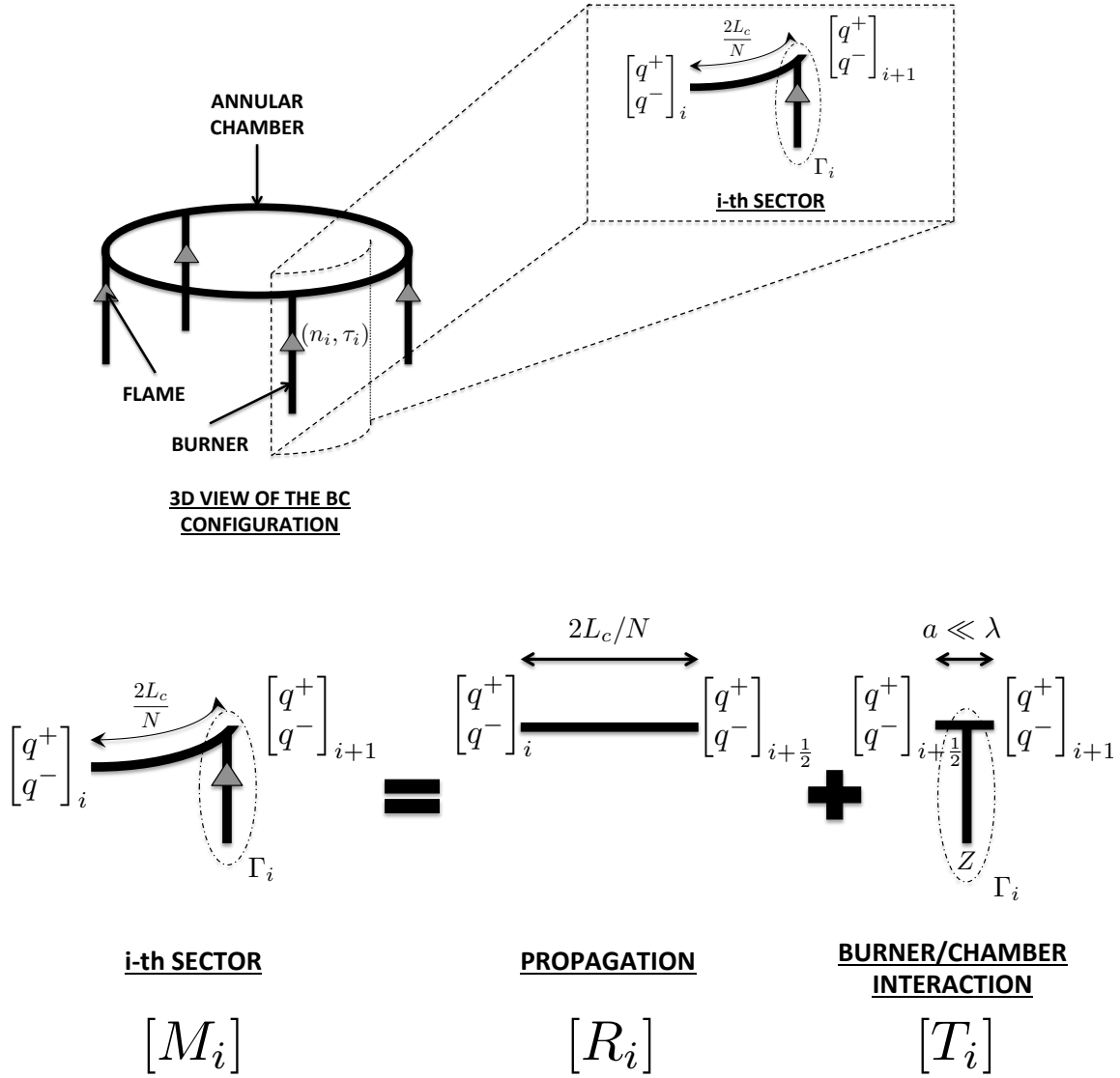
Figure 5.6: Schematic 3D view of a BC configuration with N = 4 burners. Zoom on the i^{\text{th}} sector, where \Gamma_i represents the burner/chamber interaction [111] (top). Each sector is decomposed into a free propagation of azimuthal waves q^+ and q^- (characteristic length 2L_c/N ) and a compact burner/chamber interaction (characteristic length a \ll \lambda ) modeled by the coupling parameter \Gamma_i (bottom).
