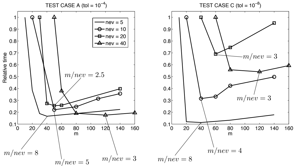
Figure 4.12: Influence of the ratio m/nev on the computation time for test cases A and C.
