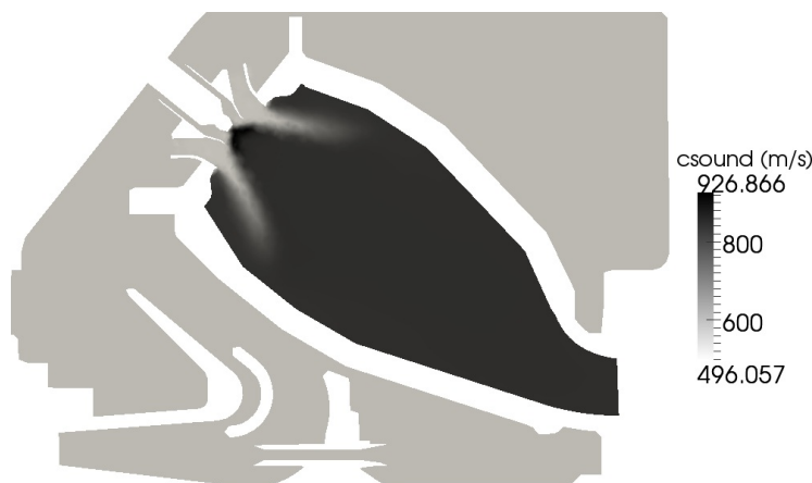
Figure 6.4: Longitudinal cut: sound speed c_0(\vec{x}) field obtained from a LES time-average solution used for AVSP simulations.
