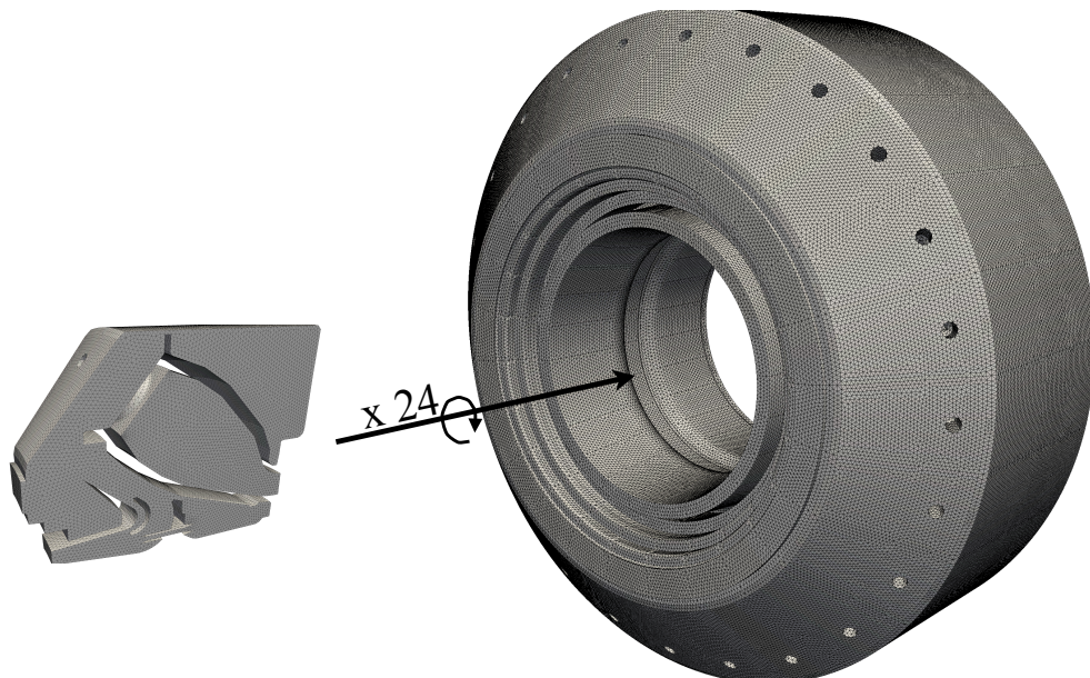
Figure 6.3: 360° mesh obtained from a single sector mesh used for AVSP simulations: 1,782,384 nodes and 9,527,472 cells.
