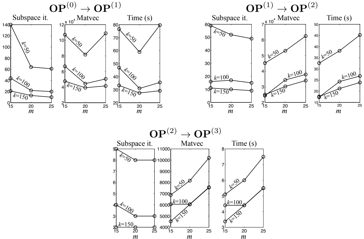
Figure 4.22: Test case A: Computational cost (number of restarted iteration, matrix/vector products and runtime) of the computation of 10 smallest magnitude eigenvalues associated with the sequence of linear problems \mathbf{OP}^{(1)} , \mathbf{OP}^{(2)} and \mathbf{OP}^{(3)} obtained during the computation of the smallest magnitude nonlinear eigenvalue \omega_1 ( k : degree of the Chebyshev polynomial; m : size of the subspace).
