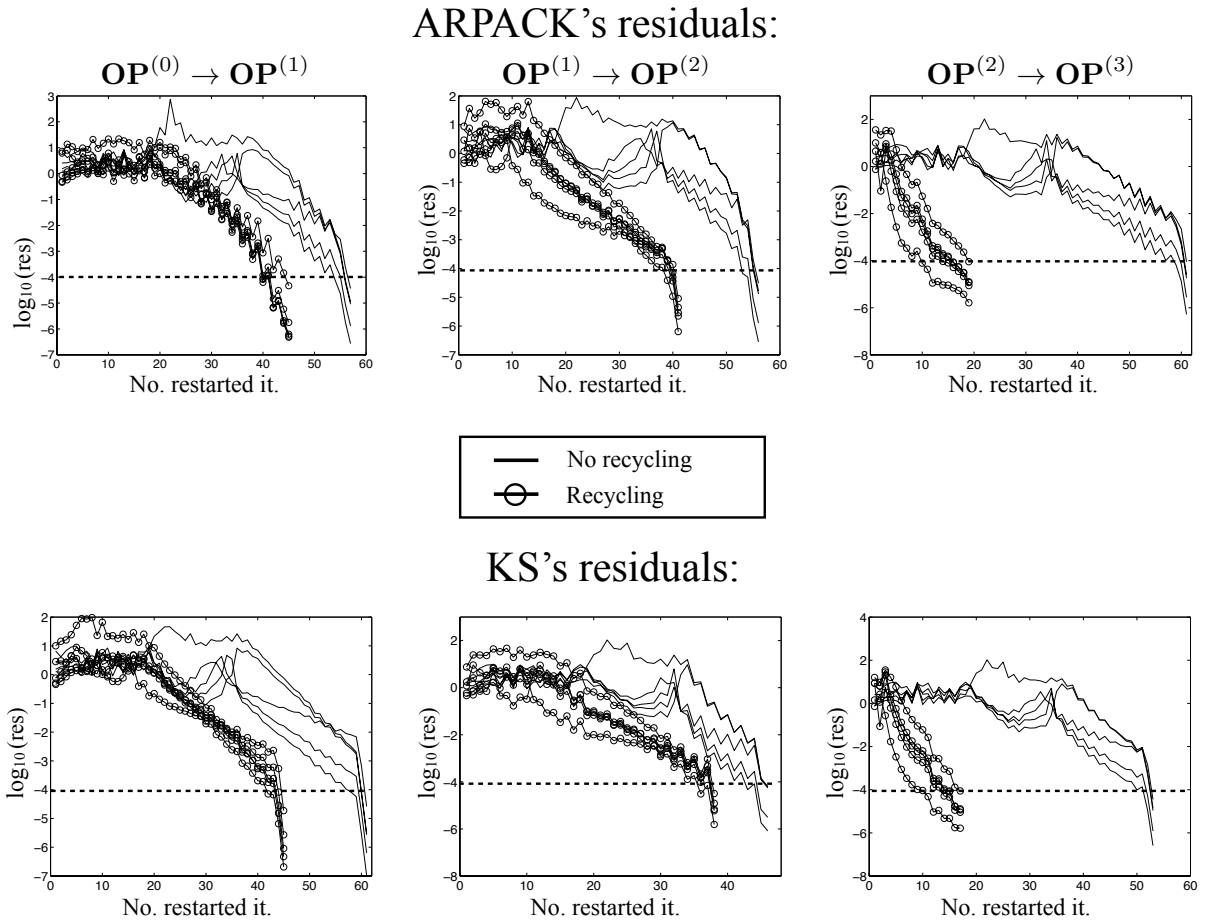
Figure 4.19: Test case A: Residuals corresponding to the nev = 5 smallest magnitude eigenpairs of the sequence of linear problems OP^{(1)} , OP^{(2)} and OP^{(3)} solved with tol = 10^{-4} for the computation of the smallest magnitude nonlinear eigenfrequency \omega_1 . ( -\circ- ): with recycling strategy; ( --- ) without recycling strategy.
