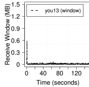
(c): Receive Window.
