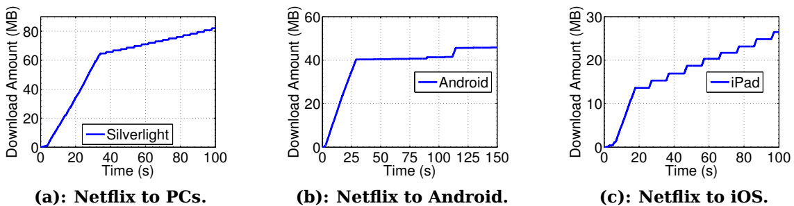
Figure B.1: Netflix Streaming Strategies
