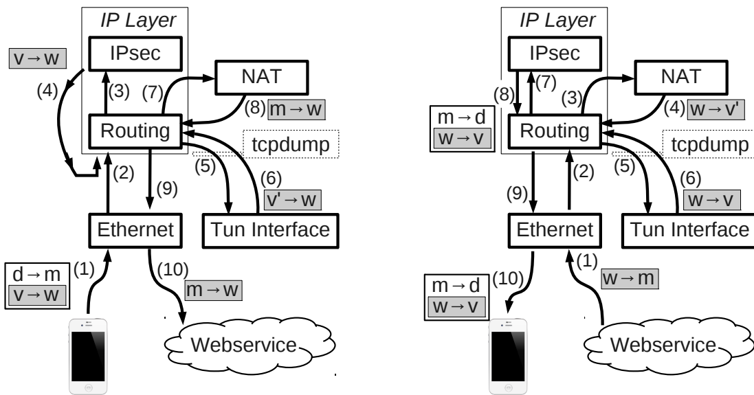
(c): Packet from mobile device. Tcpdump captures packets at step (5) v \rightarrow w , and (6) v' \rightarrow w .
