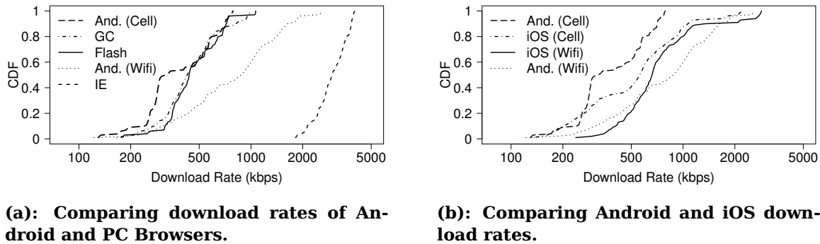
Figure 4.10: Comparison of download rates. Among desktop browsers, only Internet Explorer (IE) streaming HTML5 videos is more aggressive than Android. Android is less aggressive compared to iOS when using cellular networks because Android explicitly demands user’s permission to stream high quality videos when using cellular networks.
