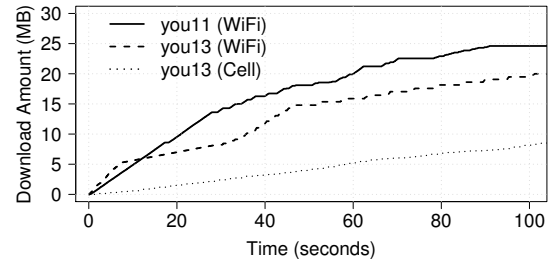
(b): Sample iOS streaming session.
