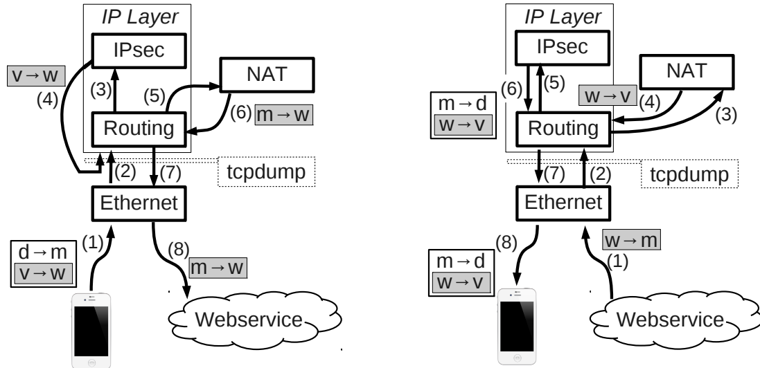
(a): Packet from mobile device. Tcpdump captures packets at step (2) d \rightarrow m , (4) v \rightarrow w , and (7) m \rightarrow w .
