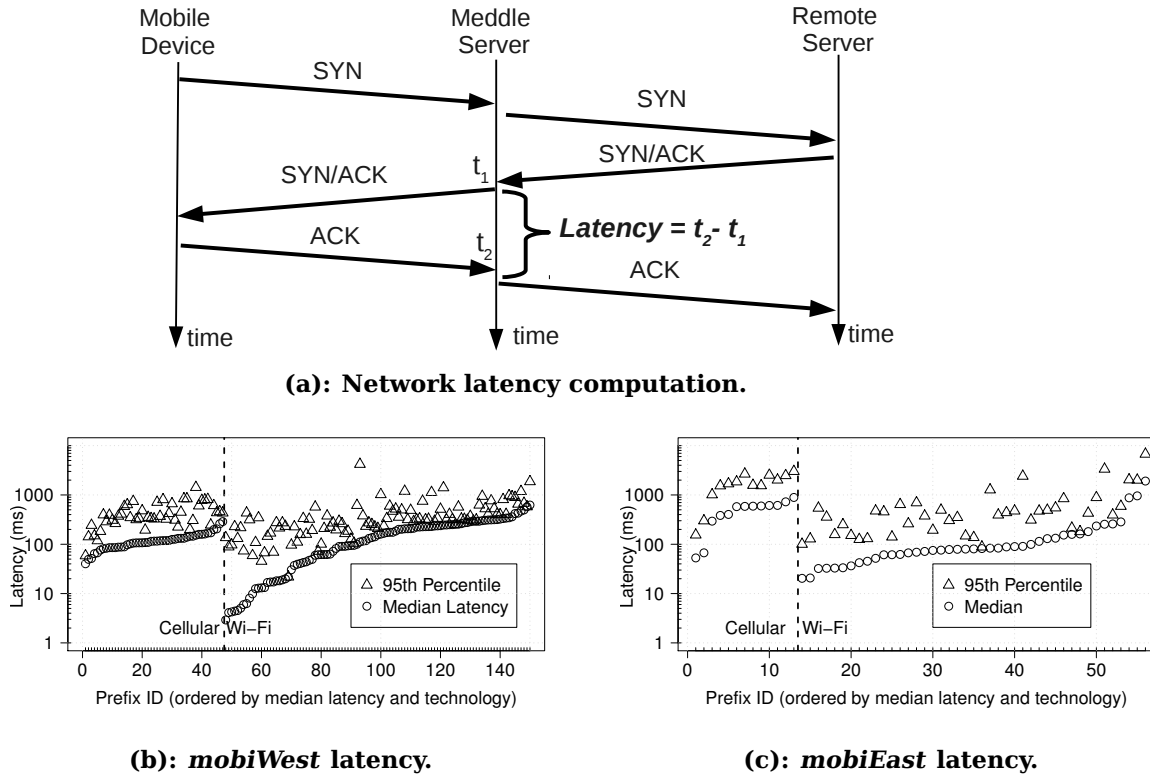
Figure 2.4: Network latency to Meddle servers. The network latency between Meddle servers and the devices is measured as the time between the SYN/ACK and ACK packet of a TCP three way handshake. We observe a median latency of less than 1 second across majority of prefixes through which devices tunneled their traffic.
