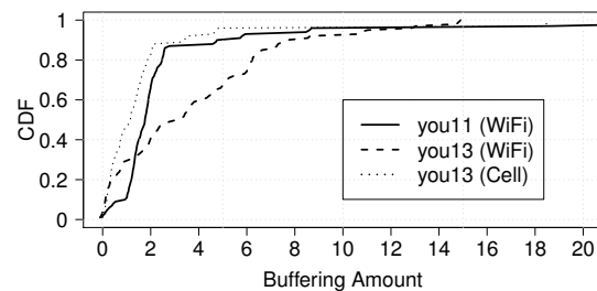
(b): Buffering Amount (iOS).
