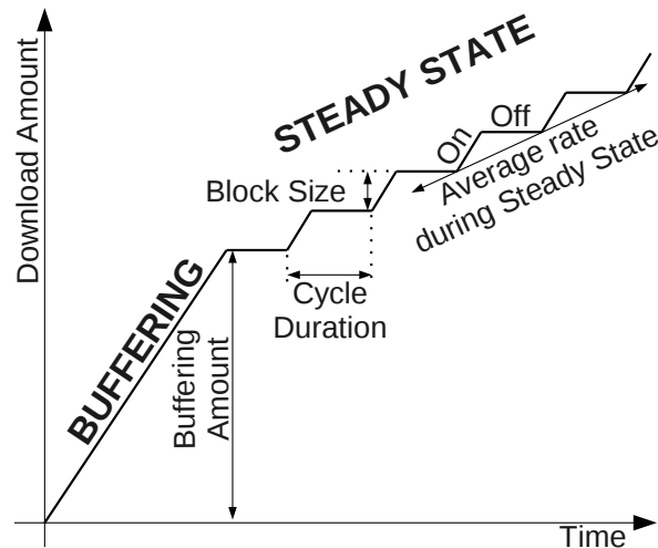
Figure 4.1: The two phases of video download. Video streaming begins with a buffering phase followed by a steady state phase. Cycles of ON-OFF periods in the steady state phase are used to throttle the data transfer rate.
