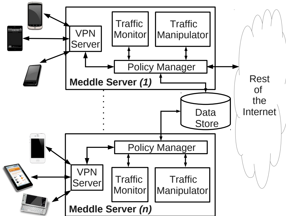
Figure 2.1: Meddle’s Architecture. Devices use VPN connections to tunnel all traffic to one of the potentially many Meddle servers. Each Meddle server uses a device-specific profile to determine the set of services that operate on the network traffic.
