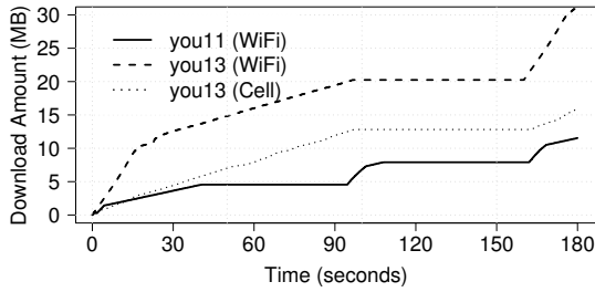
(a): Sample Android streaming session.
