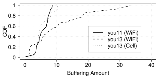
(a): Buffering Amount (Android).
