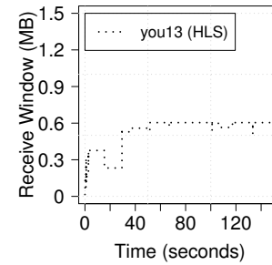
(d): Receive Window.
