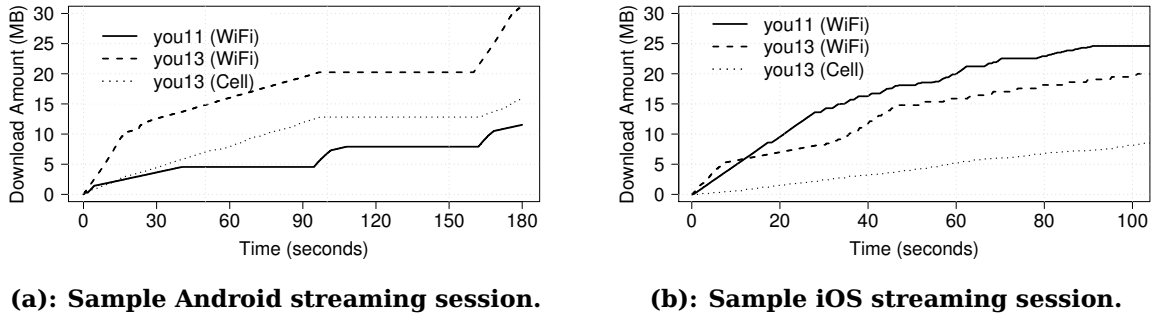
Figure 4.8: Sample streaming session to mobile devices. We observe iOS and Android use large blocks to download multiple copies of the video content, each of which is encoded using a different encoding rate.
