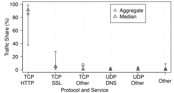
(e): mobiEast Android. A higher share for HTTP traffic over SSL is because the custom ROMs such as Xiaomi and MIUI rely on HTTP to provide services such as searching for apps on their default stores.
