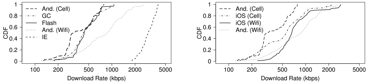
(a): Comparing download rates of Android and PC Browsers.
