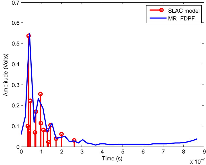
Figure 4.19: The comparison of the impulse response.
