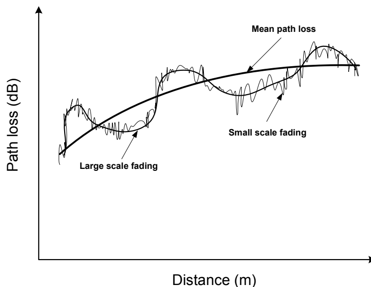
Figure 1.1: The instantaneous path loss.
