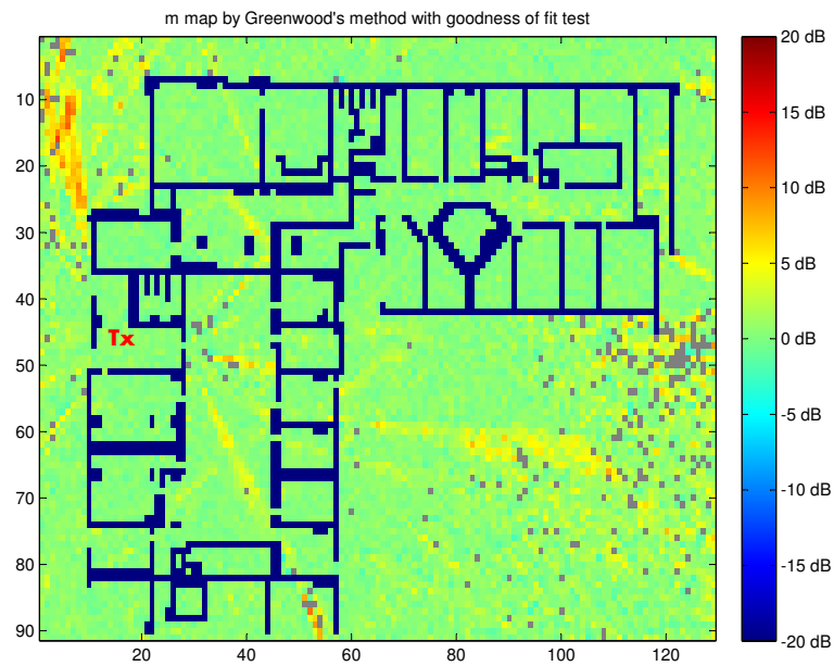
Figure 5.6: The m parameter map by the Greenwood's method with goodness of fit test.
