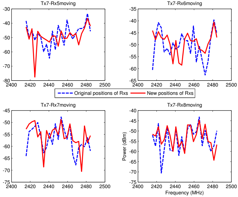
Figure 6.7: The comparisons of the wideband fast fading characteristics of the links between the Tx7 and the Rx5-8 when moving the Rxs with 2cm.
