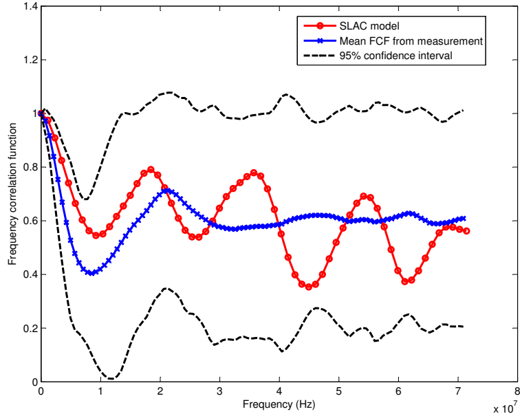
Figure 4.23: The comparison of FCFs obtained from the SLAC model and measurements.
