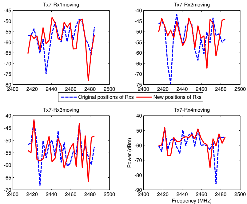
Figure 6.6: The comparisons of the wideband fast fading characteristics of the links between the Tx7 and the Rx1-4 when moving the Rx's with 2cm.
