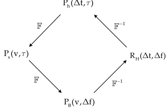
Figure 3.3: Interrelations among P-functions for WSSUS channels.
