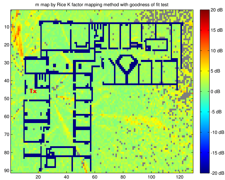
Figure 5.5: The m parameter map by the Rice K factor mapping method with goodness of fit test.
