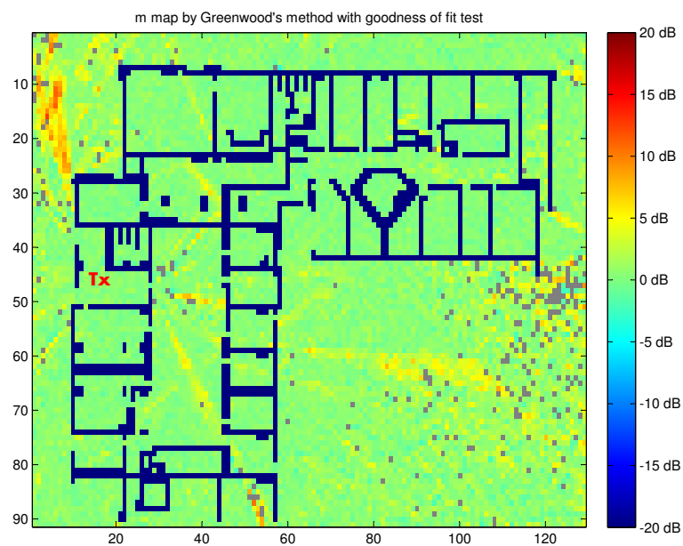
Figure 5.6: The m parameter map by the Greenwood's method with goodness of fit test.
