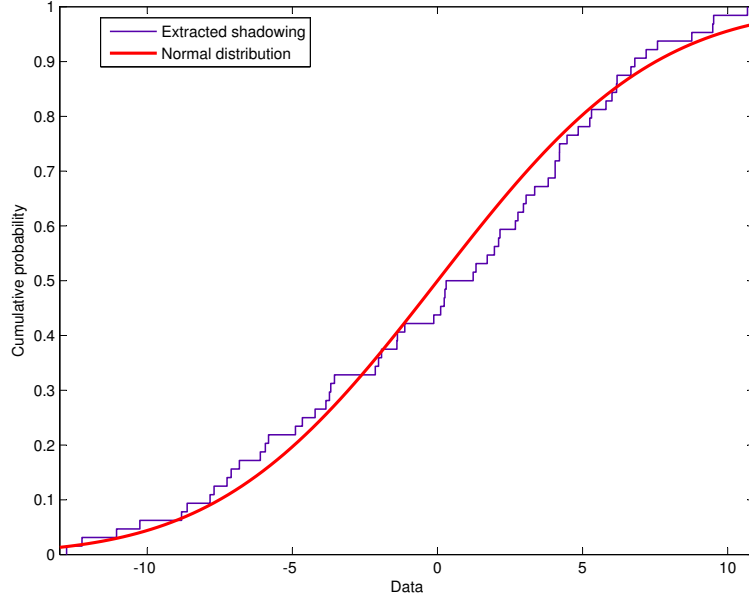
Figure 4.14: CDF comparison between the extracted shadow fading from the MR-FDPF model and normal distribution.
