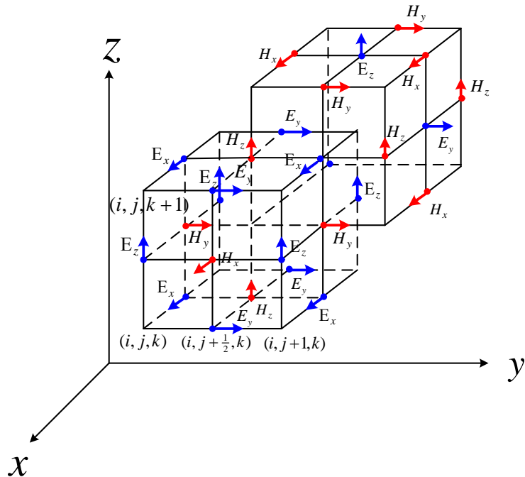
Figure 2.5: Yee grid.
