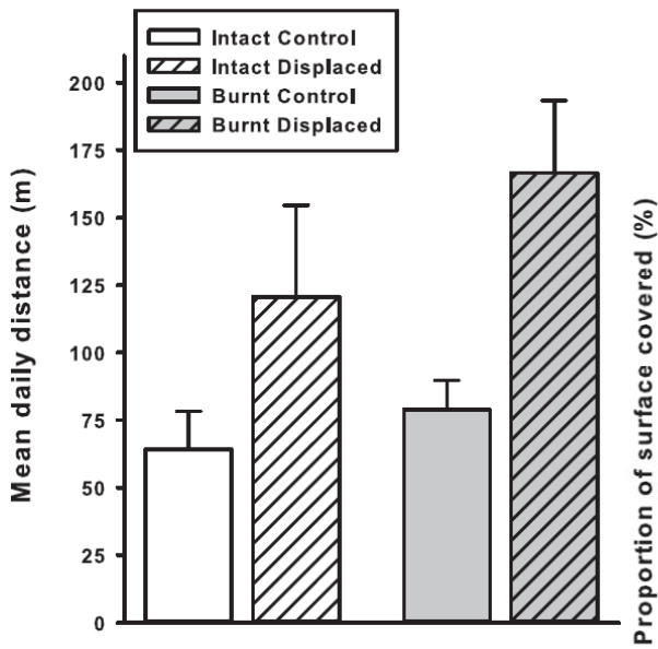
Figure 5: Mean daily distance ( \pm 1SE ) travelled by control ( N=12 , open bars) and displaced tortoises ( N=12 , hatched bars). Intact area and burnt areas are indicated in white and grey respectively (sample size was 6 for each bar).
