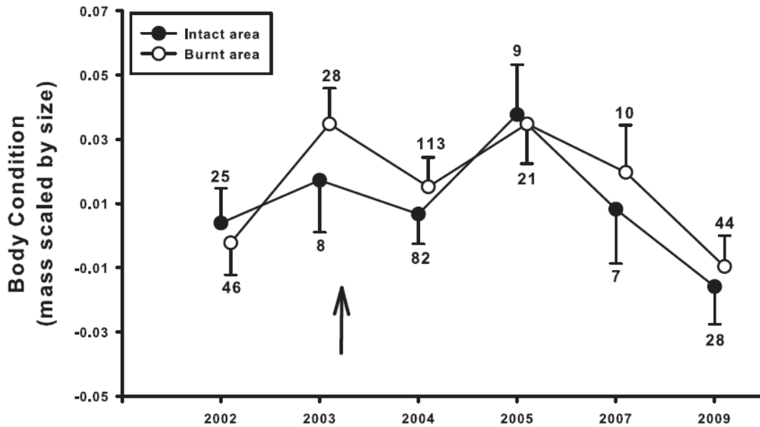
Figure 3: Comparison of the mean body condition (mass scaled by size) of tortoises monitored in two areas, intact versus burnt. The arrow indicates a major fire event (summer 2003). Means calculated for 2004 include tortoises found in late 2003, after the fire. Means are expressed \pm 1SE , numbers indicate sample size. Due to small sample size ( N < 10 tortoises observed per year) means could not be reliably calculated in 2006 and 2008.
