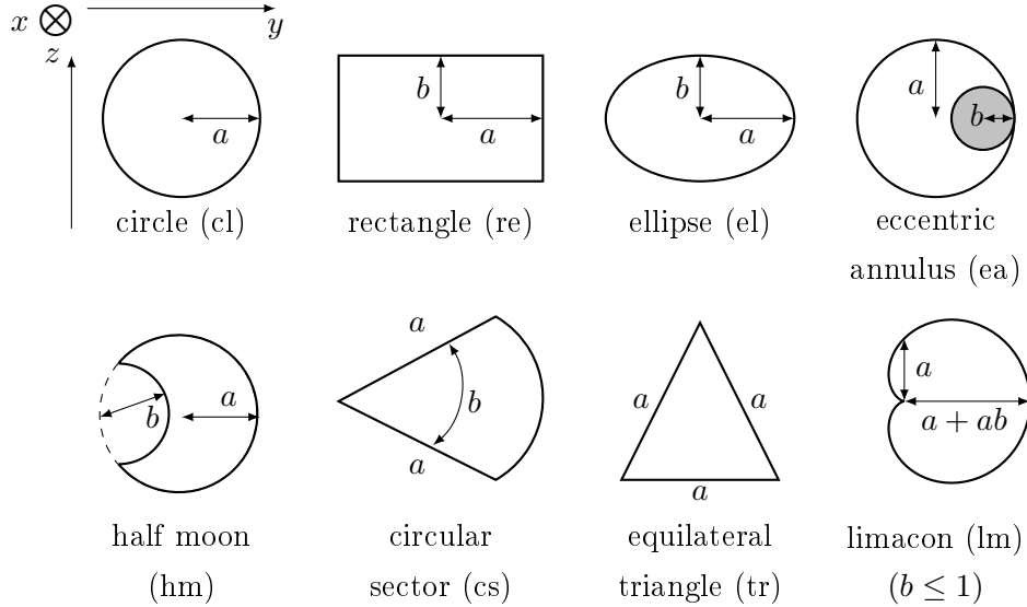
Figure 2.3: cross section shapes with parameters ( a, b ) in the ( y, z ) plane. Note that for a circular sector, b indicates an angle. As in Fig. 2.1, x denotes the streamwise, y the spanwise and z the transverse direction.
