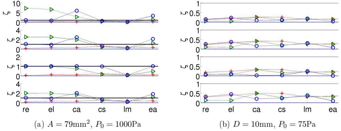
Figure 4.10: Illustration of \zeta for a smooth expansion and default parameter set (+), non-default parameter set (▷), fixed width (o) for different geometrical, fluid and flow configurations. For subplots in Fig. 4.10a and Fig. 4.10b values of R_c , L_c/D_{cl} and \mu are the same as indicated in Fig. 4.9a.
