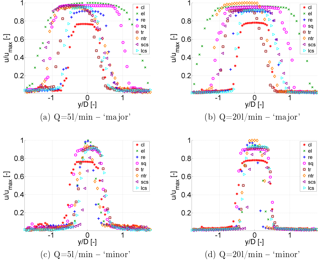
Figure 5.22: Measured normalized transverse mean velocity profiles u/u_{max} following the ‘major’ and ‘minor’ axis defined in Fig. 5.3a as a function of the cross section shape for volume flow rate Q = 5\text{l/min} and Q = 20\text{l/min} in the case of sharp edges at the constriction inlet (label C in Table 5.4). u_{max} denotes the maximum mean velocity for all cross section shapes at a given volume flow rate.
