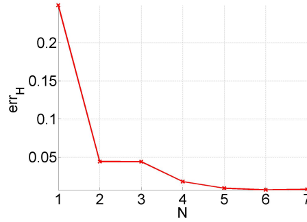
Figure 3.3: Illustration of relative boundary error err_N^H as a function of truncated sum number N for Dirichlet problem of Helmholtz equation. The shape with stretched parameters (Table 3.1) is assessed in domain \Omega .
