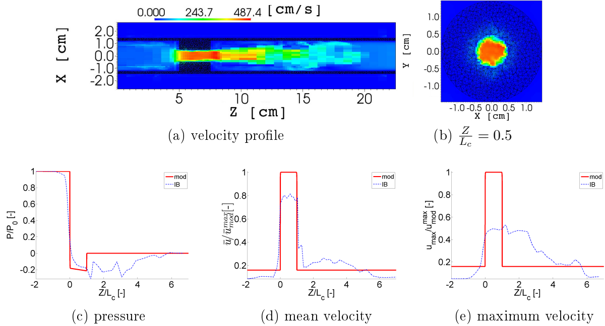
Figure 6.18: Illustration of flow field for a channel with circular constriction for upstream pressure P_0 = 10 Pa. Simulated (IB) quantities are obtained at time t = 90 ms: a) instantaneous simulated (IB) streamwise velocity magnitude, b) instantaneous simulated (IB) transverse velocity magnitude at the middle of the constriction ( Z/L_c = 0.5 ), c) normalized modeled (mod) and simulated (IB) streamwise pressure distribution, d) normalized modeled (mod) and simulated (IB) mean streamwise velocity distribution and e) normalized modeled (mod) and simulated (IB) streamwise velocity distribution along the centerline of the constriction.
