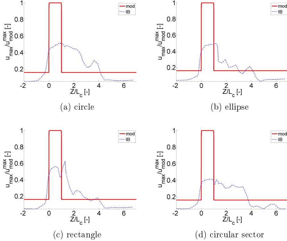
Figure 6.12: Modeled (mod) and simulated (IB) streamwise velocity distributions are normalized by the maximum modeled velocity u_{mod}^{max} . Simulated and modeled values are sampled at the transverse (X,Y) position associated with the maximum velocity in the analytical model for viscous developed flow through a constricted channel as outlined in chapter 2. for a volume rate obtained from the quasi-three-dimensional model described in chapter 4. Instantaneous simulated values are assessed at time t = 43\text{ms} for the circular constriction shape and at time t = 50\text{ms} for the other constriction shapes.
