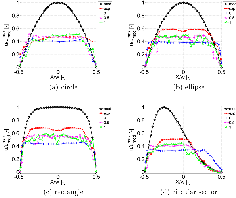
Figure 6.13: Illustration of normalized transverse velocity distributions along the X direction: modeled (mod), experimental (exp) and simulated (IB). Simulated profiles are shown for different streamwise positions within the constriction: at the inlet ( Z/L_c = 0 ), in the middle ( Z/L_c = 0.5 ) and at the outlet ( Z/L_c = 1 ). Instantaneous simulated profiles are assessed at time t = 43\text{ms} for the circular constriction shape and at time t = 50\text{ms} for the other shapes. The X coordinate is normalized by the the width of the constricted portion w along the X dimension.
