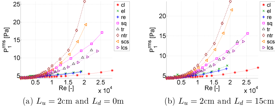
Figure 5.12: Measured root mean pressure values within the constriction P_1^{rms} for L_u = 2\text{cm} (label A in Table 5.4).
