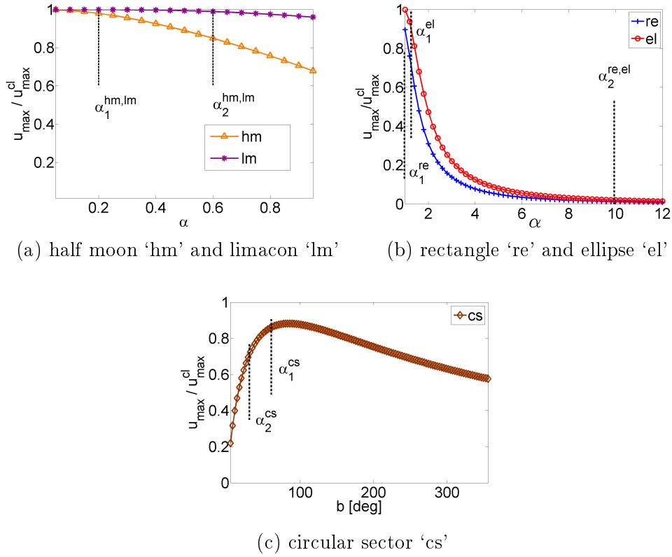
Figure 2.4: Illustration of the influence of geometrical parameter \alpha on normalized maximum velocity, u_{max}/u_{max}^{cl} , for different cross section shapes and imposed area A = 79 \text{ mm}^2 . Vertical lines indicate values corresponding to default parameter set ( \alpha_1 ) and non-default parameter set ( \alpha_2 ) for which u_{max}/u_{max}^{cl} \approx 1 and u_{max}/u_{max}^{cl} \ll 1 , respectively.
