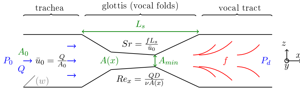
Figure 4.11: Schematic overview of main flow (blue), geometrical (green) and acoustic (red) quantities to determine non-dimensional numbers motivating simplified flow descriptions applied in phonation models. Upstream pressure P_0 , downstream pressure P_d , volume flow rate Q , inlet cross section area A_0 , minimal glottal area A_{min} , streamwise varying area A(x) , glottal streamwise length L_s , acoustic auto-oscillation frequency f , inlet bulk velocity \bar{u}_0 , Reynolds number Re_x based on hydraulic diameter D and Strouhal number Sr . Note that, the channel has arbitrary cross section shape and hence the width w (in gray shade) is only relevant with respect to the particular case of a rectangular channel with fixed w .
