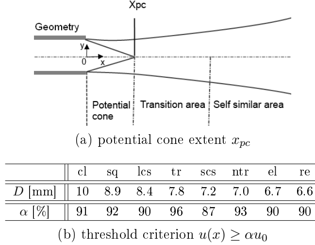
Figure 5.17: Free jet development: a) schematic overview of potential cone extent x_{pc} . b) Threshold \alpha as a function of the cross section shape applied to determine the potential cone extent x_{pc} presented in Fig. 5.19 [4]. For a round jet, 4 < x_{pc}/D < 8 [40].
