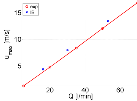
Figure 6.22: Illustration of the maximum velocity u_{\max} for a circular constriction along the centerline immediately downstream from the constriction ( Z/L_c=1.04 ) for experiment (exp) and IB method (IB).
