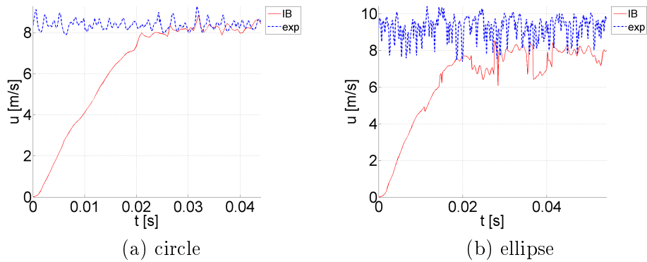
Figure 6.16: Measured (exp) and simulated (IB) velocity signal as a function of time immediately downstream from the constriction ( Z/L_c = 1.04 ) for P_0 = 35 Pa: a) circular constriction and b) elliptical constriction.
