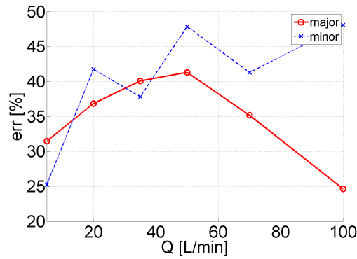
Figure 5.28: Illustration of the overall error (5.5) between modeled and experimental transverse velocity profiles along the ‘major’ and ‘minor’ axis of the rectangular cross section for different volume flow rates Q .
