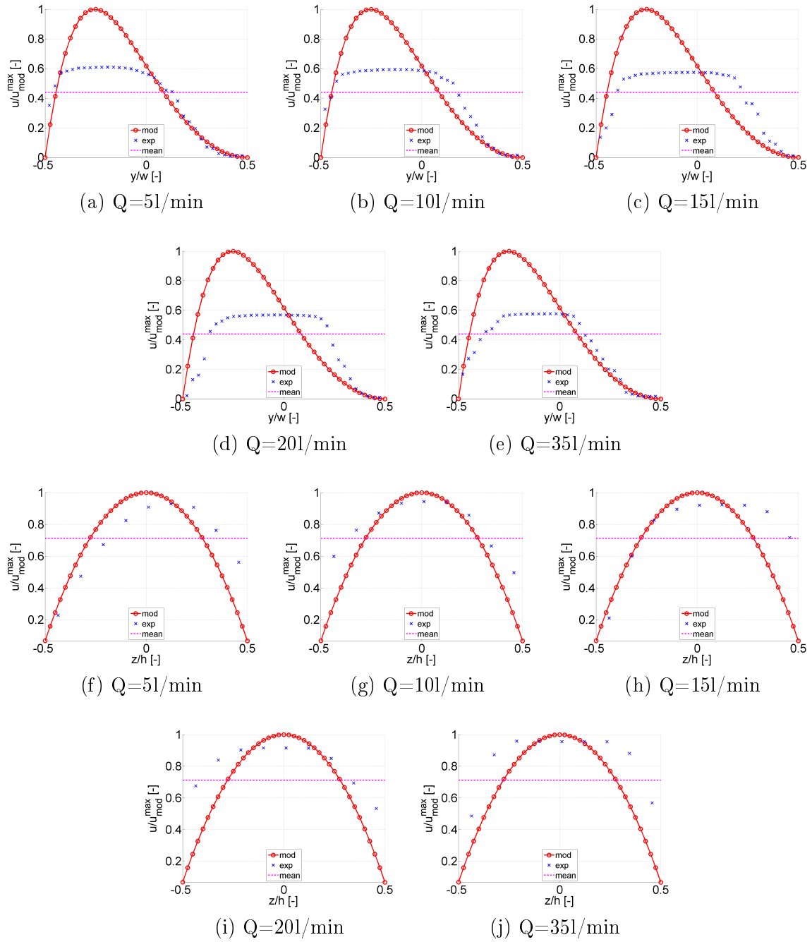
Figure F.13: Comparison of modeled and experimental assessed velocities normalized by the maximum modeled velocity u_{mod}^{max} at the exit of constriction for: (a-e) major axis and (f-j) minor axis of small circular sector. Volume flow rate are assessed for 5, 10, 15, 20 and 35l/min. Velocity estimated from transverse profiles using spatial step \Delta y = 0.5\text{mm} is labeled "exp". The modeled results is denoted as "mod" and \bar{u} is the bulk velocity. The width and height of the constricted portion along major and minor axis is labeled 'w' and 'h'.
