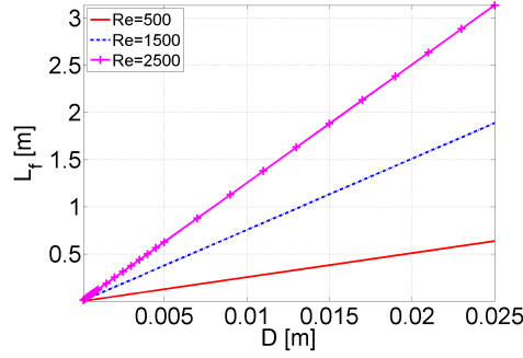
Figure 2.2: Illustration of the relationship between entry length L_f and hydraulic diameter D for different Reynolds numbers. The hydraulic diameter range and the Reynolds number range is relevant for the aimed biological flow applications mentioned in Fig. 1.5.
