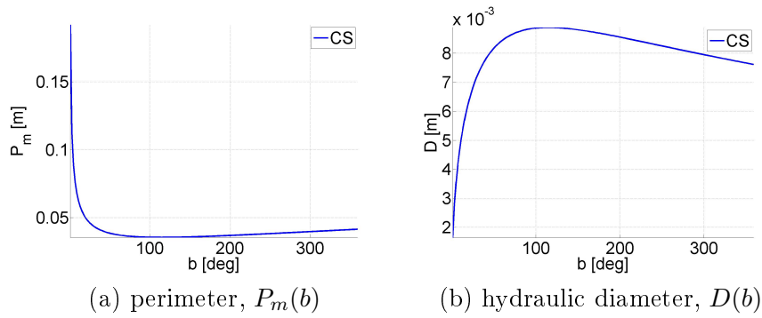
Figure 2.5: Circular sector (cs) of fixed area and varying angle b : a) perimeter P_m(b) and b) hydraulic diameter D(b) .
