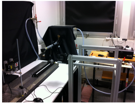
Figure 5.5: Illustration of the experimental setup used for flow visualization.
