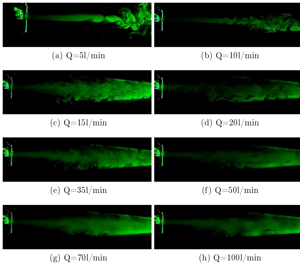
Figure F.20: Visualization of the flow profiles along the centerline of major axis of circular shape at a distance from 0cm to 21cm of the exit. Volume flow rate equal to 5, 10, 15, 20, 35, 50, 70 and 100l/min are experimentally assessed.
