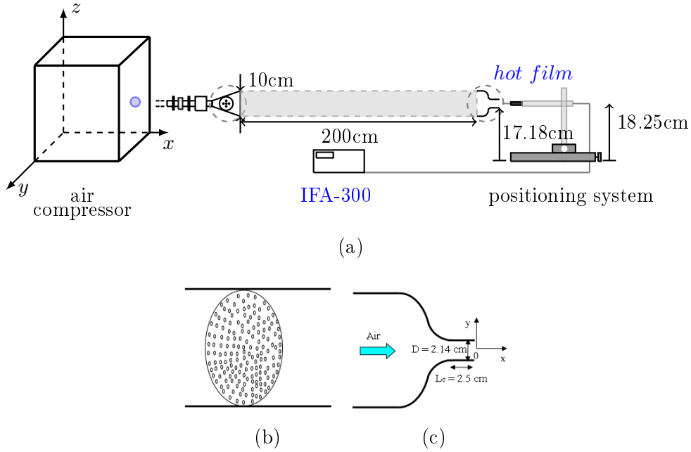
Figure E.5: a) Overview the setup of calibration for hot film. b) cross sectional view of the tube arranged in the diverging portion. c) cross sectional view of the converging tube.
