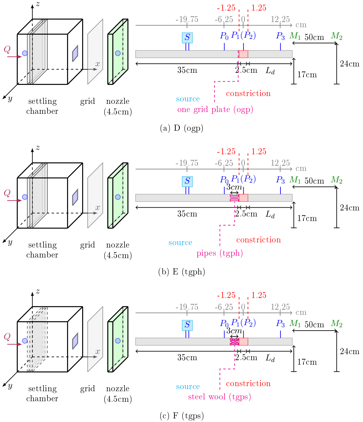
Figure 5.10: Schematic overview of assessed configurations for all cross section shapes shown in Fig. 5.1 for the values of L_u = 35 cm, L_d and with the used of a mixing element for the configurations labeled D, E and F listed in Table 5.4: without downstream pipe ( L_d = 0 cm) or with downstream pipe ( L_d = 15 cm).
