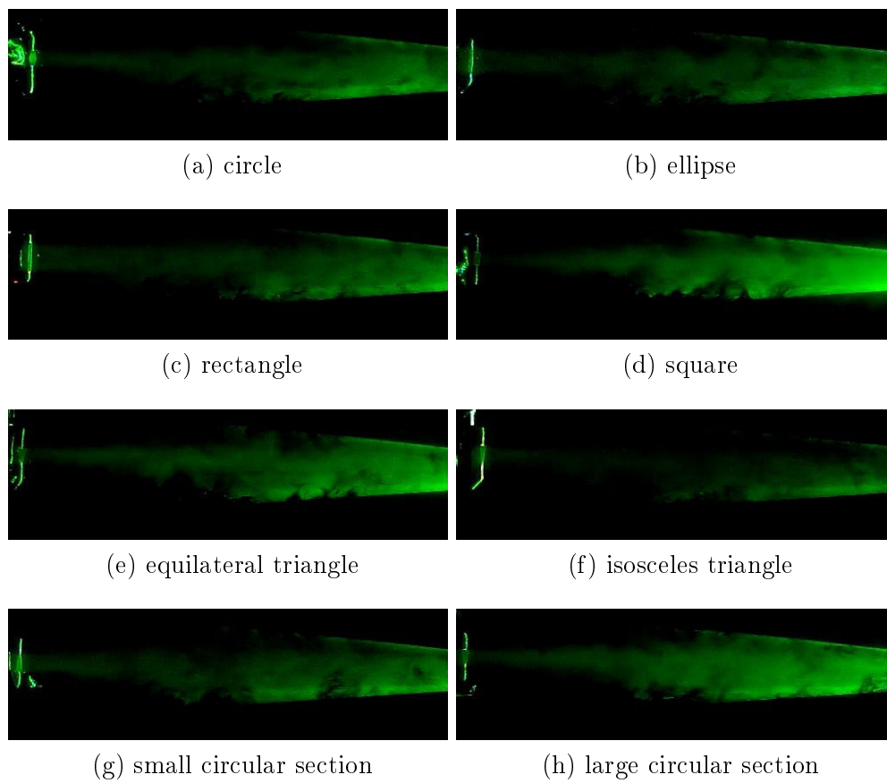
Figure F.16: Illustration of the visualization at major axis for all cross section shapes when volume flow rate equal to 50l/min.
