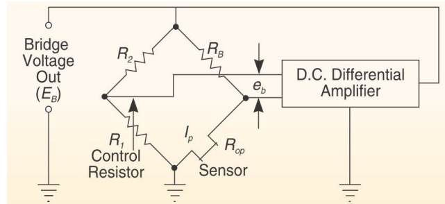
Figure E.4: Schema of constant temperature anemometer, where E_B : bridge voltage output, e_b : small voltage change at amplifier input, I_P : current through sensor, R_{op} : resistance of sensor at operating temperature, R_1 , R_2 , R_B : bridge resistor ( http://www.tsi.com/uploadedFiles/Product_Information/Literature/Catalogs/Hotwire_Catalog_2980465.pdf ).
