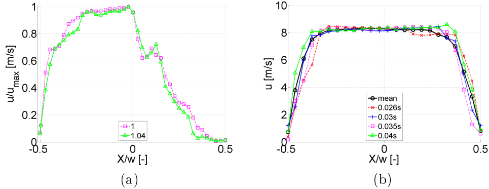
Figure 6.14: (a) Simulated transverse velocity profile along the X direction ( t = 50 ms) at the constriction outlet ( Z/L_c = 1 ) and downstream from the constriction ( Z/L_c = 1.04 ) for a constriction with circular section shape. (b) Several instantaneous ( t = 26 ms, t = 30 ms, t = 35 ms and t = 40 ms) and mean transverse velocity profiles immediately downstream ( Z/L_c = 1.04 ) from a circular constriction are shown. The mean value is obtained for t \geq 20 ms. The X coordinate is normalized by the the width of the constricted portion w along the X dimension.
