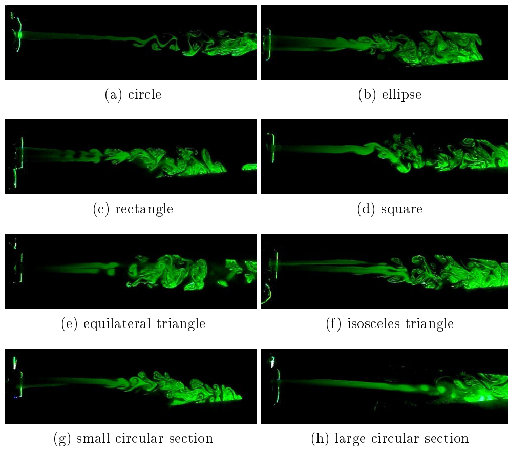
Figure F.17: Illustration of the visualization of centerline flow profile at major axis for all cross section shapes with one grid plate placed at the inlet of the constricted portion when volume flow rate equal to 5l/min.
