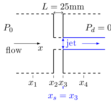
Figure G.1: Flow through an abrupt expansion.
