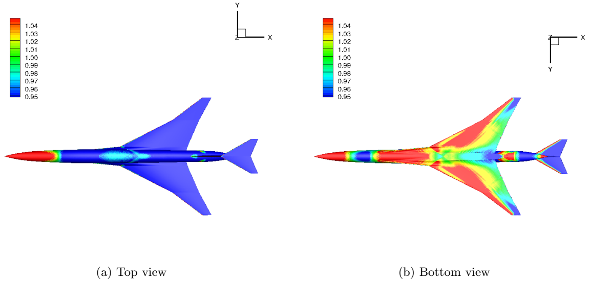
Figure B.4: Skin Pressure ( p/p_\infty ). Reference configuration.
