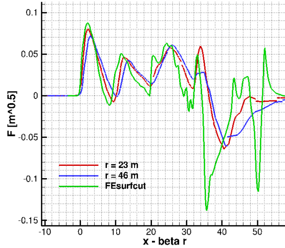
Figure B.10: Comparison of F-function obtained from pressure signal and FEsurcut.
