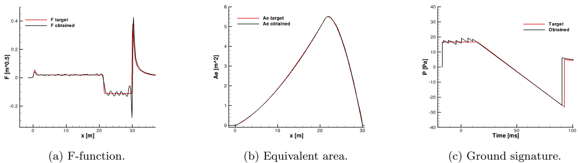
Figure 4.21: Wing-body configuration obtained after fuselage tailoring.
