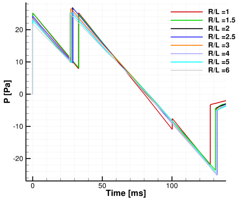
Figure 3.33: Ground signature obtained from the pressure field extracted at different distances from the source. The grid adopted is the one obtained after 20 adaptation iterations.
