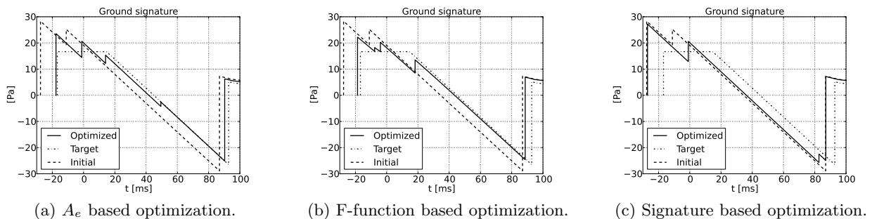
Figure 4.14: Ground signature obtained with the different objectives - Parametrization B: 27 design variables.
