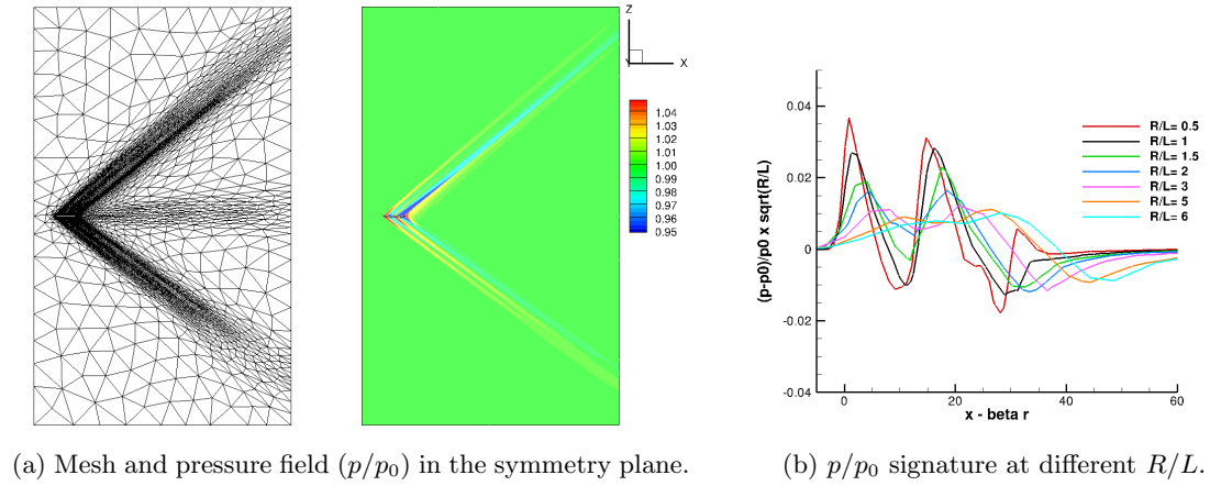
Figure 3.23: 5th adaptation at complexity \mathcal{C} = 20,000 .
