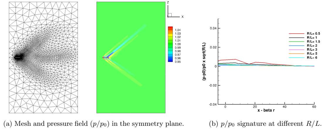
Figure 3.22: 1st adaptation at complexity \mathcal{C} = 20,000 .
