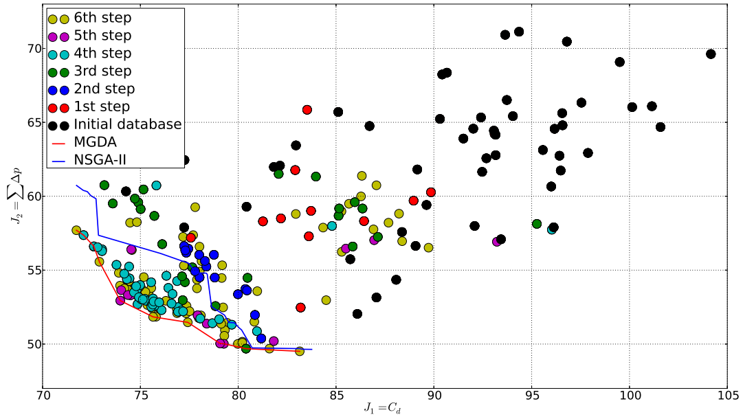
Figure 6.18: Convergence history of MA-MGDA. The comparison with NSGA-II is made at an identical number of high-fidelity function evaluation calls. (Data plotted are results from CFD analysis)
