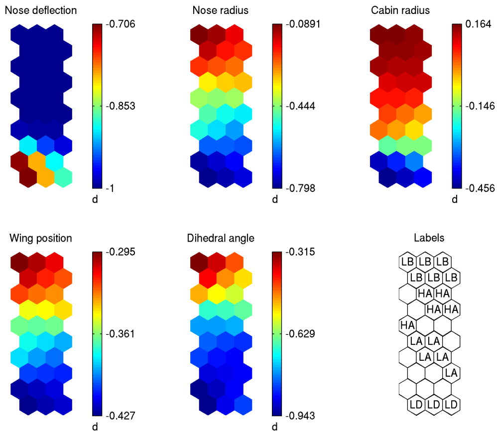
Figure 6.30: Variables SOM.
