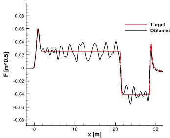
(a) F-function.
