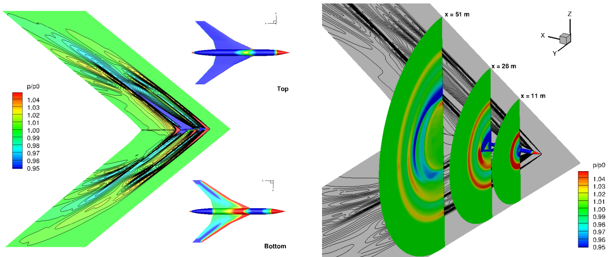
Figure 3.7: Near field pressure p/p_0 .
