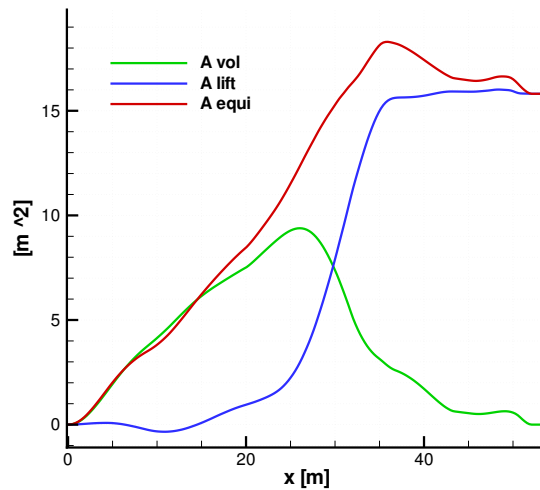
Figure B.6: Equivalent area. Reference configuration.
