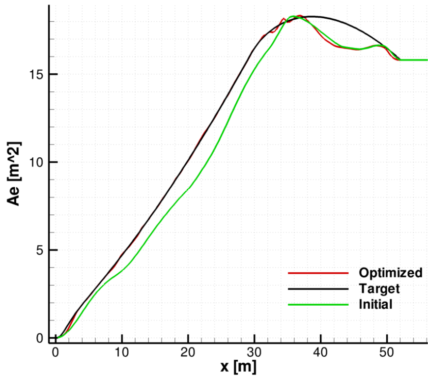
Figure B.24: Comparison of the obtained equivalent area distribution.
