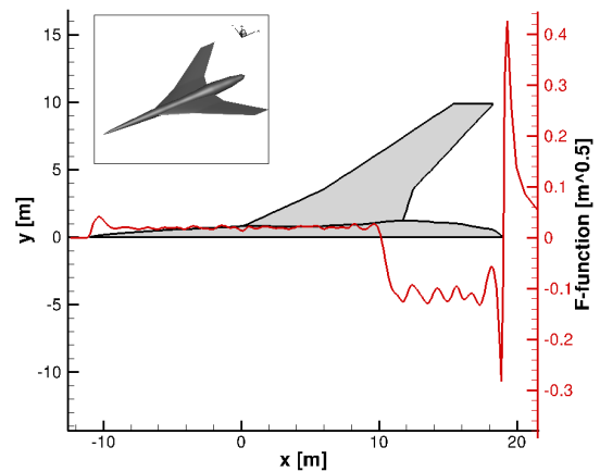
(b) Shaped configuration. Geometry and corresponding F-function.
