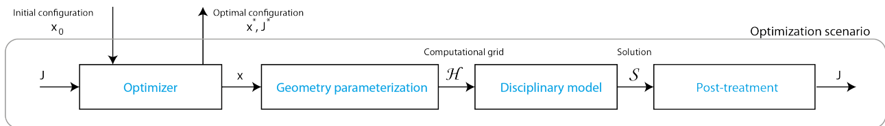
Figure 5.1: Generic shape optimization scenario.
