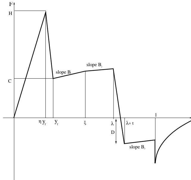
Figure 4.4: Rallabhandi F-function parameterization.
