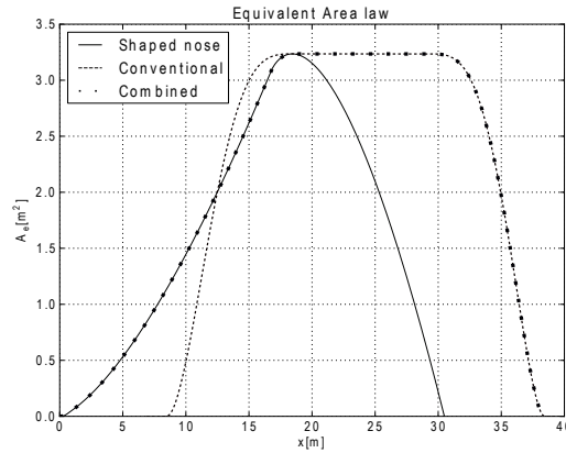
Figure 5.23: Equivalent area for a conventional fuselage with a shaped nose.
