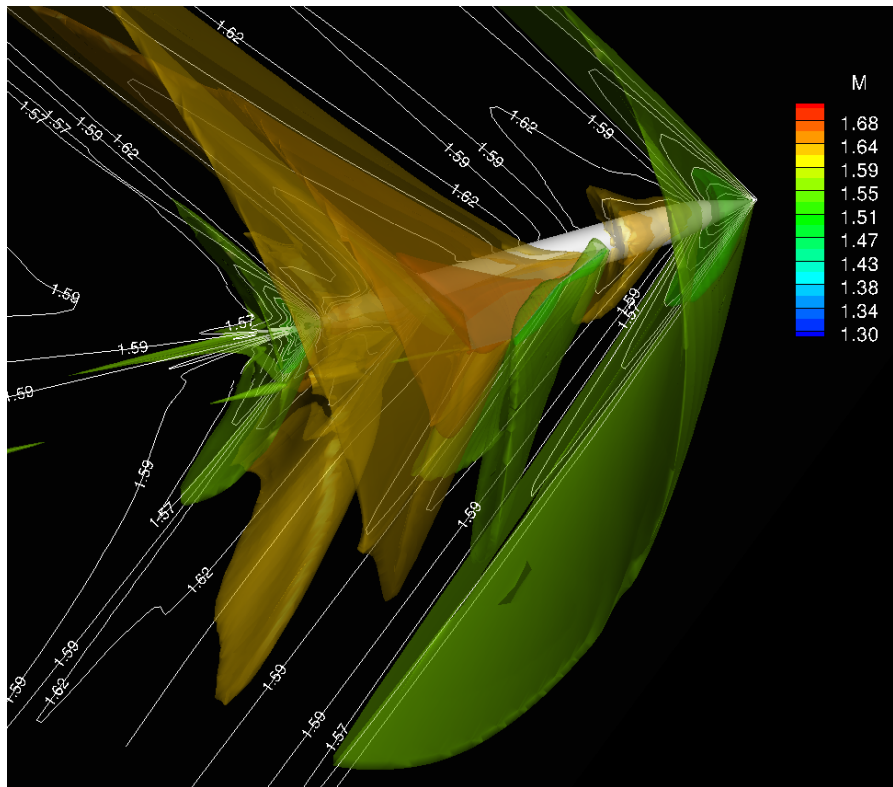
Figure 3.8: Mach iso-surfaces.
