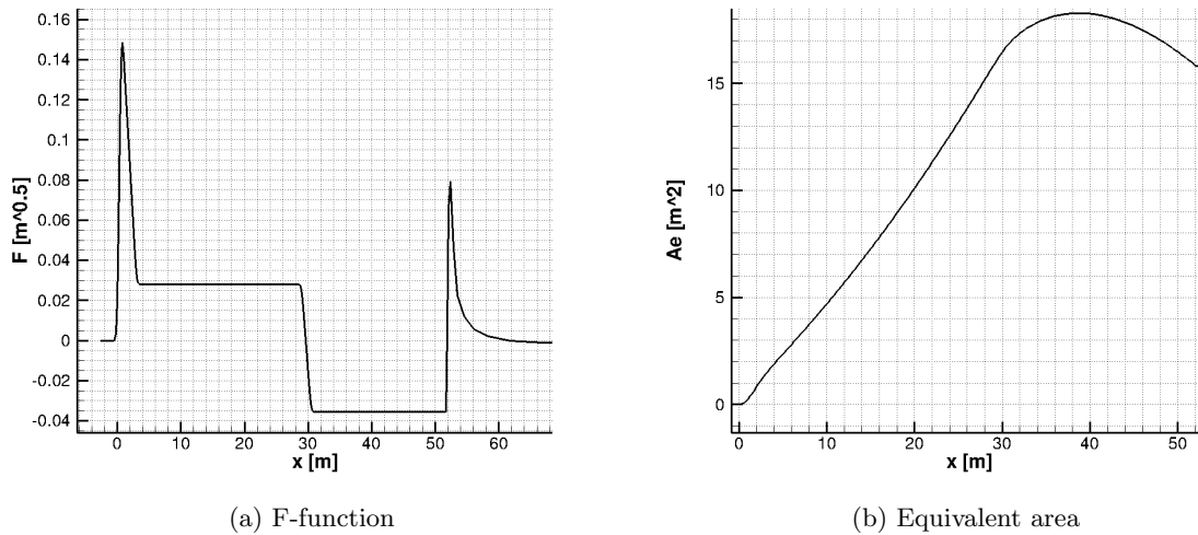
Figure B.22: Shaped design for Free-Form deformation.
