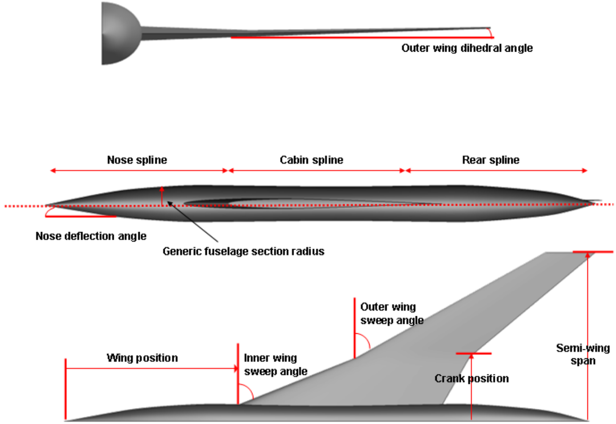
Figure 5.2: Generic shape parameterization adopted for the optimization problems.
