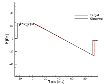
(c) Ground signature.
