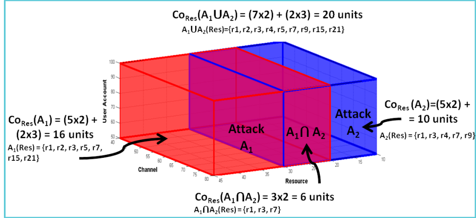
FIGURE 7.4 - Resource-based volume union and intersection
