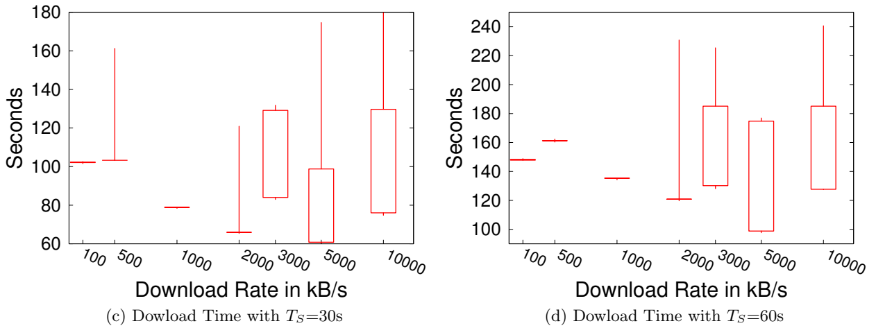
Figure 3.5: Upper-layer’s Reactivity
