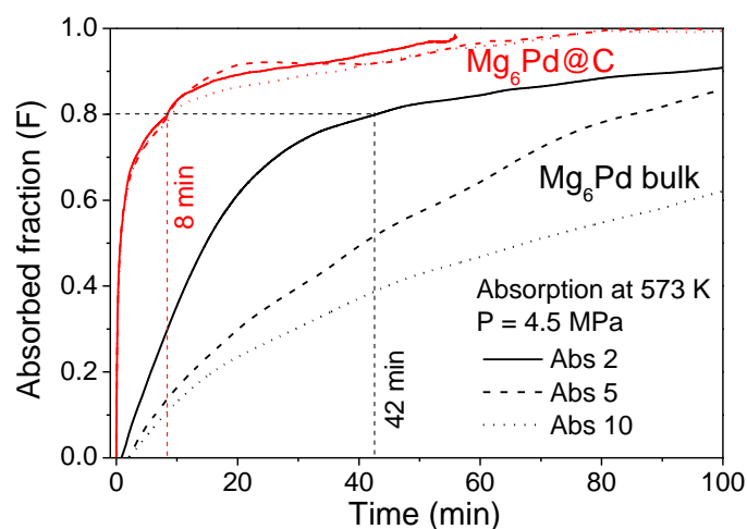
Figure 4.11. Time-evolution of the transformed fraction during H-absorption at 573 K in bulk and nanoconfined Mg_6Pd . Absorption curves during cycles 2, 5 and 10 are represented as solid, dash and dot lines, respectively.
