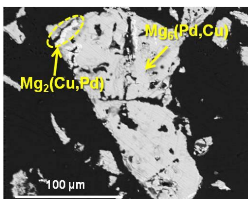
Figure 3.33. BSE image of the \text{Mg}_6\text{Pd}_{0.7}\text{Cu}_{0.3} compound after desorption.
