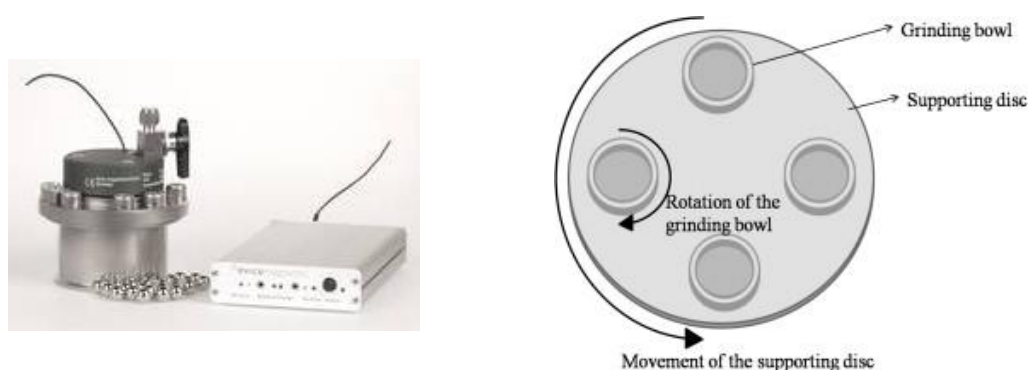
Figure 2.3. The Evicomagnetics milling vial and the telemetric receptor (left). Schematic representation of the principle of a planetary mill (right).
