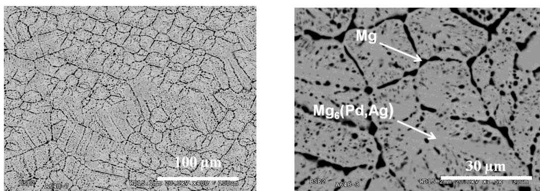
Figure 3.8. BSE images of an ingot slice of the Mg_6Pd_{0.5}Ag_{0.5} alloy.
