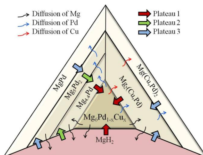
Figure 3.32. Schematic illustration of the phase growth during hydrogenation of the \text{Mg}_6\text{Pd}_{1-x}\text{Cu}_x compound. Large arrows represent the growing direction of the phases. Thin arrows symbolize the diffusion of each element.
