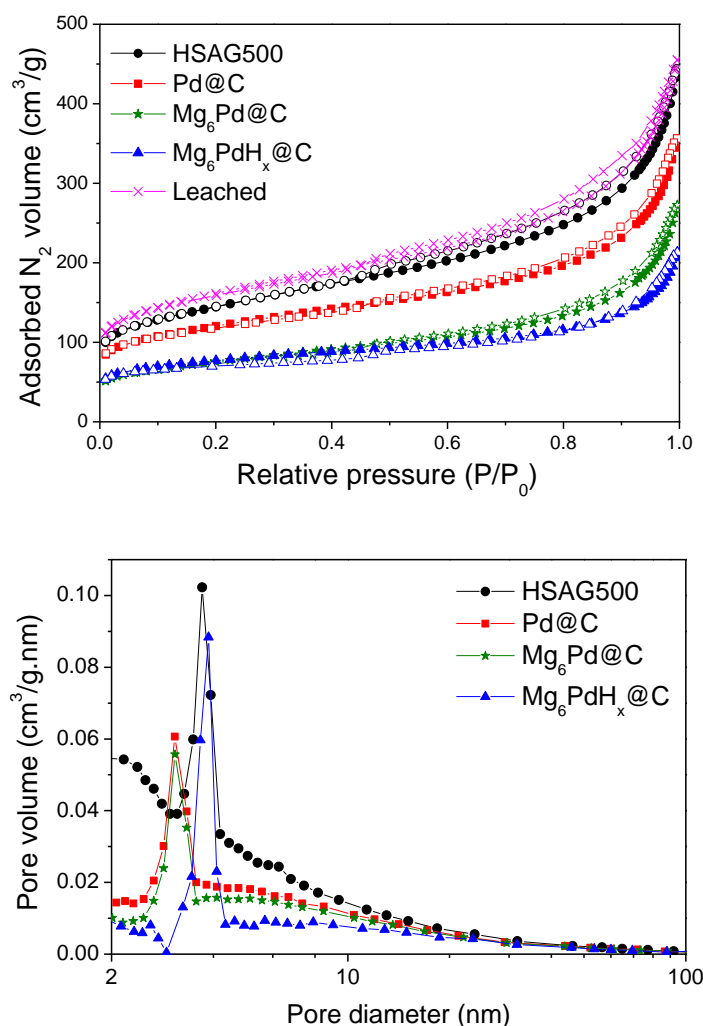
Figure 4.5. Nitrogen physisorption isotherms (top) and pore size distribution (bottom) of pristine HSAG500, after Pd impregnation (Pd@C), after infiltration of Mg (Mg 6 Pd@C), after hydrogenation (Mg 6 PdH x @C) and after removal of all metal species (leached). Full symbols correspond to adsorption and empty symbols to desorption.
