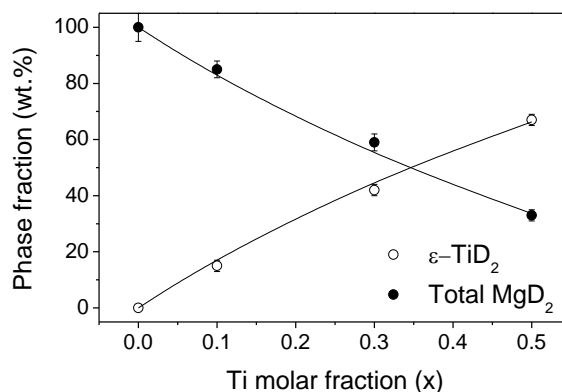
Figure 5.6. Refined phase content (TiD 2 and (\beta+\gamma) -MgD 2 ) in the as-milled (1-x)\text{MgD}_2-x\text{TiD}_2 samples. Continuous lines display the theoretical phase content for a MgD 2 -TiD 2 composite assuming no solubility of Mg in TiD 2 nor Ti in MgD 2 phases.
