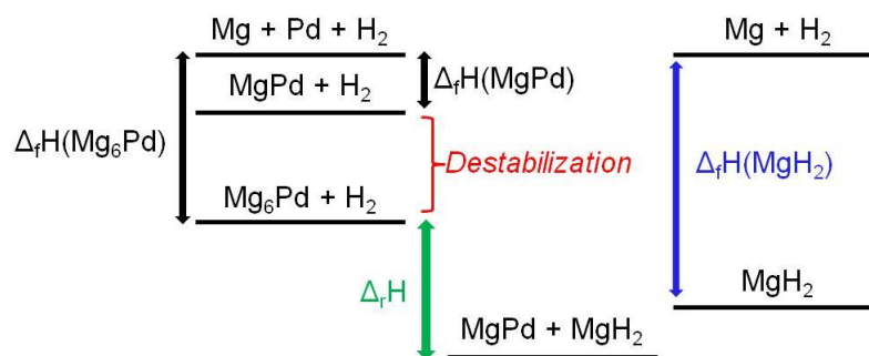
Figure 6.1. Schematic representation of the thermodynamic states during hydrogenation of the Mg 6 Pd compound. \Delta_r H is the enthalpy change corresponding to the global hydriding reaction ( \text{Mg}_6\text{Pd} + 5 \text{H}_2 \leftrightarrow 5 \text{MgH}_2 + \text{MgPd} ). \Delta_r H is smaller than \Delta_r H(\text{MgH}_2) because Mg 6 Pd is more stable than MgPd.
