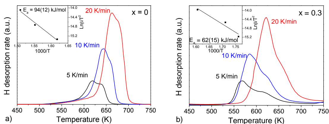
Figure 5.11. TDS spectra of RBM a) MgH 2 and b) 0.7MgH 2 -0.3TiH 2 samples obtained during heating at different rates (5, 10 and 20 K/min). The insets display the Kissinger plots used to determine the activation energies of desorption.
