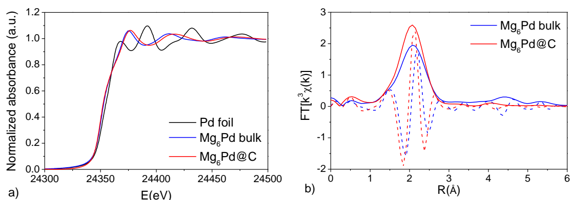
Figure 4.8. a) XANES spectra near Pd-edge of bulk and nanoconfined Mg 6 Pd compared to the Pd metal signal. b) Fourier transform of the EXAFS function \chi(k) ( k^3 -weighted calculated on 2.8-11.5 \text{\AA}^{-1} domain) of bulk and nanoconfined Mg 6 Pd. Continuous and dashed lines correspond to modulus and imaginary part, respectively.
