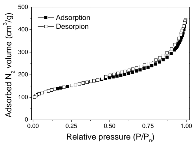
Figure 4.3. Nitrogen physisorption isotherm of pristine HSAG500.
