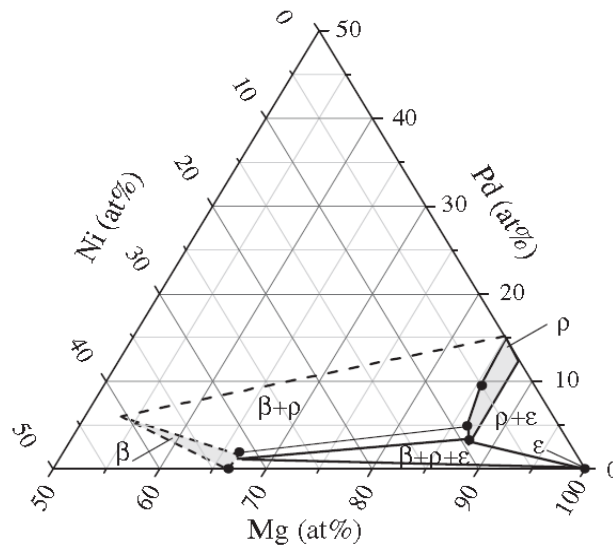
Figure 1.9. Ternary phase diagram of the Mg-Ni-Pd system in the Mg-rich corner at 673 K [84]. Labels: \rho for \text{Mg}_6\text{Pd} phase; \beta for \text{Mg}_2\text{Ni} phase; \epsilon for Mg phase.
