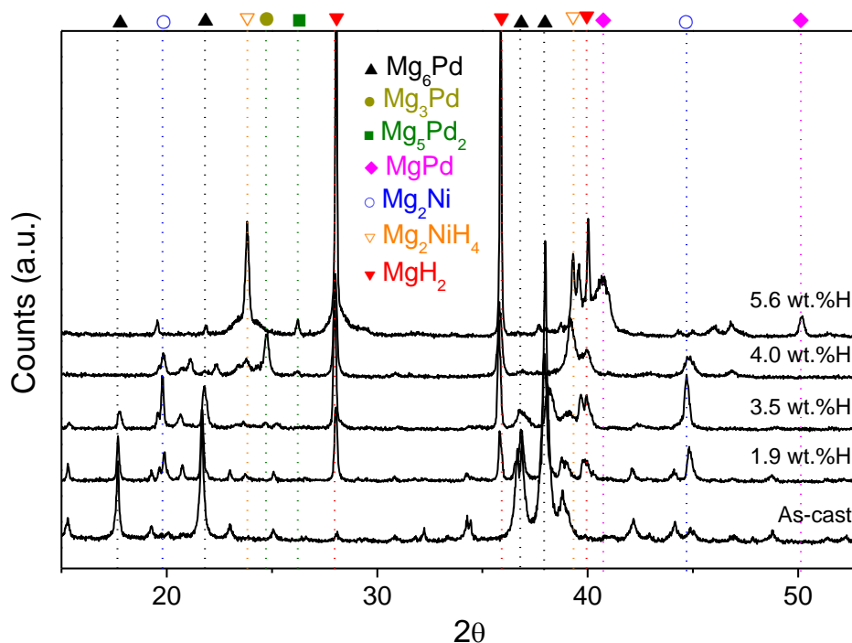
Figure 3.40. XRPD patterns (Cu K_\alpha radiation) of the \text{Mg}_6\text{Pd}_{0.25}\text{Ni}_{0.75} compound at different H-contents during absorption. Phase identification of main diffraction peaks is expressly indicated.
