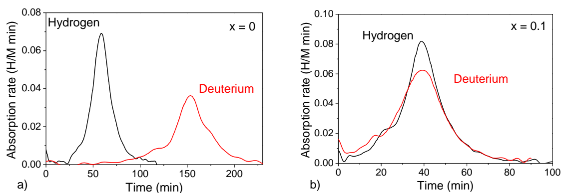
Figure 5.3. Time-derivative plots of the absorption curves obtained during RBM under hydrogen (black line) and deuterium gas (red line) for a) pure Mg and b) 0.9Mg-0.1Ti mixture.
