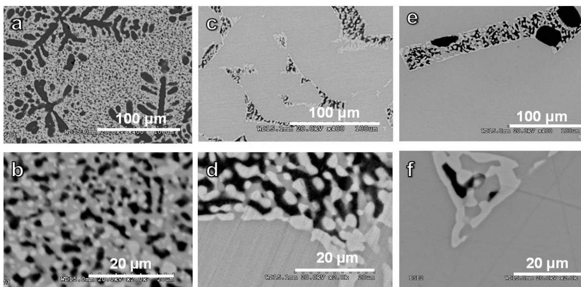
Figure 3.23. BSE images of Mg_6Pd_{1-x}Cu_x compounds with x = 0.5 (a and b), x = 0.3 (c and d) and x = 0.2 (e and f). Top and bottom images show different magnification views.
