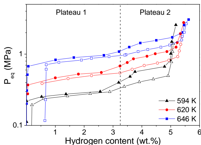
Figure 3.38. PCI curves of the Mg_6Pd_{0.25}Ni_{0.75} compound during absorption (full symbols) and desorption (empty symbols) at 594, 620 and 646 K.
