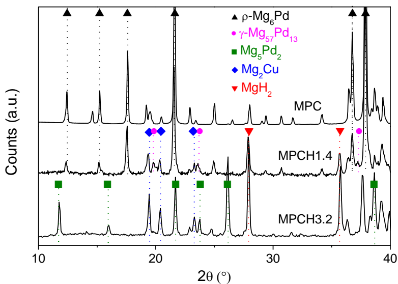
Figure 3.30. XRPD patterns (Cu K_\alpha radiation) of the \text{Mg}_6\text{Pd}_{0.7}\text{Cu}_{0.3} alloy before hydrogenation and hydrided to 1.4 wt.% H and 3.2 wt.% H.
