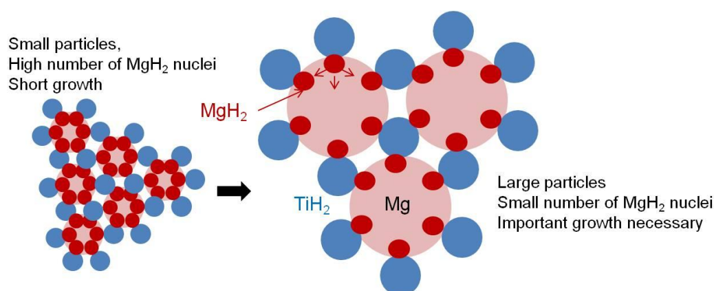
Figure 5.27. Illustration of the crystallite size effect on the absorption kinetics in MgH 2 -TiH 2 nanocomposites.
