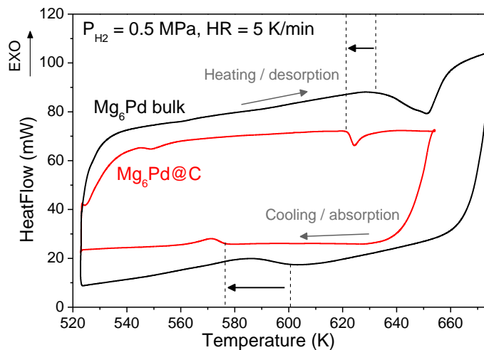
Figure 4.15. HP-DSC measurements obtained during heating and cooling ramps under 0.5 MPa of hydrogen pressure on bulk (black line) and nanoconfined (red line) Mg_6Pd .
