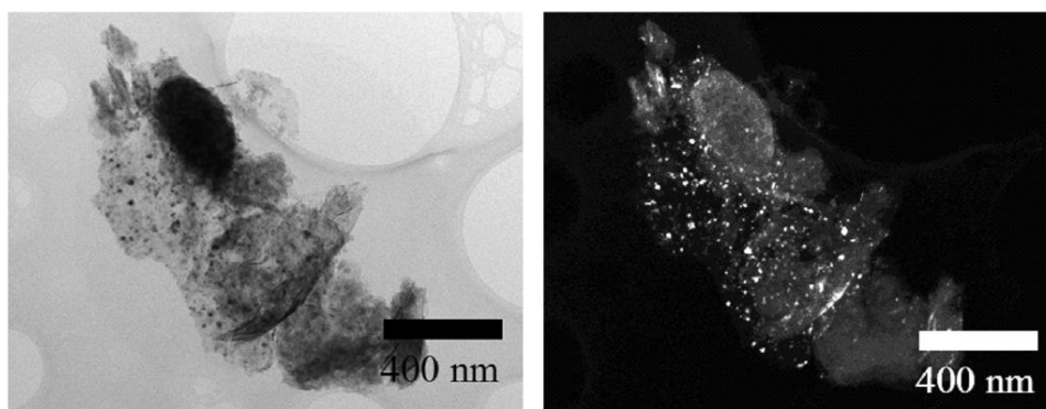
Figure 1.11. Bright field (left) and dark field (right) transmission electron micrographs of Mg_{0.87}Ni_{0.13} nanoparticles supported on a high surface area graphite [139].
