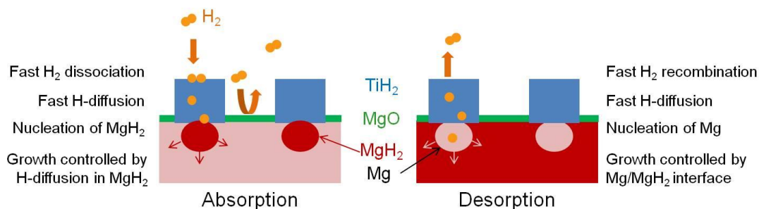
Figure 5.26. Schematic representation of hydrogen absorption and desorption mechanisms in MgH 2 -TiH 2 nanocomposites.
