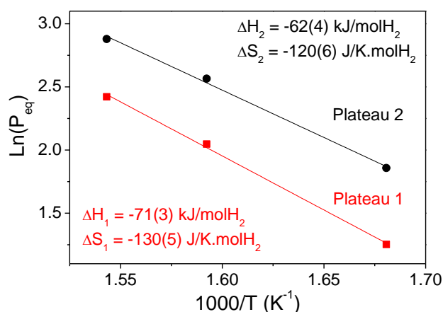
Figure 3.29. Van't Hoff plots corresponding to the two absorption plateaus of the Mg_6Pd_{0.7}Cu_{0.3} isotherms.
