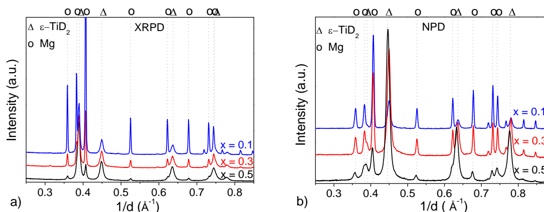
Figure 5.8. a) X-ray and b) neutron powder diffraction patterns of thermally desorbed (1-x)Mg-xTiD 2 nanocomposites for x = 0.1 , 0.3 and 0.5.
