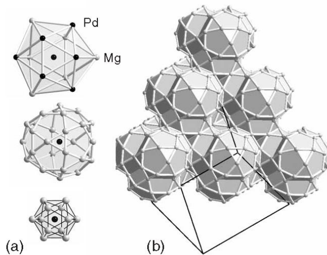
Figure 1.8. a) The three concentric shells of a Mackay cluster and b) arrangement of Mackay clusters in the Mg 6 Pd cell [72].
