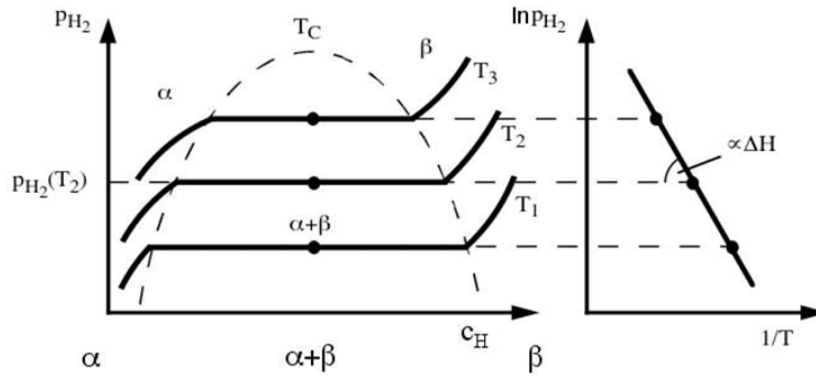
Figure 1.2. Schematic PCI diagram and corresponding Van't Hoff plot, taken from [23].
