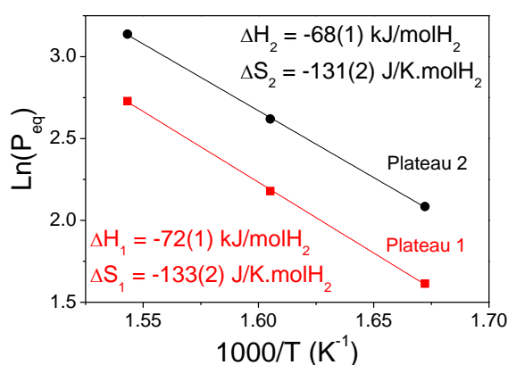
Figure 3.4. Van't Hoff plots corresponding to the two absorption plateaus of the Mg_6Pd isotherms.
