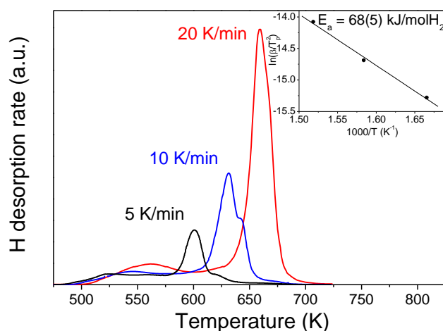
Figure 3.49. TDS spectra of the Mg 6 Pd 0.25 Ni 0.75 compound hydrided at 5.6 wt.% H measured at heating rates of 5, 10 and 20 K/min. The inset displays the Kissinger plot and corresponding activation energy.
