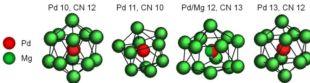
Figure 4.9. Representation of the first coordination sphere around each Pd site in the Mg 6 Pd structure.
