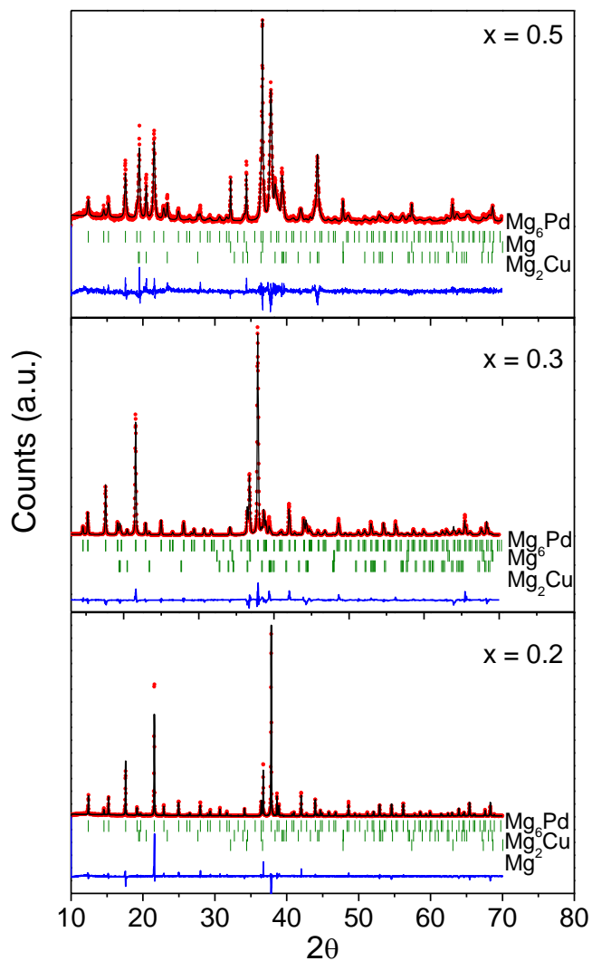
Figure 3.24. XRPD patterns (Cu K_\alpha radiation) of the \text{Mg}_6\text{Pd}_{1-x}\text{Cu}_x alloys for x = 0.5, 0.3 and 0.2 (dots) and the corresponding Rietveld refinement (solid line). Bragg peak positions are plotted as vertical bars. The line below represents the difference between the calculated and the experimental patterns.
