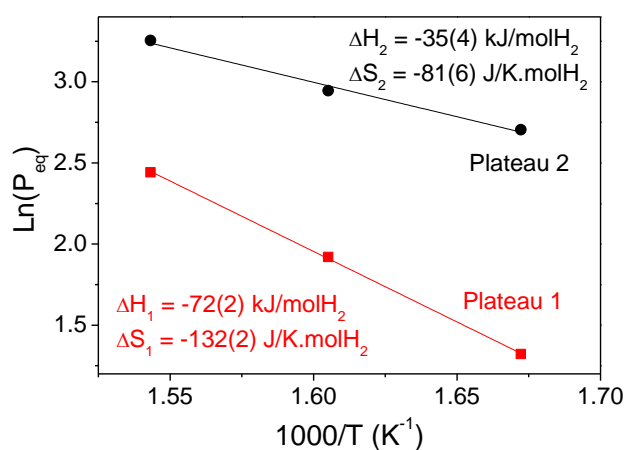
Figure 3.15. Van't Hoff plots corresponding to the two absorption plateaus of the Mg_6Pd_{0.5}Ag_{0.5} isotherms.
