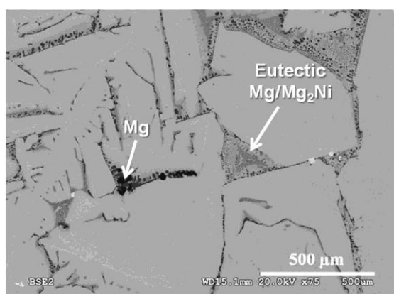
Figure 3.36. BSE image of an ingot slice of the Mg_6Pd_{0.25}Ni_{0.75} alloy.
