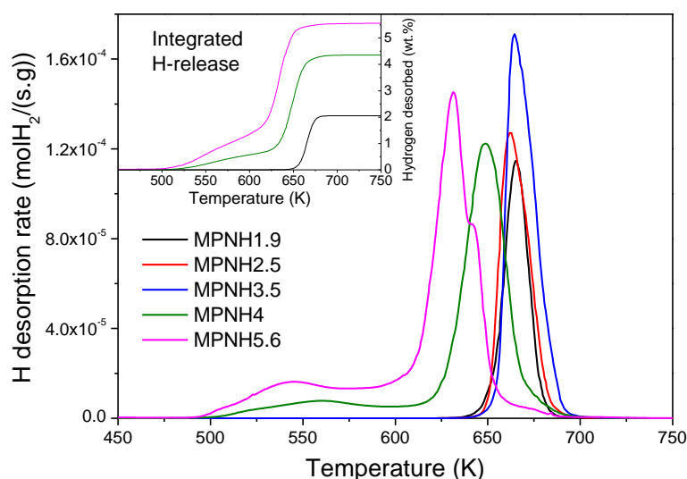
Figure 3.48. TDS spectra measured at 10 K/min for several partially hydrided Mg_6Pd_{0.25}Ni_{0.75} compounds. The inset represents the amount of hydrogen desorbed (wt.% H) as a function of the temperature.
