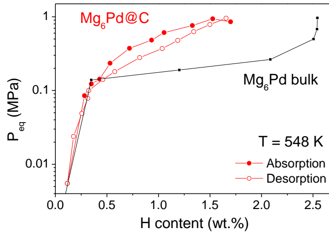
Figure 4.14. PCI curves at 548 K of the bulk (black line) and nanoconfined (red line) Mg_6Pd .
