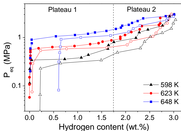
Figure 3.14. PCI curves of the Mg_6Pd_{0.5}Ag_{0.5} sample during absorption (full symbols) and desorption (empty symbols) at 598, 623 and 648 K.
