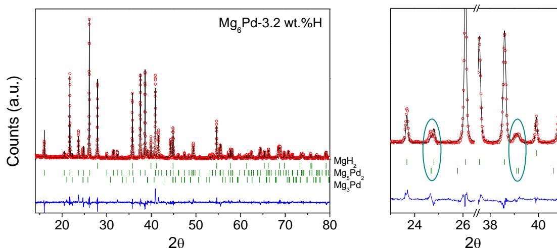
Figure 3.5. XRPD Rietveld refinement of the hydrided (3.2 wt.% H) Mg_6Pd compound (Cu K_\alpha radiation). The plot on the right shows a detailed view of the Mg_3Pd main peaks. Continuous line shows the calculated diffraction pattern and vertical bars correspond to the Bragg positions. The difference between experimental and calculated patterns is given below.
