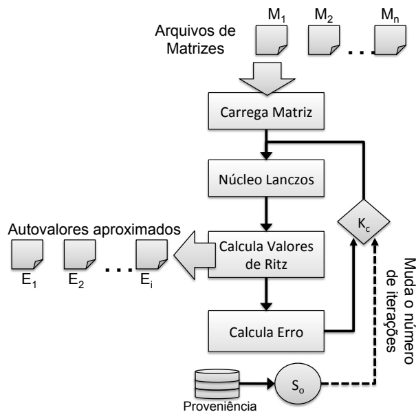
Figura 18. O Workflow Lanczos (Dias et al. 2011).
