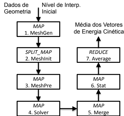
Figura 23. Workflow de QI manual
