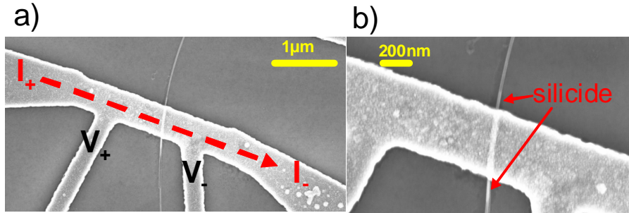
Figure 3.6: a) SEM micrograph of a sample used for the temperature estimation of the stripline. The potential drop V^+ - V^- falling between the inner probes is measured while a current flows through the constriction under a constant voltage bias. The stripline contacts a nanowire sitting between the voltage probes. b) Close up view of the contacted nanowire. The red arrows shows the silicides formed after Joule heating.
