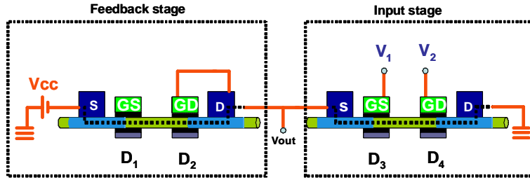
Figure 2.18: Schematics of the circuit. V_1 and V_2 represent the input voltages. D1, D2, D3, D4 correspond to the interfaces between the Nickel silicide and the silicon and are represented as Schottky diodes. The gate voltage controlling D1 is kept at a fixed value V_{GS} = -3V . The alimantation voltage is V_{cc} = -1.5V
