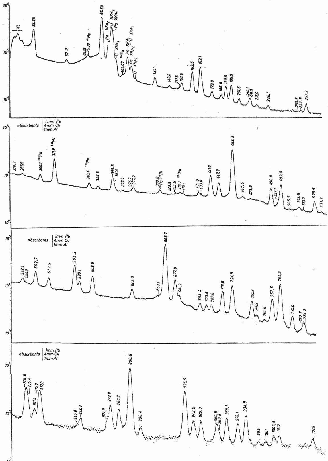
Fig. III.1 - 233 Th → 233 Pa - Spectre γ.
