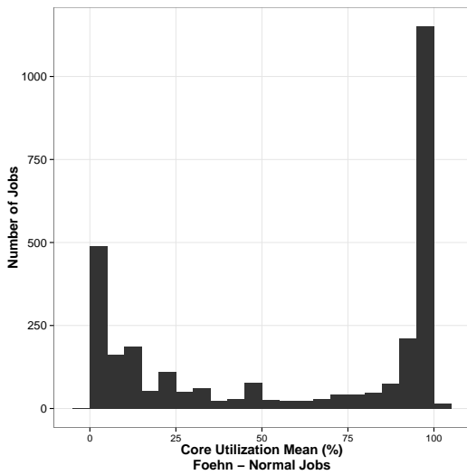
Figure 3.1: Distribution of the jobs' core utilization means.
