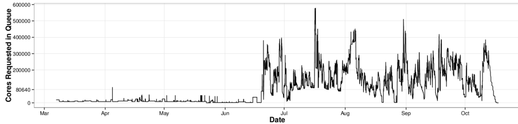
(b) Queue Size (total cores requested) of the SWF Trace on Curie.
