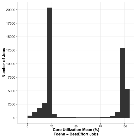
Figure 3.5: Distribution of the jobs' core utilization means.
