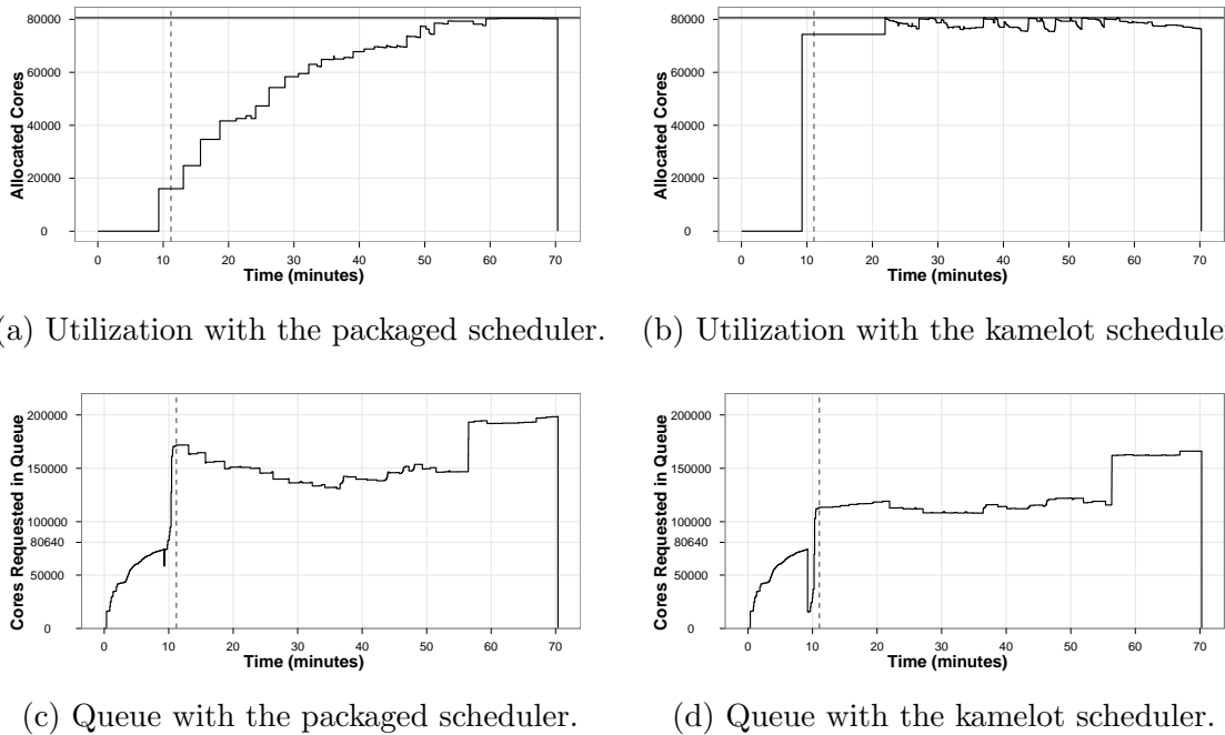
Figure 3.5: OAR utilization and queue size for the 2 schedulers replaying the Curie selected trace.
