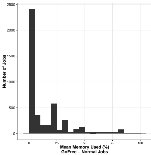
Figure 3.10: Distribution of the mean memory used by job.
