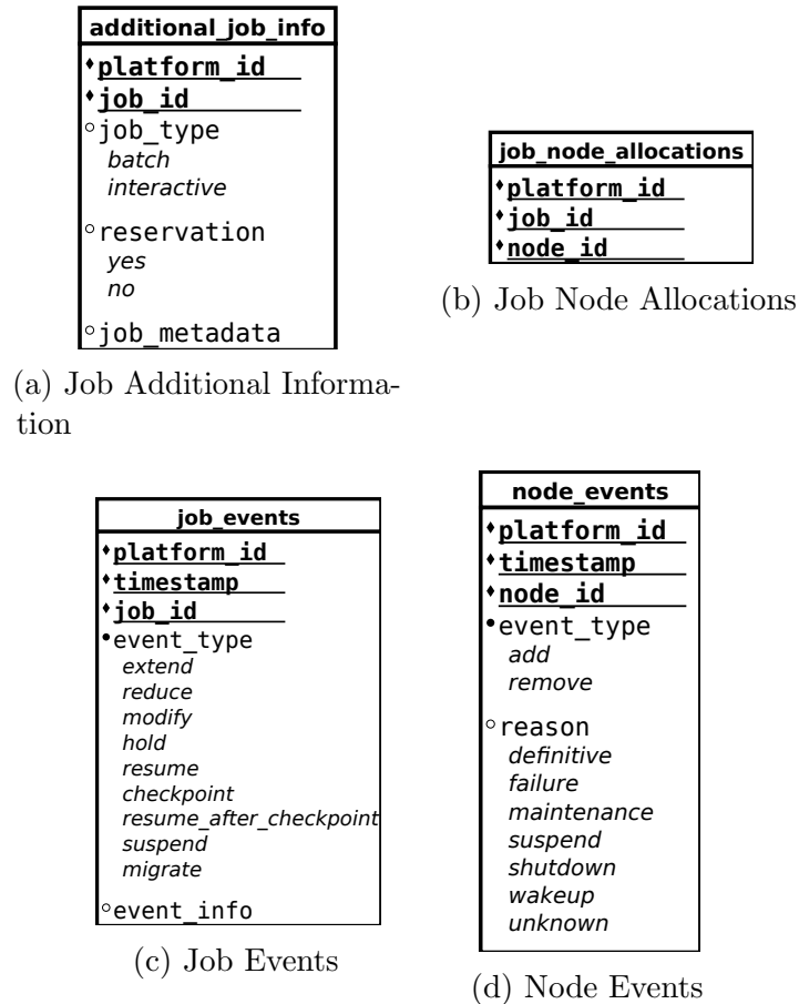
Figure 4.4: SWF Extensions
