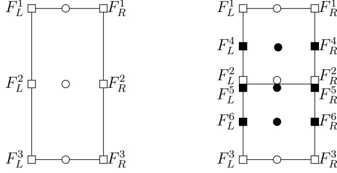
Figure 3.13: Example of a splitting procedure to save the computational cost associated to the degree of freedom already computed. On the left the cell at level of resolution k is reported while on the right the corresponding split cells are reported with the new points to explicitly add (black symbols).
