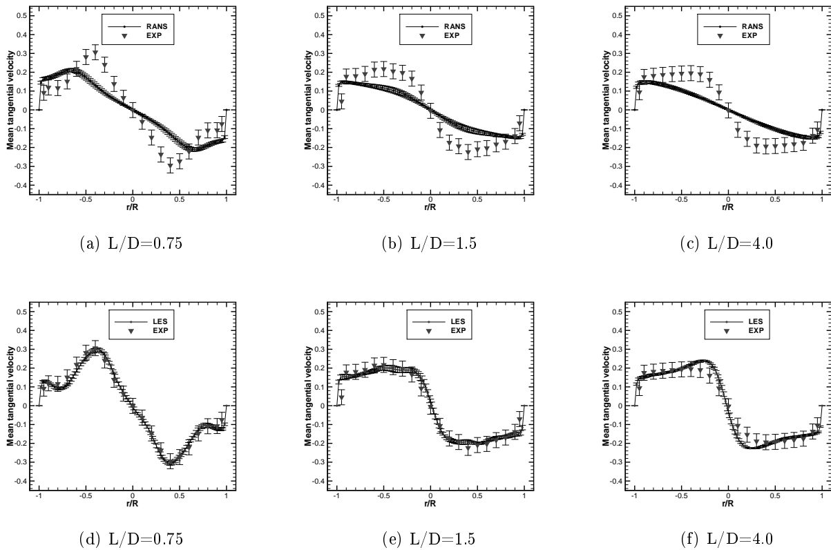
Figure 4.11: High-swirl flow. Statistics of the tangential velocity distributions (mean value and standard deviation displayed as error bar) at successive sections (from left to right : upstream to downstream) computed with RANS modeling / PC(3) (top : a,b,c) and LES modeling / PC(2) (bottom : d,e,f). Numerical results are compared with experimental measurements (mean value and assumed experimental error bar).
