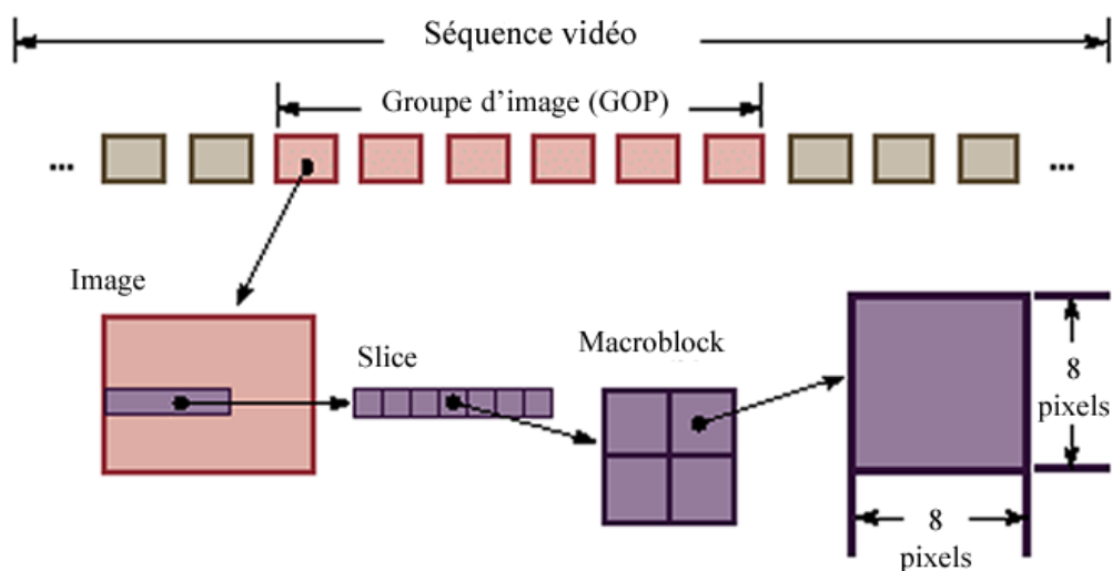
Figure 2.2. Syntaxe MPEG
