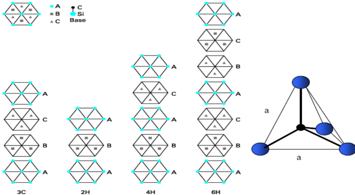
Figure 5 : Structure : Si-C.
