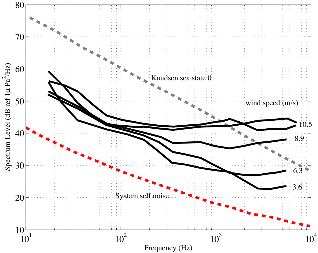
Figure 3.3: Spectra of wind noise under shore-fast ice for several wind speeds (source: [Milne67]).
